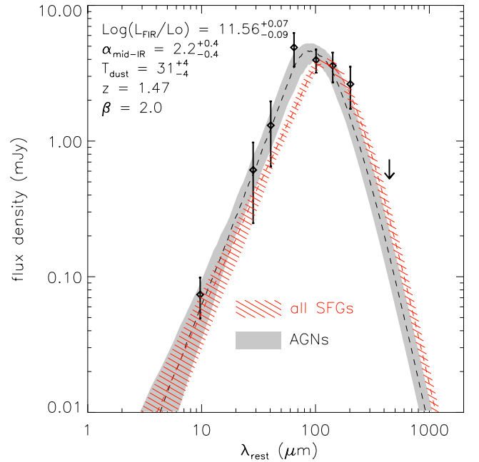
Figure 3. Stacked SED for all possible AGN (grey shaded region), including radio-loud, X-ray-detected and mid-IR identified ones (see Section 2.1 for details). The derived far-IR properties for the AGN sample are inset at the top-left. The stacked AGN SED is compared to the one obtained from all HiZELS star-forming galaxies (red line filled; presented in Fig. 2, right).
