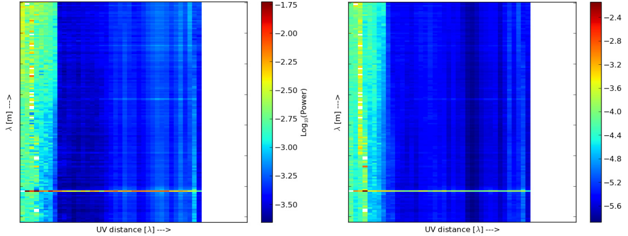
Fig. 7. Distribution of the power ( left panel ) and its error ( right panel ) as a function of the UV-distance (up to 10 \text{ k}\lambda ) and frequency, detected by CS stations only. The row showing a systematic excess of power over the entire UV-distance range corresponds to the corrupted and discarded SB 233.
