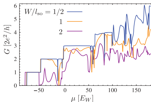
FIG. 4. (Color online) Conductance of a disordered NS junction, calculated numerically from the model Hamiltonian (21). The chemical potential \mu is increased at constant V_Z = 90 E_W , \Delta_0 = 8E_W (blue dashed line in the BDI phase diagram of Fig. 3), for three different values of the spin-orbit coupling length l_{\text{so}} . Each curve is for a single disorder realization (of strength U_0 = 180 E_W ). The conductance quantization at 2, 3, 4 \times 2e^2/h is lost by chiral symmetry breaking as W becomes larger than l_{\text{so}} .
