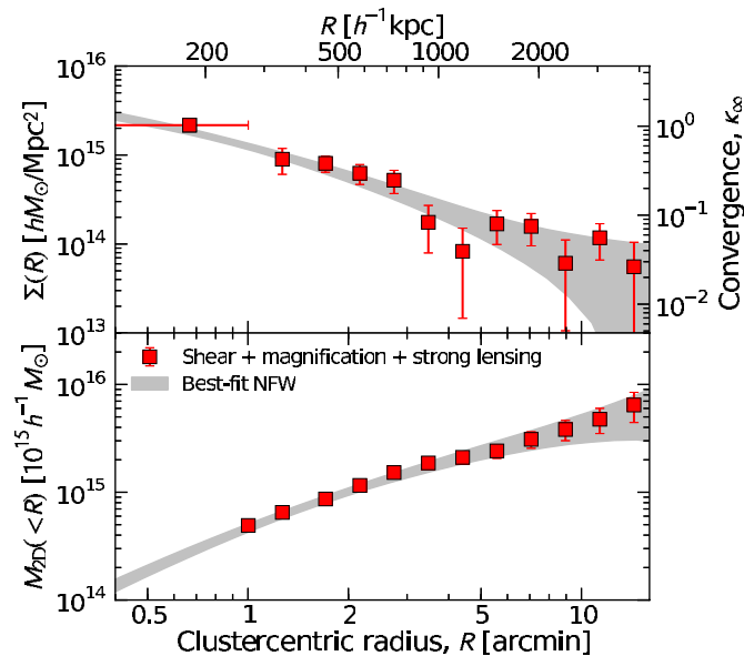
Figure 9. Top: surface mass density profile \Sigma(R) (squares) derived from a joint SL, WL distortion and magnification (WL+SL) likelihood analysis of our HST + Subaru lensing observations. The gray area represents the best-fit NFW profile for the mass profile solution \Sigma(R) . Bottom: the cumulative mass M_{2D}(<R) (red squares) as derived from the full lensing analysis. The gray area is the NFW fit ( 1\sigma confidence interval) to the WL+SL constraints as described above.
