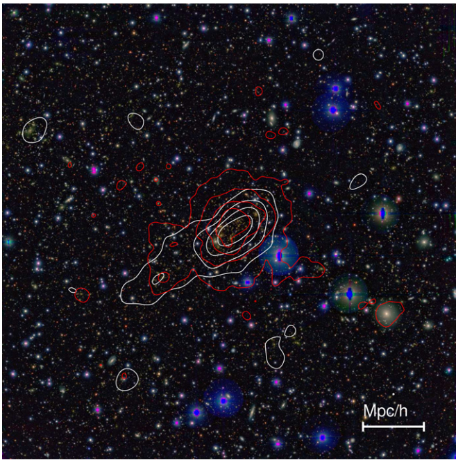
Figure 1. 28' \times 28' CFHT u^* + \text{Subaru } BVRCi'z' composite color image showing the galaxy cluster MACSJ0717 ( z = 0.548 ). Overlaid are the surface mass density map reconstructed from our Subaru WL analysis (white contours) and the X-ray brightness map from XMM-Newton observations (red contours). North is up and east is to the left.
