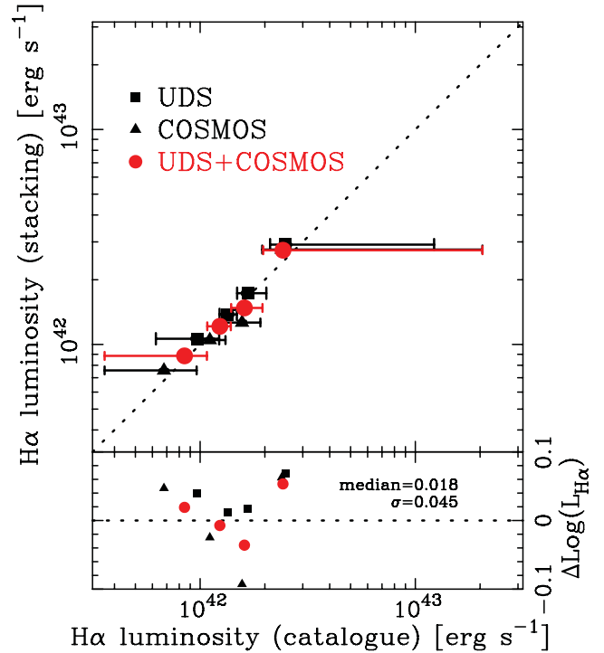
Figure 4. Comparison between H\alpha luminosities measured on the stacked ( \text{NB}_H - H ) image and median values of H\alpha luminosities extracted from the catalogues, for H\alpha emitters which are individually detected as galaxies with (H - \text{NB}_H) colour excess. We plot both the individual fields and our combined sample. The median and standard deviation of \Delta \log L_{H\alpha} , the difference between both H\alpha luminosities, are 0.018 and 0.045, implying good agreement between the two H\alpha luminosities, which confirms the validity of our stacking analysis procedure.
