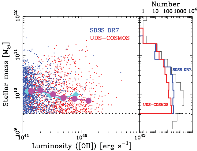
Figure 3. The left-hand panel shows stellar mass as a function of [O II] luminosity. The red dots show [O II] emitters at z = 1.47 in the combined sample and the blue dots show galaxies in the SDSS sample with similar median mass distribution to that of [O II] emitters at z = 1.47 . The magenta circles and cyan diamonds show the median stellar mass of galaxies in each [O II] luminosity bin for the samples of [O II] emitters and SDSS galaxies, respectively. The right-hand panel shows the mass distribution of each samples: the black thin histogram shows the whole sample of SDSS galaxies with \log(L_{[\text{O II}]}/\text{erg s}^{-1}) > 41 and \text{EW}_0 > 10 \text{ \AA} at z \sim 0.1 , the blue thick histogram shows those of local galaxies extracted from the SDSS sample and the red thick histogram shows the mass distribution of [O II] emitters at z = 1.47 in the combined sample including the UDS and COSMOS fields.
