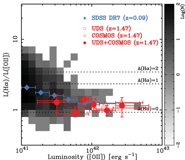
Figure 7. Same as Fig. 5, but the ratio of H\alpha to [O\text{ II}] as a function of [O\text{ II}] luminosity. The flux ratios are corrected by 3 per cent for the bias caused by the difference of profile of the two narrow-band filters (Section 2.2) and by 15 per cent for the possible contamination to be included in the sample (Section 3.1). The dotted lines show the ratio of H\alpha to [O\text{ II}] in the case of each dust attenuation in H\alpha which is derived from the best-fitting polynomial function shown in Fig. 6.
