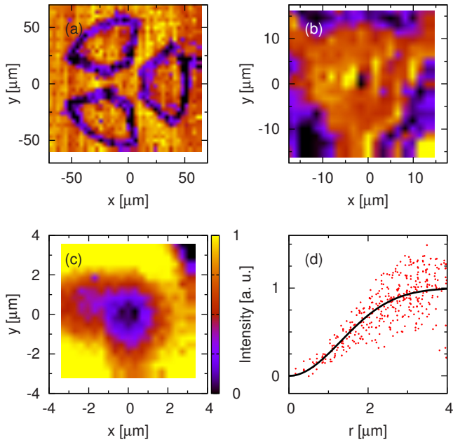
FIG. 2. (Color online) [(a)–(c)] Resonant reflection measurements at room temperature of a micropillar structure with 125 \mu\text{m} outer trench diameter with increasing resolution: (a) the full structure, (b) the micropillar itself, and (c) the aperture. (d) Radial plot of (c) and a Gaussian fit, yielding a cavity mode diameter at the surface of 4.0 \pm 1.5 \mu\text{m} .
