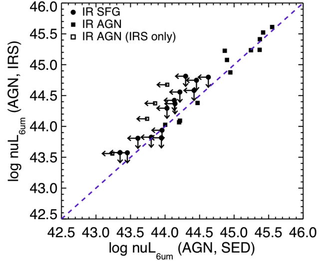
Fig. A.1. Comparison of the AGN 6\ \mu\text{m} luminosity obtained from the SED fitting of the photometric Spitzer and Herschel data points ( \nu L_{6\ \mu\text{m}} , SED) versus the L_{6\ \mu\text{m}} estimated from the IRS spectral (+ Herschel data points) fitting ( \nu L_{6\ \mu\text{m}} , IRS). For the IR SFGs, where the AGN component was not significantly detected, we plotted an upper limit of the AGN L_{6\ \mu\text{m}} (i.e., 30% of the total 6\ \mu\text{m} luminosity; see Appendix A). Sources where the classification from the two analyses agree are shown as filled symbols: IR AGN (filled squares) and IR SFG (filled circles). The AGN identified only from the IRS spectral fit are shown as open squares.
