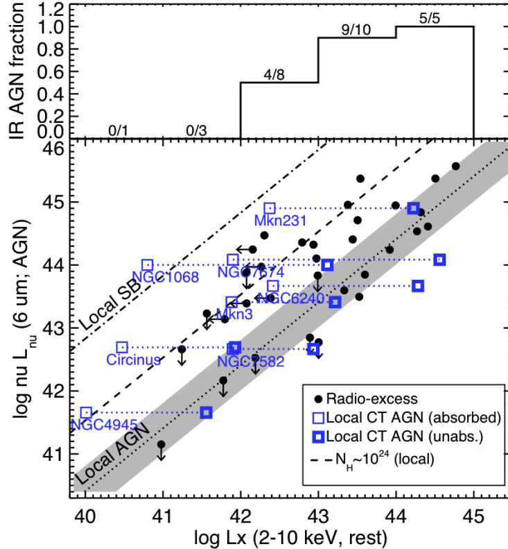
Fig. 9. Fraction of IR detected AGN as a function of the X-ray luminosity ( top panel ); the sources have been divided in five luminosity bins, between L_X = 10^{40} – 10^{45} erg s ^{-1} , although no AGN is expected to be found below L_X = 10^{41} erg s ^{-1} . The bottom panel shows the X-ray luminosity at 2–10 keV (rest-frame; not corrected for absorption) vs. the monochromatic 6 \mu m AGN luminosity ( \nu L_\nu ) for the radio-excess sources. Some local Compton-thick AGN are also plotted as open squares (thin marks: observed L_X ; thick marks: absorption corrected L_X ). The shaded region represents the typical L_{6\mu\text{m}} - L_X relation for local AGN (Lutz et al. 2004), while the dashed line is the relation expected for heavily obscured AGN ( N_H \approx 10^{24} cm ^{-2} ) and the dash-dotted line is the typical relation for starburst galaxies (taken from Alexander et al. 2008).
