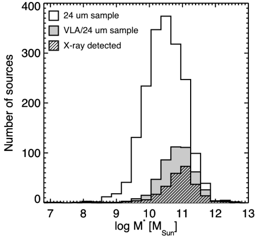
Fig. 1. Galaxy stellar masses in units of M_{\odot} for the entire 24\ \mu\text{m} detected sample with redshift identification (spectroscopic or photometric). The stellar masses for the sources detected in the VLA radio band are shown as grey histogram and the X-ray detected sources are shown as shaded black histogram.
