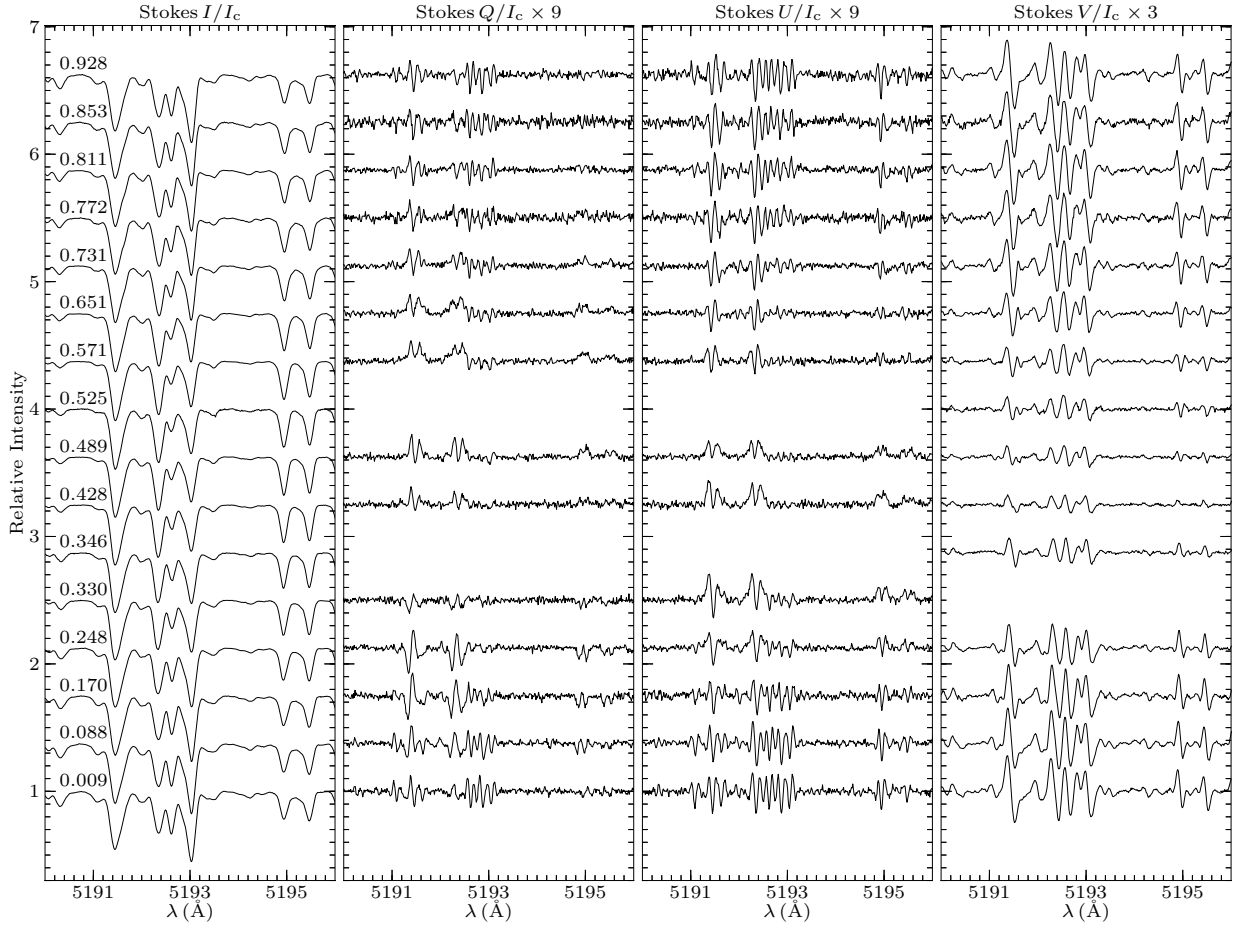
Fig. 3. Variations of Stokes IQUV profiles in the 5190–5196 \text{\AA} wavelength region. The four prominent features at 5191–5193 \text{\AA} are blends of Fe-peak and REE lines. The other two lines around 5195 \text{\AA} belong to Fe. This plot is characteristic of the complex polarization profiles observed in the spectra of HD 24712. The format of this figure is similar to Fig. 2.
