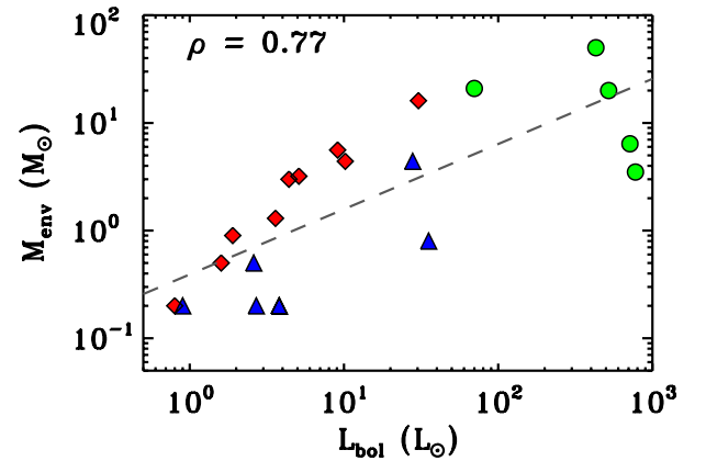
Fig. 11. Bolometric luminosity vs. envelope mass of the sources.
