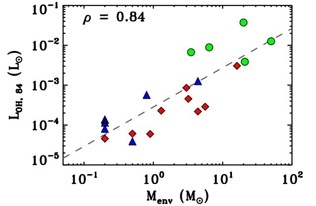
Fig. 10. OH 84 \mu\text{m} luminosity vs. envelope mass of the source.
