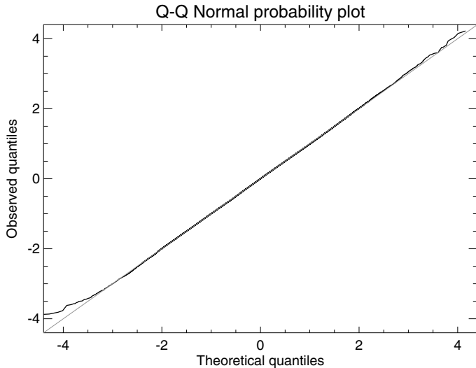
Fig. 9. Quantiles of a normal distribution versus the measured quantiles of Fig. 8. The grey line indicates a perfect normal distribution. The two agree well up till the 4\text{-}\sigma level, which is determined by the number of available sampling points.
