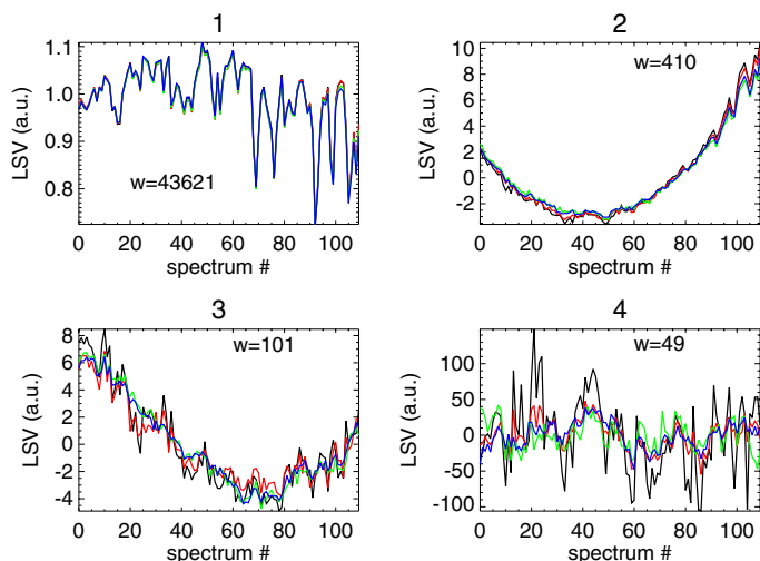
Fig. 2. First four left singular vectors for all four detectors (black – detector 1; red – detector 2; green – detector 3; blue – detector 4) at 2.3 \mu\text{m} on 13 July 2011, divided by their median value. The corresponding eigenvalues for detector 2 are also given to indicate their relative strengths. These vectors can be compared with the parameters in Fig. 4.
