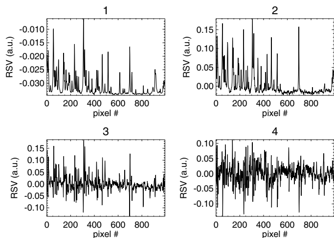
Fig. 3. First four right singular vectors, or eigenvectors, for detector 2 at 2.3 \mu\text{m} on 13 July 2011.
