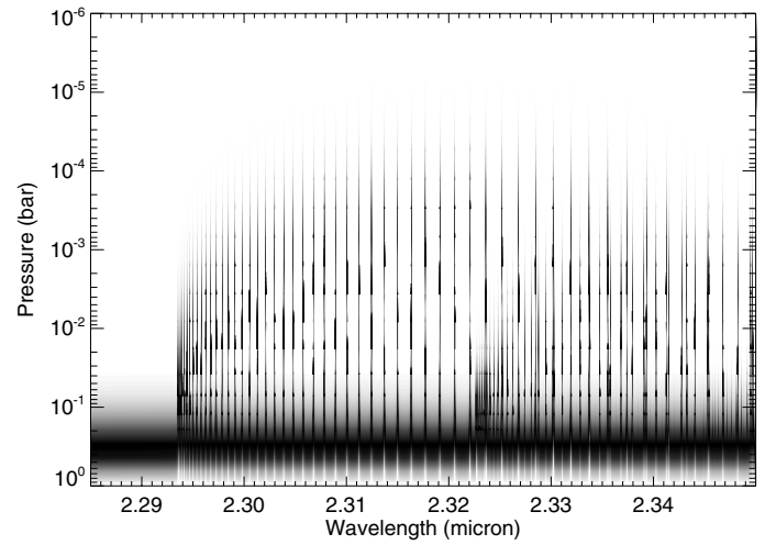
Fig. 12. Normalised contribution functions for a model spectrum with CO at a volume mixing ratio of 10^{-4} . These show where in the atmosphere the thermal flux is emitted for each wavelength.
