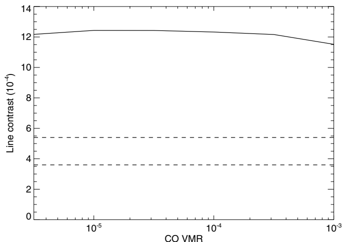
Fig. 13. The highest line contrasts (solid line) as a function of CO volume mixing ratio in our model grid (see Sect. 3). The lowest line contrast in a planetary atmosphere is zero for an isothermal atmosphere. Dashed lines show our determined limits on the CO line contrast.
