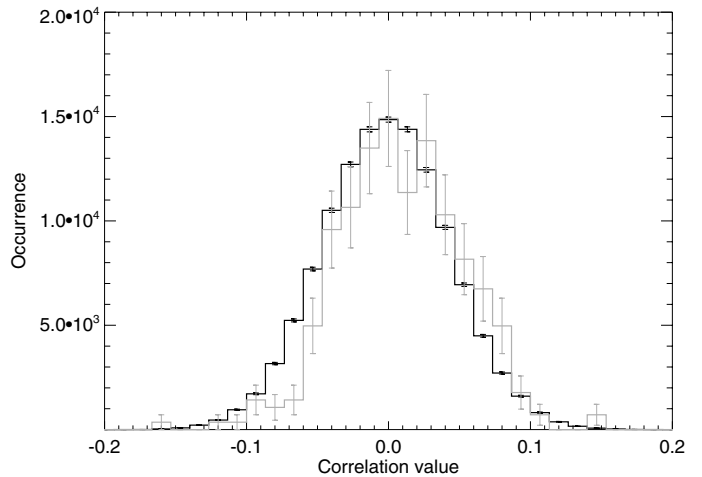
Fig. 10. Histogram of correlation values away from the expected planet velocity ( +10\text{--}400\text{ km s}^{-1} with respect to the planet), and those at the planet velocity (grey line, scaled), for detectors 2–4 combined.
