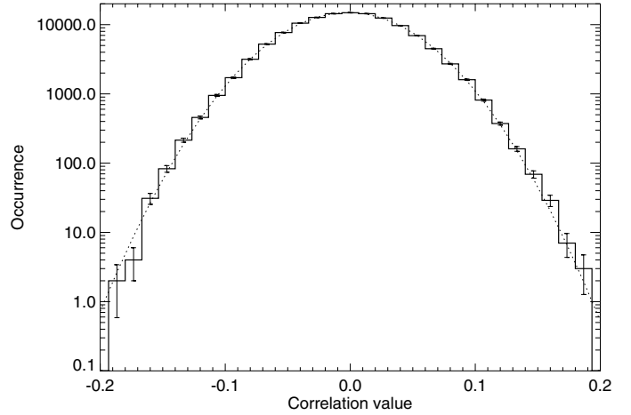
Fig. 8. Histogram of correlation values outside the expected planet velocity ( +10 – 400 \text{ km s}^{-1} with respect to the planet) for detectors 2–4 combined. Error bars are the square root of the number of occurrences in each bin. The dotted line shows a Gaussian fit.
