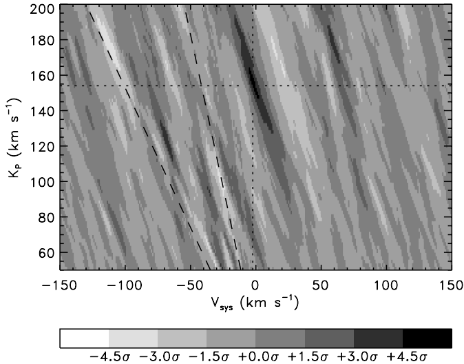
Fig. 6. Combined cross-correlation values for all four detectors as a function of system velocity and K_p . The dashed line indicates where the stellar CO lines are expected to leave the strongest contamination signal. The area in between the dashed lines can also be contaminated by stellar residuals. The dotted lines indicate the system velocity of HD 189733 and the peak position of K_p .
