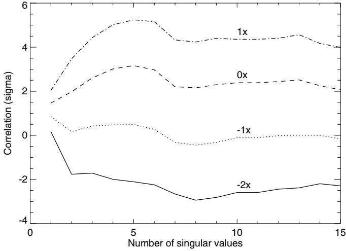
Fig. 5. Total correlation at the planet position as a function of the number of subtracted singular values for detector 2 at 2.3 \mu\text{m} on 13 July 2011 for the planet model giving the highest correlation. Different lines indicate different multiplication factors of the inserted planet signal (see text), as indicated by the labels.
