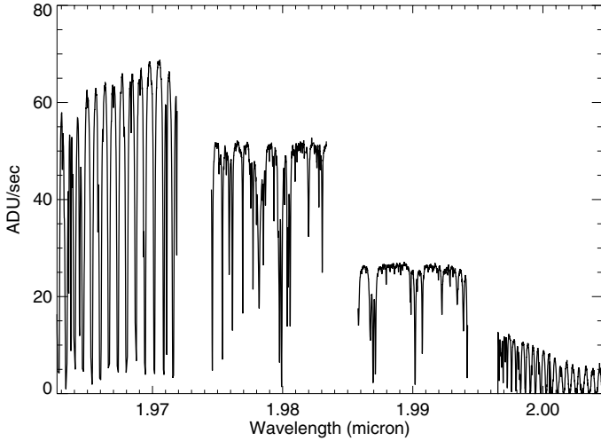
Fig. 11. Example spectrum of the data at 2.0 \mu\text{m} .
