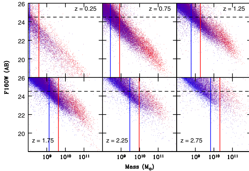
Figure 2. Observed H_{F160W} magnitude vs. stellar mass in six redshift bins. The color coding represents the rest-frame U - V colors, ranging from U - V = 0 (blue) to U - V = 2 (red). The horizontal dashed lines indicate the limit ( H_{F160W} = 24.5 ) down to which we can determine sizes with good fidelity. The vertical lines illustrate the resulting mass completeness limits for blue ( U - V = 0.5 ) and red ( U - V = 2.0 ) galaxies, respectively. See Section 2.4 for further details.
