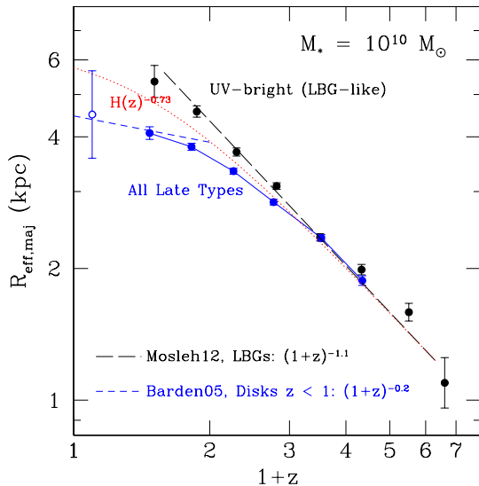
Figure 12. Size evolution of galaxies in a narrow (0.3 dex) mass bin around 10^{10} M_\odot . The black points represent UV-bright galaxies (with U - V < 1 in the rest-frame), selecting a sample akin to LBGs at high redshift. Their size evolution is fast, consistent with the size evolution of UV-selected samples up to z = 7 as recently determined by Mosleh et al. (2012)—also see Oesch et al. (2010). The blue points represent late-type galaxies as defined in this paper (see Figure 1), that is, all star-forming galaxies. The size evolution of those is slower at low redshift, consistent with previous measurements at z < 1 (here, Barden et al. 2005).
