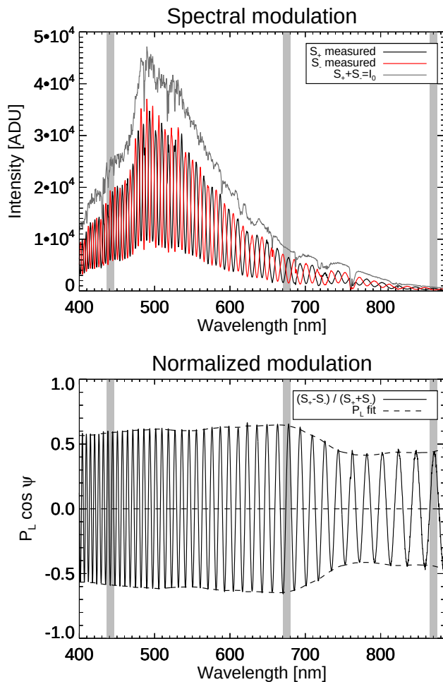
Figure 1. Top: the groundSPEX instrument measures the two perpendicularly modulated spectra S_+ and S_- simultaneously. The degree ( P_L ) and angle ( \phi_L ( \psi )) of linear polarization are encoded as the relative amplitude and phase of the modulation pattern, respectively. The sum of the two modulated spectra is the intensity spectrum I_0 at full resolution. Bottom: curve fits of P_L \cos \psi to the normalized modulation in a moving window provide the spectral polarization information. Note the decrease in polarization at 550 nm and above 700 nm, due to the increase in the albedo of grass, called the green bump and red edge, respectively. Note also that the strong oxygen A absorption band around 765 nm is clearly visible in the intensity spectrum (top plot), whereas it has no impact on the normalized modulation pattern (bottom plot). The grey vertical bands indicate the wavelength bins that have been used for retrieving the aerosol parameters, matching the spectral bands of the colocated AERONET sun photometer, viz. 441, 675, and 870 nm, all with a full width at half maximum of 10 nm.
