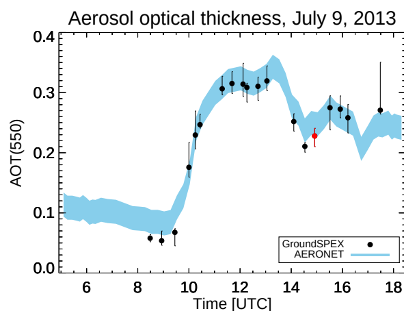
Figure 6. Aerosol optical thickness at 550 nm during the day of 9 July 2013 at Cabauw, the Netherlands. GroundSPEX diffuse-sky measurements are compared with AERONET direct-sun measurements. The red data point at 14:55 UTC is retrieved from the measurements displayed in Fig. 5.
