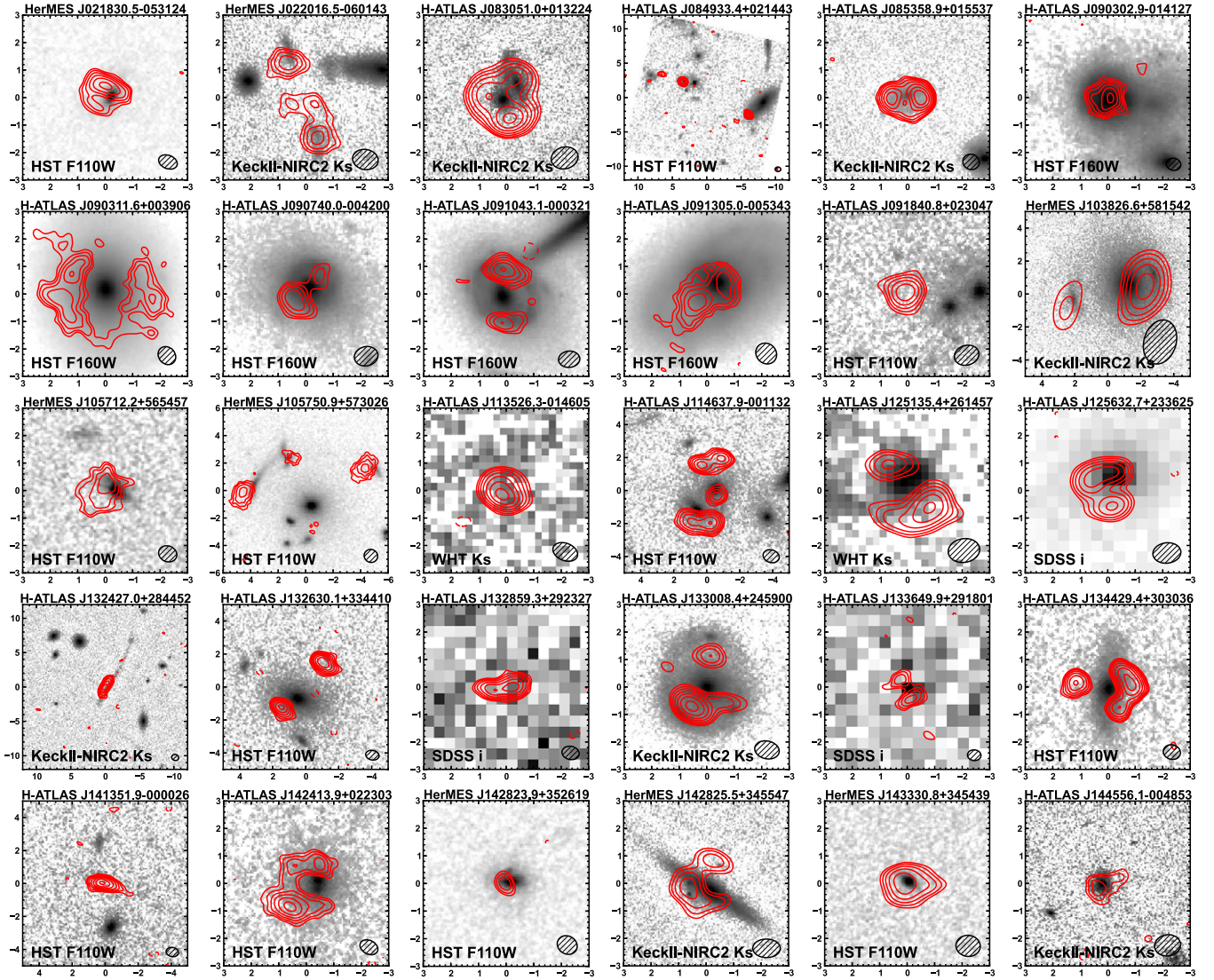
Figure 2. SMA 880 \mu\text{m} images (red contours, starting at \pm 3\sigma and increasing by factors of \sqrt{2} ) of candidate lensed SMGs from H-ATLAS and HerMES, overlaid on best available optical or near-IR images (logarithmic scaling; telescope and filter indicated in lower left corner of each panel). North is up and East is left, with axes having units of arcseconds relative to the 880 \mu\text{m} centroid as given in Table 1. The elliptical FWHM of the SMA's synthesized beam is shown in the lower right corner of each panel. The image separations are \approx 1\text{--}2'' , suggesting gravitational potential wells typical of isolated galaxies or small numbers of galaxies for the lenses (only two lensed sources are associated with galaxy clusters: J132427.0+284452 and J141351.9–000026).
