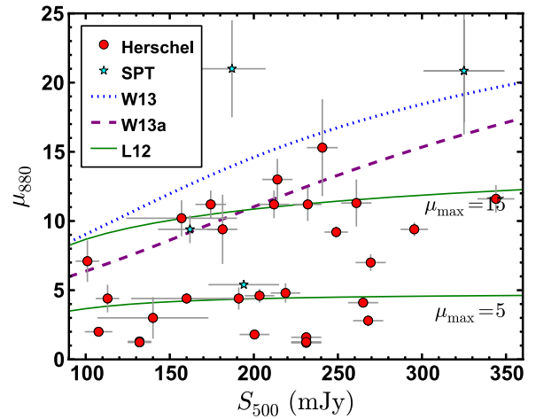
Figure 6. Magnification factor from the SMA lens model as a function of 500\text{ }\mu\text{m} flux density. The prediction for these values from Wardlow et al. (2013) is shown by the dotted blue line, whereas the dashed purple line traces the same model, but with parameters tuned to jointly match the observed number counts and magnification factors shown in this diagram. The solid green lines show the effects of different maximum magnifications and are taken from Lapi et al. (2012).
