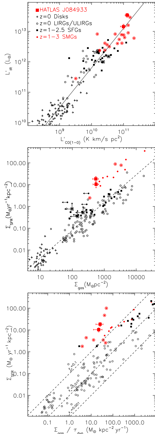
Figure 6. Plots relating the rate or surface density of star formation with the available gas. Components W and T are shown as red squares, with error bars, in each plot. Circled red symbols denote high-redshift measurements made directly in CO J = 1\text{--}0 . Low- and high-redshift star-forming galaxies (SFGs), e.g., z = 0 disks, LIRGs and ULIRGs, and z = 1\text{--}2.5 BzK galaxies, are taken from Genzel et al. (2010) for all three plots. Top: L_{\text{IR}} vs. L'_{\text{CO}} , where we find no compelling evidence that SMGs follow a different relation than the other SFGs. Middle: surface-density S-K relation, where W and T lie among hyperluminous SMGs, such as SMM J02399–0136 and GN 20, offset from the relation for other SFGs. Lower: Elmegreen–Silk relation between star formation surface density and the ratio of gas surface density and dynamical timescale. W and T exhibit extreme star formation efficiencies, even relative to SMGs. The fraction of their available gas converted into stars per dynamical timescale, \epsilon_{\tau} , is >0.1 . (A color version of this figure is available in the online journal.)
