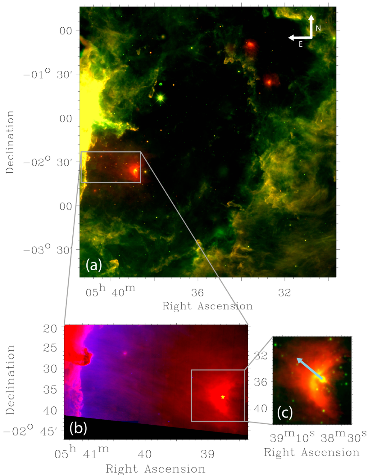
Fig. 1. a) Mid-IR view of the IC 434 region. The total field-of-view is 3.1^\circ \times 2.9^\circ . Green is the WISE-3 12\ \mu\text{m} band; red is the WISE-4 22\ \mu\text{m} band. b) Blown-up part of the upper image with different scaling to accentuate the extended emission around \sigma Ori AB. The Horsehead nebula is located at the top left. Here, blue represents H\alpha taken with the KPNO 4m telescope, whereas red is MIPS 24\ \mu\text{m} emission. The KPNO image does not extend over the entire field of view but cuts off 6' eastwards of \sigma Ori AB. c) Close up of the environs of \sigma Ori AB. Green is WISE-3, while red is MIPS 24\ \mu\text{m} . Overplotted is the proper motion vector which displays the movement in the plane of the sky.
