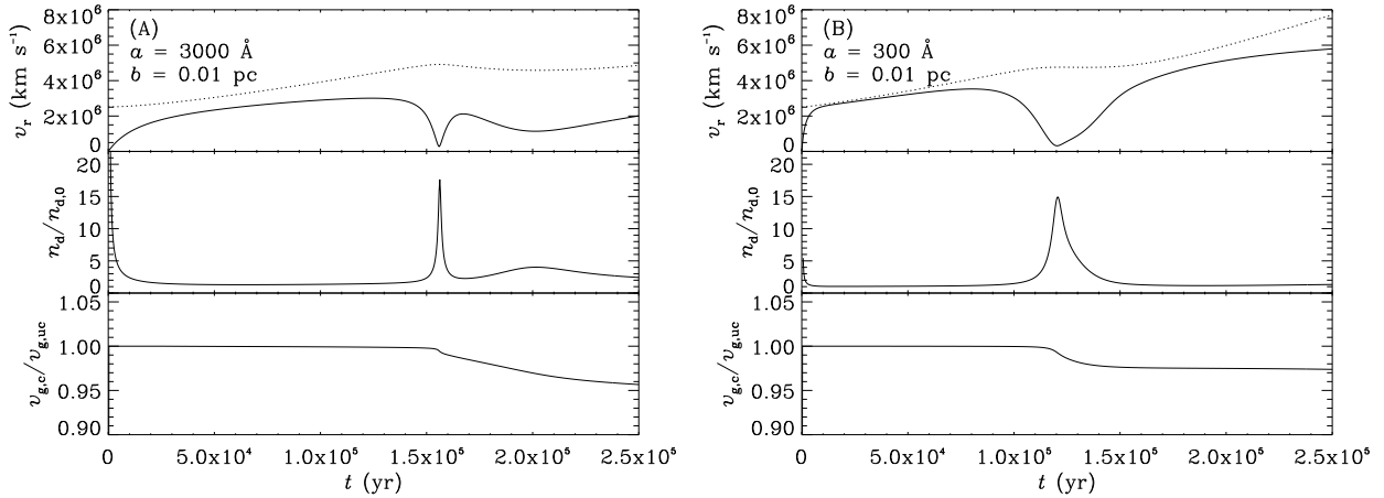
Fig. 6. Upper panels: radial velocity v_r of a dust grain (solid) and a gas particle (dotted, evaluated at the position of the dust grain in the frame of the star) as a function of time. At time t = 0 , the gas is ionized and enters the H II region. Middle panels: relative density increase in dust along the trajectory. This value approaches unity when the gas and dust are coupled. Lower panels: velocity ratio of a gas particle v_{g,c} , after momentum transfer with the dust, to an uncoupled gas particle v_{g,uc} , which reflects the amount of momentum transferred from the dust to the gas. a) Velocity, density increase and the amount of momentum transfer, evaluated for a 3000 Å dust grain with impact parameter b = 0.01 . b) Same figures, but for a dust grain with a 300 Å radius.
