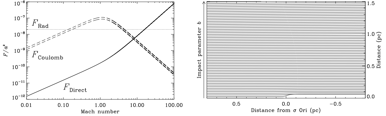
Fig. 9. Dependence of the direct drag force and Coulomb drag force on drift velocity and the structure of the photo-evaporation flow with the inclusion of Coulomb drag. Left: direct drag (solid line) and the Coulomb drag on a 300 \text{ \AA} dust grain with charge Z_d = 195 (upper dashed line) and a 3000 \text{ \AA} dust grain with charge Z_d = 1809 (lower dashed line). Plotted is the dependence of the drag forces on the relative velocity between the gas and the dust, expressed in the Mach number M = v_{\text{drift}}/c_s . The dotted horizontal line represents the radiation pressure force at r = 0.1 \text{ pc} . Right: calculated trajectories of a dust grain with \kappa_{\text{rp}} = 6.7 \times 10^3 including the Coulomb drag force. The grains only decouple from the gas very close to the star (i.e., d < 0.025 \text{ pc} ).
