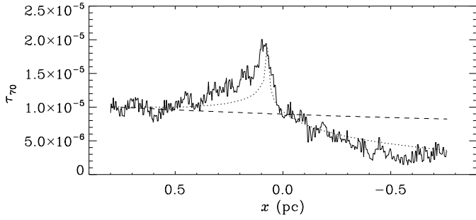
Fig. 8. A cross cut of the optical depth map in Fig. 3 taken horizontally through the stagnation point of the dust wave (solid). Overplotted is a model without radiation pressure force (dashed) and a model with radiation pressure force (dotted).
