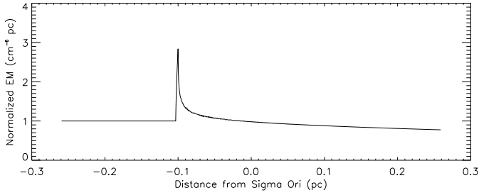
Fig. 10. Emission measure from the gas expected from a bow shock as described in Wilkin (1996), normalized to the expected background emission measure of the entire flow. The computed emission profile at resolution 0.26'' (the resolution of the KPNO H\alpha image) has been convolved with a Gaussian of width 1'' to account for (typical) astronomical seeing at the wavelength of H\alpha . A cut through the stagnation point and the star is shown, adopting wind parameters from Howarth & Prinja (1989) and ISM parameters calculated in Sect. 5.
