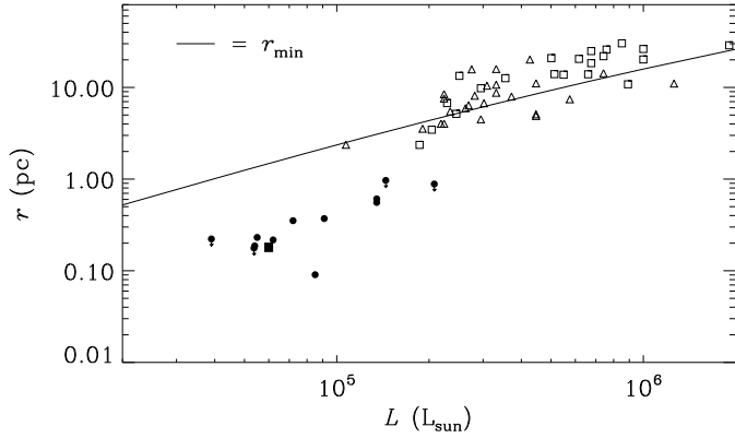
Fig. 12. Solid curve: r_{\min} for dust grains with \kappa_{\text{tp}} = 6.7 \times 10^3 \text{ cm}^2 \text{ g}^{-1} plotted as a function of luminosity L , assuming typical parameters for the stellar velocity ( =10 \text{ km s}^{-1} ) and an ISM density similar to the WNM ( =0.5 \text{ cm}^{-3} ). Overplotted are Galactic O-stars (open squares) and B-supergiants (open triangles) where wind parameters are taken from Puls et al. (1996) and Crowther et al. (2006). The filled circles are weak-wind objects from Bouret et al. (2003), Martins et al. (2004) and Najarro et al. (2011). \sigma Ori AB is marked as the filled square symbol.
