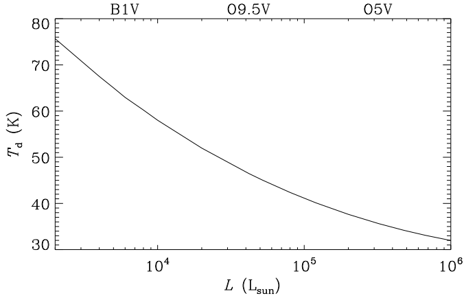
Fig. 14. Dust temperature T_d for silicate grains ( \kappa_{rp} = 6.7 \times 10^3 \text{ cm}^2 \text{ g}^{-1} ), located at r_{\min} , plotted as a function of luminosity L . For comparison, several spectral types for main sequence stars are plotted on the top axis.
