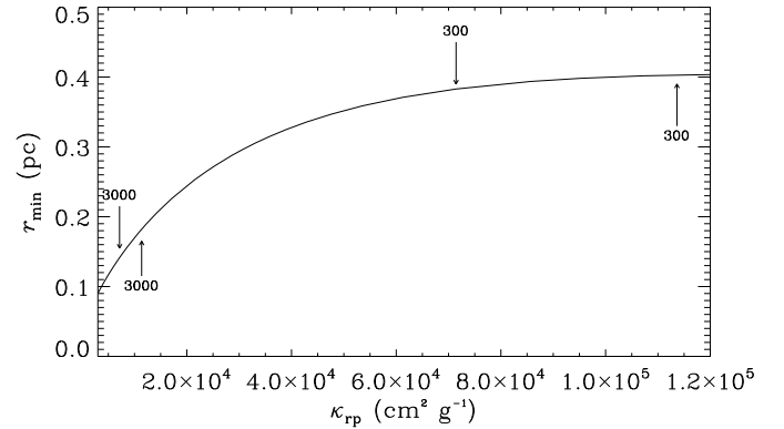
Fig. 7. Point of closest approach to the star r_{\min} versus radiation pressure opacity \kappa_{rp} for trajectories with b = 0 , assuming \bar{Q}_{rp} = 1 independent of grain size a . Labeled above the curve are typical grain sizes in angstroms for silicates. Below the curve are the corresponding grain size but for graphite grains.
