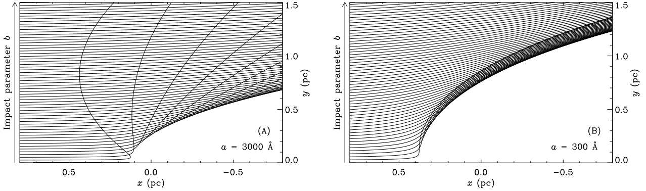
Fig. 5. Two dimensional plots of dust grain streamlines, evaluated for different grain sizes a . The x -axis represents the projected distance from L1630 to \sigma Ori, while the y -axis is the direction perpendicular to the line connecting L1630 and \sigma Ori AB, in the plane of the sky. a) Dust trajectories for a 3000 Å silicate grain trajectories for different values of impact parameter b . b) Same, but for a different value of \kappa_{\text{rp}} , which represents a 300 Å silicate grain.
