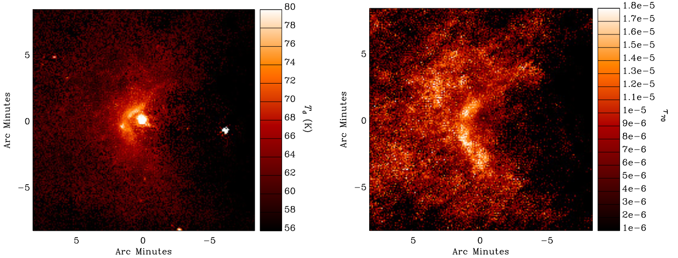
Fig. 3. Left: MIPS 24 \mu\text{m} versus 70 \mu\text{m} PACS dust color temperature map. The scale size is 16.5' \times 16.5' . Only pixels with values >3\sigma in the PACS 70 \mu\text{m} image are plotted. North is up, east is to the left. Right: 70 \mu\text{m} optical depth map.
