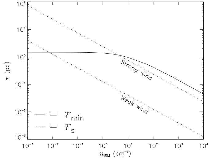
Fig. 13. r_{\min} and r_s as a function of ISM number density n_{\text{ISM}} . The stand-off distance r_s is plotted using wind parameters from Najarro et al. (2011, lower dotted line) and Vink et al. (2000, upper dotted line). r_{\min} reaches a maximum at n_{\text{ISM}} < 10 \text{ cm}^{-3} where the drag force F_d becomes negligible. r_s and r_{\min} show the same dependency on ISM density for n_{\text{ISM}} > 10 \text{ cm}^{-3} .
