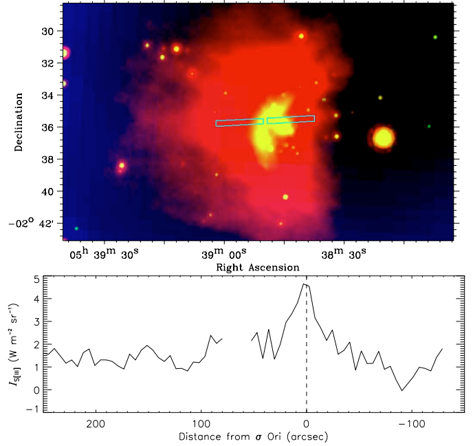
Fig. 11. Upper: 0.45^\circ \times 0.2^\circ three color image of the IR emission around \sigma Ori AB. Red is WISE-4 24\ \mu\text{m} , green is WISE-3 12\ \mu\text{m} and blue is H\alpha from the SHASSA mission, smoothed over 5 pixels in order to remove star residuals. Overplotted are the Spitzer /IRS LL2 regions. Lower: continuum subtracted and integrated intensity of the S[III] 18.7\ \mu\text{m} line inside the IRS regions as a function of distance towards \sigma Ori AB (a positive distance corresponds to the region in front of the star). The dashed line marks the position of \sigma Ori AB. The IR arc is located at \sim 0.1\text{--}0.4\ \text{pc} (the peak IR value being at \sim 0.1\ \text{pc} ), corresponding to 50\text{--}200\ \text{arcsec} in front of \sigma Ori AB.
