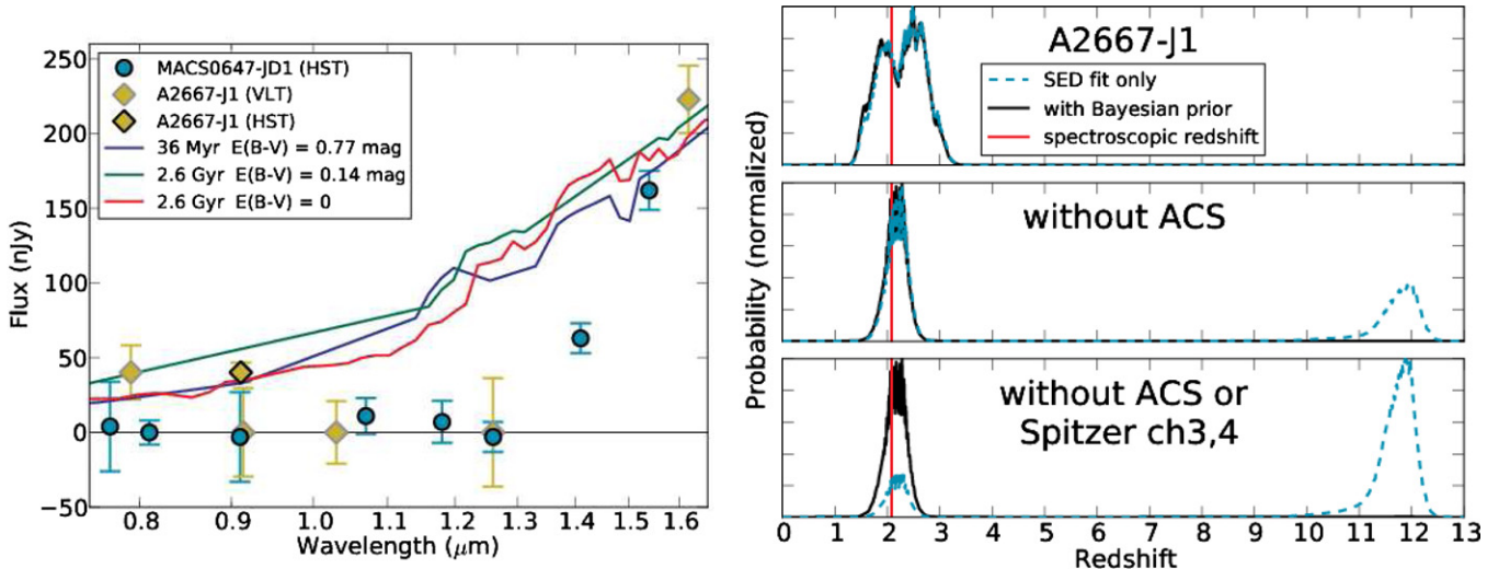
Figure 12. Left: comparison of near-infrared photometry of lensed J -dropouts MACS0647-JD1 (this work) and A2667-J1 (Laporte et al. 2011; Hayes et al. 2012). Also overplotted are three SED fits from Figure 2 of Hayes et al. (2012) to the photometry of A2667-J1 at its spectroscopic redshift z = 2.082 . The Hayes et al. (2012) photometry plotted here is all from VLT (FORIS2 and HAWK-I) except for the 6.0\sigma detection in HST /ACS F850LP, the upper diamond with a darker border at 0.91 \mu\text{m} . Right: photometric redshift probability distribution for A2667-J1 based on our reanalysis of the photometry provided in Hayes et al. (2012) with and without a Bayesian prior. The top panel uses all the available photometry. The middle panel omits the 6.0\sigma detection in ACS/F850LP. The bottom panel omits both ACS and Spitzer IRAC ch3 and ch4. The spectroscopic redshift z = 2.082 is indicated by the red vertical lines.
