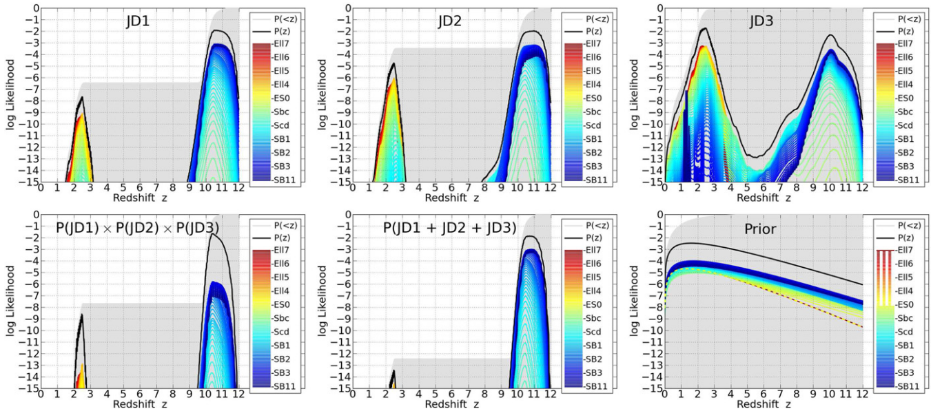
Figure 8. Top row: photometric redshift probability distributions based on our BPZ analysis (Section 4.1) of HST+Spitzer photometry for each image. Cumulative probabilities P(<z) are shaded gray; probabilities P(z) per unit 0.01 in redshift are drawn as black lines; and likelihoods for individual SED templates are drawn as colored lines. In this work, we use four elliptical templates (E11), one E/S0, two spirals (Sbc and Scd), and four starbursts (SB). We then interpolate nine templates between each pair of adjacent templates. Bottom left: joint likelihoods for all three images. Bottom center: likelihoods based on the summed photometry of all three images. For all of these likelihoods, we assume the prior plotted at bottom right for galaxies of an intrinsic (de lensed) magnitude of \sim 28.2 . This prior was empirically derived from large surveys with photometric and spectroscopic redshifts and extrapolated to higher redshifts.
