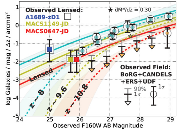
Figure 17. Observed number counts for both lensed (squares) and field (circles/arrows) galaxies at z \approx 8, 9.6, and 10.8 as a function of observed F160W AB magnitude. CLASH discoveries of candidates at z \approx 10.8 (MACS0647-JD; this work) and z \approx 9.6 (MACS1149-JD; Zheng et al. 2012) in \sim 78 \text{ arcmin}^2 (17 cluster lensing fields) are plotted as the red and yellow squares, respectively, in units of counts per unit magnitude, redshift, and square arcminute. The blue square indicates the single robust z \approx 7.5 candidate (A1689-zD1; Bradley et al. 2008) identified in 11 non-CLASH cluster fields covering 21 \text{ arcmin}^2 (Bouwens et al. 2009). Cyan and orange circles represent counts in unlensed fields at z \approx 8 and 10.3 , respectively, from the BoRG survey (Bradley et al. 2012b) as well as CANDELS, ERS, and HUDF09 (Oesch et al. 2012a) including UDFj-39546284 (Bouwens et al. 2011a). The arrows give both 1\sigma and 90% confidence upper limits from Oesch et al. (2012a). The bottom dashed curves are expected counts with uncertainties from the Bradley et al. (2012b) z \sim 8 luminosity function and extrapolated to z \sim 9.6 and 10.8 assuming an evolution of dM^*/dz = 0.30 , similar to that found in, e.g., Bouwens et al. (2008, 2012a; also see Figure 18). This yields F160W m^* \sim 27.0, 27.7, and 28.3 at these redshifts, plotted as a small star along each curve. We then simulate the lensing of these expected counts in our CLASH WFC3/IR survey area using mass models of the 17 clusters and excluding the area ( \sim 17\% ) covered by foreground objects. These are given as the upper solid curves, which are consistent with the CLASH discoveries (red and yellow squares).
