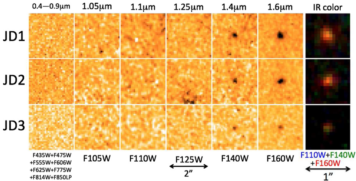
Figure 2. Three images of MACS0647-JD as observed in various filters with HST . The leftmost panels show the summed 11 hr (17-orbit) exposures obtained in eight filters spanning 0.4\text{--}0.9\ \mu\text{m} with the Advanced Camera for Surveys. The five middle columns show observations with the Wide Field Camera 3 IR channel in F105W, F110W, F125W, F140W, and F160W, all shown with the same linear scale in electrons per second. The F125W images were obtained at a single roll angle, and a small region near JD2 was affected by persistence due to a moderately bright star in our parallel observations immediately prior (see also Figure 4). The right panels zoom in by a factor of 2 to show F110W+F140W+F160W color images scaled linearly between 0 and 0.1\ \mu\text{Jy} .
