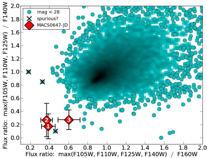
Figure 13. Observed NIR colors of the J -dropouts (red diamonds with 1\sigma uncertainties) plotted against those observed for all other 20,746 CLASH sources brighter than 28th magnitude in both F160W and F140W and also observed in F125W (filled circles and density map). The horizontal axis gives the ratio of the F160W flux to the maximum flux in all bluer WFC3/IR filters. The vertical axis gives a similar flux ratio but for F140W. Three objects with colors similar to the J -dropouts appear to be spurious IR artifacts based on visual inspection, and we mark these with X’s.
