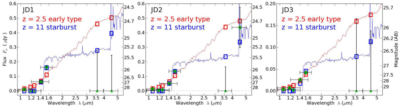
Figure 9. Observed NIR photometry from HST WFC3/IR and Spitzer IRAC (filled circles and triangles) compared to the expected fluxes (open squares) from two SEDs: the z = 11.0 starburst from Figure 3 (blue) and a z = 2.5 early-type galaxy (red). Note that the JD3 plot is scaled differently along the y-axis.
