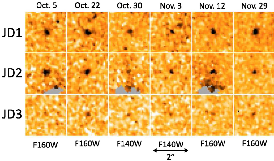
Figure 4. MACS0647-JD as observed in each of the individual epochs of F160W and F140W obtained over a 56 days period. These observations were obtained at two different telescope roll angles, which alternate between the stamps shown here. A small region of the WFC3/IR images in our first roll angle was affected by persistence due to a moderately bright star in our parallel observations immediately prior. These pixels happen to fall within 1'' of JD2 at that roll angle (marked in gray here and flagged as unreliable). Excluding this roll angle for JD2 does not significantly affect the derived photometry. (A color version of this figure is available in the online journal.)
