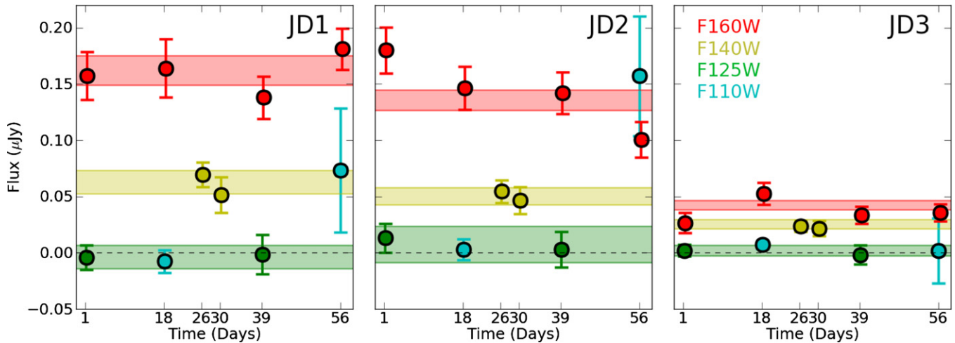
Figure 5. Flux measurements in the individual epochs observed over a period of 56 days. Filters are colored F160W (red), F140W (yellow), F125W (green), and F110W (blue) as both individual data points and solid bands, as determined for the summed observations. The F110W exposures obtained in the second epoch (visit A9) were found to have significantly elevated and non-Poissonian backgrounds due to earthshine (Section 3.1). These were excluded in our analysis; we adopted the F110W fluxes measured in the first epoch (visit A2). (A color version of this figure is available in the online journal.)
