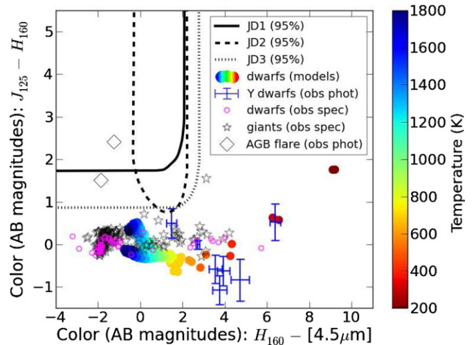
Figure 14. Observed colors in J_{125} , H_{160} , and at 4.5\ \mu\text{m} plotted as black lines (95% confidence contours) versus those observed and predicted for stars and brown dwarfs. Colors derived from stellar spectra observed with IRTF (Cushing et al. 2005; Rayner et al. 2009) are plotted as open magenta circles for dwarfs and open black star symbols for giants and supergiants. Blue error bars are observed photometry (ground-based and WISE ) for Y dwarfs (Kirkpatrick et al. 2012). Open black diamonds are post-AGB flare-ups with dust ejecta observed with 2MASS and WISE ; the upper diamond is “Sakurai’s object” (Duerbeck & Benetti 1996) and the lower diamond is WISE J1810–3305 (Gandhi et al. 2012). Simulated dwarf spectra from Hubeny & Burrows (2007) are plotted as filled circles colored as a function of temperature.
