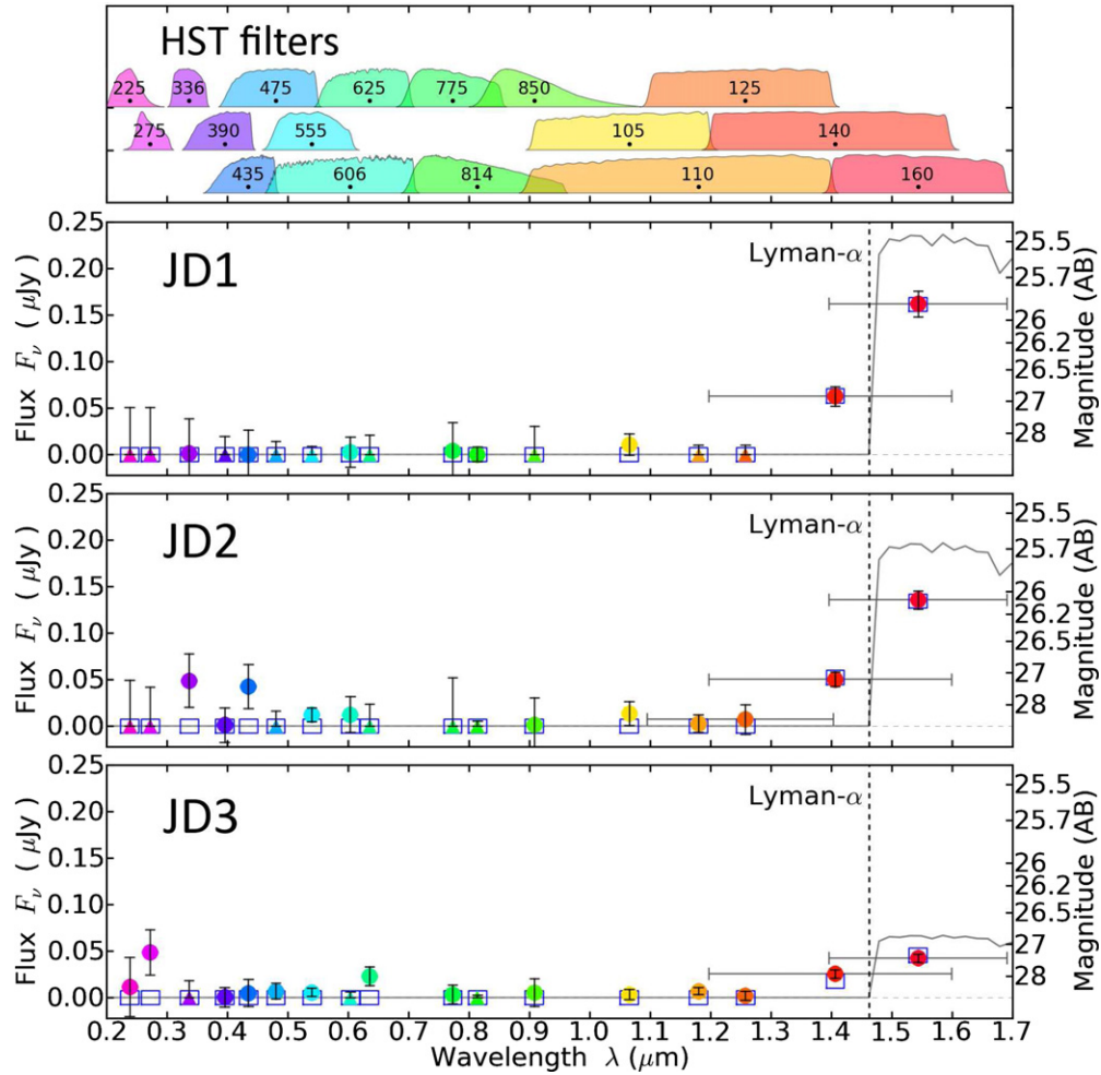
Figure 3. Observed HST photometry (filled circles and triangles) plotted against the expected fluxes (open blue squares) from a young starburst galaxy spectrum (gray line) redshifted to z \sim 11 . HST filter transmission curves are plotted in the upper panel, normalized to their maxima, and with black dots indicating the effective “pivot” wavelengths. Photometry of the J -dropouts observed through these filters (Table 3) is plotted as the larger circles and triangles for positive and negative observed fluxes, respectively, with 1\sigma error bars. For some points, horizontal “error bars” are plotted to reiterate the filter widths. The gray line is a model spectrum of a young starburst at z = 11.0 , the best fit to the summed photometry. The integrals of this spectrum through our filters give the model predicted fluxes plotted as blue squares. Other galaxy types at z \sim 11 yield similar predicted HST fluxes, as the shape of the spectrum cannot be constrained by the HST photometry alone. Redshifted Lyman- \alpha at 0.1216 \mu\text{m}(1+z) \sim 1.46 \mu\text{m} is indicated by the vertical dashed line.
