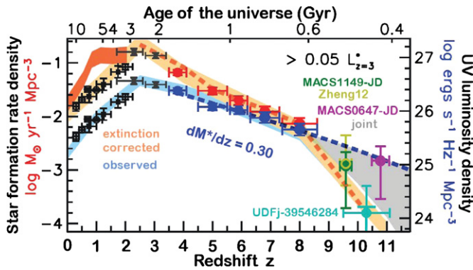
Figure 18. CLASH constraints on the cosmic star formation rate density at z \sim 9.6 and 10.8 compared to previous estimates from 0 \lesssim z \lesssim 10 as compiled and corrected for dust extinction by Bouwens et al. (2012b). We adopt the z \sim 8 LF from Bradley et al. (2012b) and assume M^* evolves with linearly redshift. MACS0647-JD constrains dM^*/dz = 0.33^{+0.35}_{-0.15} , while MACS1149-JD (Zheng et al. 2012) constrains dM^*/dz = 0.62^{+0.62}_{-0.24} , yielding a joint constraint of dM^*/dz = 0.44^{+0.29}_{-0.15} . We integrate these LFs down to 0.05 L^*(z = 3) , or M_{UV,1400} \approx -17.7 AB mag, to obtain rest-frame UV luminosity densities (magenta and green points with the gray shaded region giving the joint constraint). The yellow point is an alternative estimate of the z \sim 9.6 SFRD from Zheng et al. (2012) rescaled by 12/17 to account for the larger search volume behind 17 clusters. An extrapolation from z \sim 8 assuming dM^*/dz = 0.30 is shown as the dashed blue line. Points along the bottom blue curve are observed while the upper orange curve is corrected for extinction by Bouwens et al. (2012b). We assume that a star formation rate of one solar mass per year (left axis) produces a UV ( 0.14 \mu\text{m} ) luminosity of 8 \times 10^{27} \text{ erg s}^{-1} \text{ Hz}^{-1} (right axis), as from a Salpeter (1955) IMF truncated between 0.1 and 125 M_{\odot} . A Chabrier (2003) IMF would yield lower SFRD by a factor of \sim 1.8 . Previous data are from Schiminovich et al. (2005), Oesch et al. (2010b), Reddy & Steidel (2009), Bouwens et al. (2007, 2011a), and Oesch et al. (2012a) as described in Bouwens et al. (2012b, see their Figure 19).
