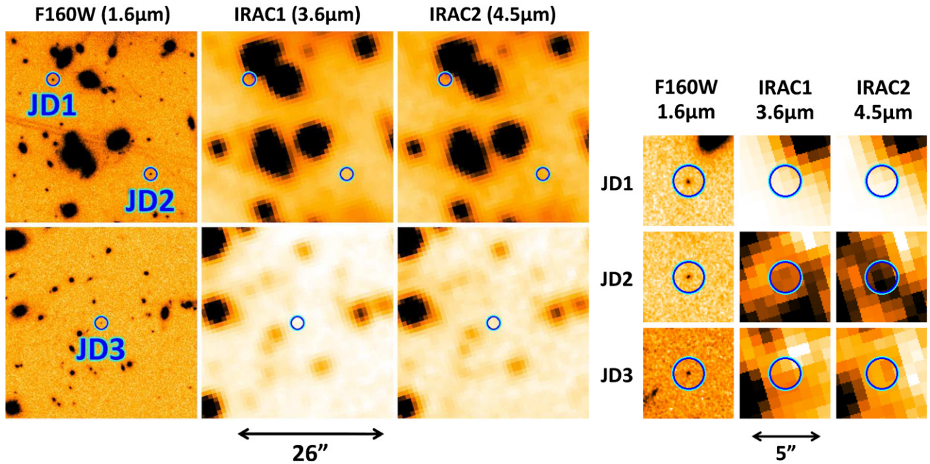
Figure 7. Spitzer IRAC ch1 ( 3.6 \mu\text{m} ) and ch2 ( 4.5 \mu\text{m} ) images of MACS0647-JD compared to the HST WFC3/IR F160W ( 1.6 \mu\text{m} ) image. Two intensity scalings and zooms are shown. Left: both 26'' \times 26'' F160W cutouts are scaled linearly in photon counts to the same range as in Figure 2. And for each Spitzer filter, the same count range is used in each row. The background photon counts are significantly higher near JD1 and JD2 (top row) due to intracluster light and scattered starlight. MACS0647-JD is not detected brightly in the Spitzer images, supporting the high-redshift solution. The only possible detection we report is for JD2 at 3.1\sigma in ch2 (Table 3). JD1 is contaminated by light from other nearby galaxies which we modeled and subtracted to estimate JD’s photometry. Right: in each of these 5'' \times 5'' closeups, the intensity is scaled independently to the observed range within the central 3'' \times 3'' .
