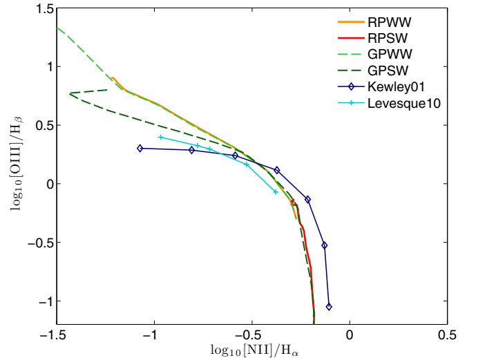
Figure 4. Comparison of model results on the BPT diagram. All results shown are for n_{\text{H, in}} = 10 \text{ cm}^{-3} and a spectrum corresponding to a zero-age stellar population. The D00 model (marked as Kewley01 in the legend) is shown in dark blue, the L10 model result is in light blue, and our model results are shown in orange and green lines.
