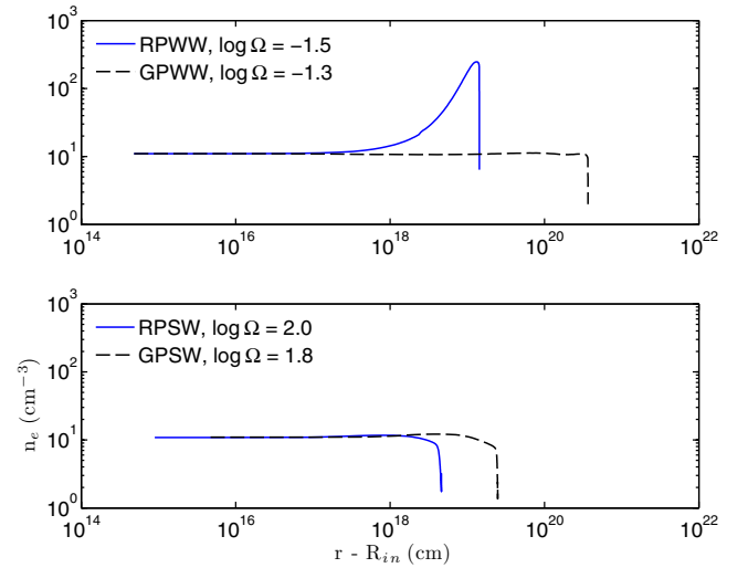
Figure 3. Electron density vs. radius for sample H II regions. Top panel: RPWW (blue solid line) and GPWW (black dashed line) regions. Bottom panel: RPSW (blue solid line) and GPSW (black dashed line) regions. The age of the ionizing star cluster in these regions is 0 Myr and the density at the inner boundary is 10 \text{ cm}^{-3} . The luminosity in all models is 10^{43} \text{ erg s}^{-1} . We select the value of R_{\text{in}} from our grid that gives \log \Omega closest to -1.5 and 2 ; exact values of \Omega for the four cases shown are as indicated in the legend. See Section 2.2 for details. Again we note that high luminosity is required here to reach radiation-pressure-dominated state because the density is low.
