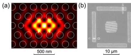
FIG. 2. (Color online) (a) Simulated electric field intensity in the modified L3-type cavity. The color scale goes from black (zero) to white (maximum intensity). (b) SEM image of a photonic crystal positioned near the center of a set of four gold markers. The lines on the upper and left markers are due to the detection procedure of the electron beam writer.
