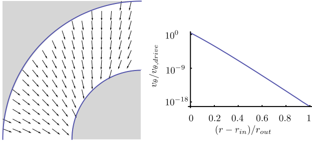
Fig. 2. (left) Vector field for the drift direction vector \hat{\mathbf{d}} in one quarter of a cylindrical Couette cell cross section (inner and outer radii r_{in} and r_{out} , respectively) driven with azimuthal velocity v_{\theta,drive} at the inner boundary. For a Couette geometry in the absence of gravity, the drift direction vector is identical in every cross section. Note that while the drift has a large inwards radial component, this will be compensated by an equal and opposite diffusion, resulting in only azimuthal flow in the steady state. (right) The azimuthal flow velocity as a function of radius on a logarithmic scale, illustrating the almost purely exponential fall-off of the velocity, consistent with for example Ref. [2].
