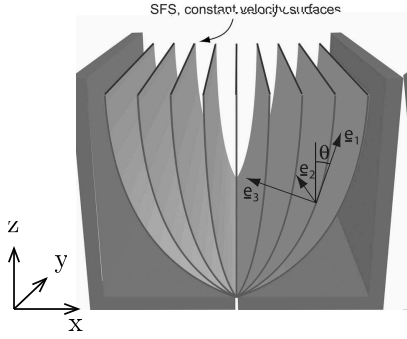
Fig. 5. A number of shear free sheets in a linear shear cell, the shear free sheet basis is indicated with e_{1,2,3} . Figure taken from Ref. [25].
