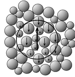
Fig. 1. Caricature [8,9] of a spot, a region where the density of grains is less than in the surrounding. When the spot moves upwards, the individual grains move downwards.
