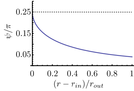
Fig. 6. (solid curve) The value of \psi , the angle between the radial axis and the axis of minor principal stress, as a function of radius in a planar Couette setup. According to the results of Ref. [24] this should always be close to \frac{1}{4}\pi (dashed line) or \frac{3}{4}\pi in a wide shear zone.
