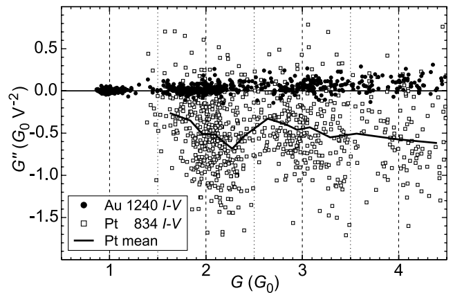
FIG. 2. Nonlinear term G'' vs low bias conductance G for Au and Pt ASCs. Each point represents a fit to Eq. (1) of one I - V curve on one ASC. There are points from 1240 Au and 834 Pt I - V curves. The solid curve represents the mean value of G'' for Pt. It is drawn through points found by averaging over 50 successive Pt points.
