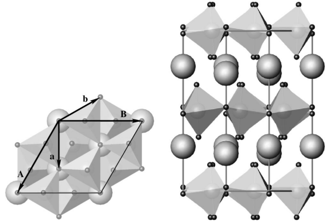
FIG. 1. Hexagonal \text{RMnO}_3 at room temperature, SG P6_3cm , (AB) plane (left), (BC) plane (right), big spheres R, small spheres O, Mn lies in the middle of the coordination polyhedra. In addition the hexagonal axes of the low-temperature phase P6_3cm \vec{a} , \vec{b} and of the high-temperature phase P6_3/mmc , \vec{A} , \vec{B} are depicted (left).
