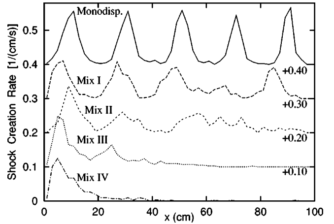
FIG. 12. Shock creation rates for monodisperse flow and polydisperse Mix I,II,III,IV. for \beta=0.4^\circ , D=10\text{mm} .
