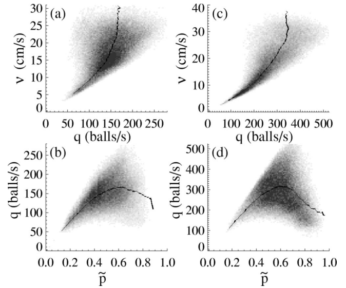
FIG. 14. Fundamental diagrams in rough wall flows. (a) and (b) Pipe flow studied in the interval 37 < x < 74 cm for \beta = 0.0^\circ and D = 15 mm. (c) and (d) Intermittent flow studied in the interval 0 < x < 37 cm for \beta = 0.4^\circ and D = 20 mm.
