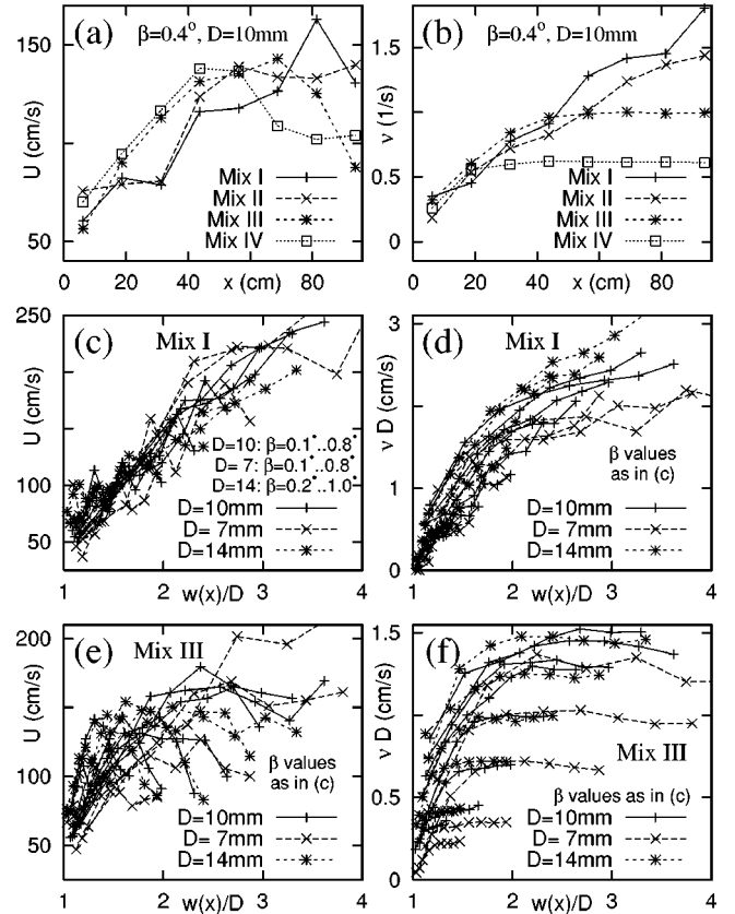
FIG. 13. RGE based plots of U(x) (a,c,e) and \nu(x) (b,d,f): (a) shows U(x) vs x at \beta=0.4^\circ , D=10\text{mm} for Mix I-IV. (b) shows \nu(x) vs x at \beta=0.4^\circ , D=10\text{mm} for Mix I-IV. (c) shows U(x) vs. w(x)/D for Mix I. (d) shows \nu(x)D vs w(x)/D for Mix I. (e) shows U(x) vs w(x)/D for Mix III. (f) shows \nu(x)D vs w(x)/D for Mix III. [In each of (c-f) 18 data sets are displayed.]
