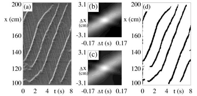
FIG. 15. Illustration of methods used to obtain shock velocities and frequencies for pipe flow for the case of D = 20 mm. (a) Modified density plot. (b) and (c) Space-time correlation functions based on data shown in (a), for (b) x = 130 cm, and (c) x = 170 cm. Note that the scales of (a), (b), and (c) are different, so that the dominant angles appear different. (d) Thresholded data used for determination of shock frequency.
