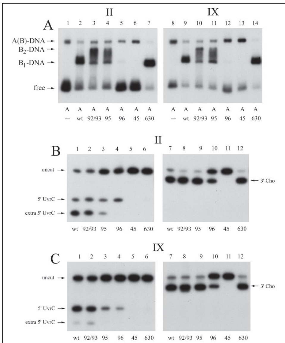
FIGURE 7. Complex formation and incisions in the presence of the mutant UvrB proteins. A, substrates II and IX were incubated with 1.25 nM UvrA and 100 nM (mutant) UvrB for 10 min at 37 °C. The mixtures were analyzed on 3.5% native polyacrylamide gels containing 1 mM ATP. Lanes 1 and 8, no UvrB; lanes 2 and 9, wtUvrB; lanes 3 and 10, UvrB(Y92A/Y93A); lanes 4 and 11, UvrB(Y95A); lanes 5 and 12, UvrB(Y96A); lanes 6 and 13, UvrB(K45A); lanes 7 and 14, UvrB630. The positions of the different protein-DNA complexes are indicated with arrows. UvrB 1 -DNA has a UvrB monomer bound to the DNA and UvrB 2 -DNA contains the UvrB dimer. B and C, substrates II and IX were incubated with 2.5 nM UvrA, 100 nM (mutant) UvrB, and 25 nM UvrC (lanes 1–6) or Cho (lanes 7–12) at 37 °C for 30 min. The incision products were analyzed on a 15% denaturing polyacrylamide gel. Lanes 1 and 7, wtUvrB; lanes 2 and 8, UvrB(Y92A/Y93A); lanes 3 and 9, UvrB(Y95A); lanes 4 and 10, UvrB(Y96A); lanes 5 and 11, UvrB(K45A); lanes 6 and 12, UvrB630. The incision products are indicated with arrows.
