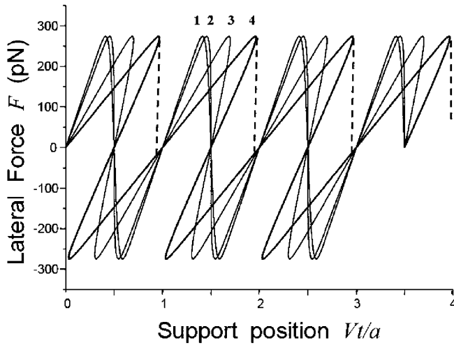
FIG. 4. Lateral force F as a function of the support position Vt , for U_0 = 0.3 eV, a = 0.25 nm, and k = 3.5 N/m. Force loops 1, 2, 3, and 4 correspond to K = \infty, 26, 4 , and 2 N/m, respectively. Dashed lines indicate mechanical slips of the tip (shown for case 4 only).
