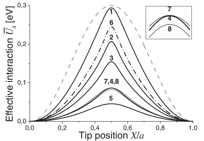
FIG. 3. Effective tip-surface interaction \bar{U}_s as a function of the tip position X for U_0 = 0.3 eV, a = 0.25 nm, and T = 300 K. Curves 1, 2, 3, 4, and 5 correspond to k = 15.2, 6, 4, 2 , and 1 N/m ( \gamma = 1, 2.5, 3.8, 7.6 , and 15.2 , respectively). 6—the same as 4, but with a = 0.5 nm; 7—the same as 4, but with T = 400 K; 8—the same as 4, but with U_0 = 0.2 eV. The dashed upper line represents the true surface potential. Only one period is shown.
