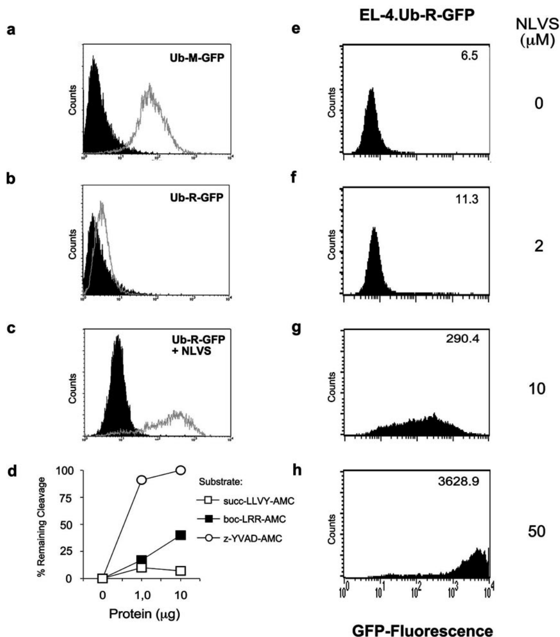
FIG. 4. Measuring proteasomal degradation by fluorescent ubiquitinated substrates in live cells. Shown are the results from FACS analysis of EL-4 cells stably transfected with Ub-M-GFP ( a ) or Ub-R-GFP ( b and c ). EL-4.Ub-R-GFP cells were left untreated ( b ) or were treated with 10 \mu\text{M} NLVS ( c ). The level of proteasomal activity in EL-4.Ub-R-GFP cells treated with 10 \mu\text{M} NLVS was measured by cytosolic high molecular mass protein ( 100,000 \times g , 5 h) cleavage of the fluorogenic peptide substrates succinyl ( succ )-LLVY-AMC, t -butyloxycarbonyl ( boc )-LRR-AMC, and benzyloxycarbonyl ( z )-YVAD-AMC ( d ). Also shown are the results from FACS analysis of EL-4.Ub-R-GFP cells treated with up to 50 \mu\text{M} NLVS ( e-h ).
