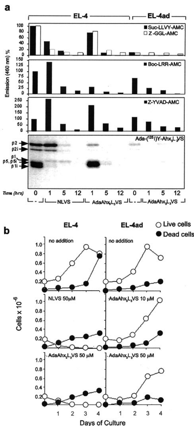
FIG. 6. EL-4ad cell proliferation despite inhibition of all catalytic sites of the proteasome by Ada-Ahx 3 -Leu 3 -VS. a , control EL-4 or EL-4ad cells were incubated with either 50 μM NLVS or 50 μM Ada-Ahx 3 -Leu 3 -VS for the indicated times, and cell lysates were submitted to differential centrifugation for partial purification of proteasomes. The samples were either tested for cleavage of the peptide reporter substrates succinyl (Suc)-LLVY-AMC, benzyloxy-carbonyl-GGL-AMC, t -butyloxycarbonyl (Boc)-LRR-AMC, and benzyloxy-carbonyl (Z)-YVAD-AMC (upper three panels) or labeled with Ada- [125] I-Tyr-Ahx 3 -Leu 3 -VS, followed by SDS-PAGE and autoradiography (lower panel). b , EL-4ad cell viability was mostly independent of proteasomal proteolysis. EL-4 (left panels) or EL-4ad (right panels) cells were left untreated (upper panels) or were incubated with 50 μM NLVS (middle left panel) or 10 μM (middle right panel) or 50 μM (lower panels) Ada-Ahx 3 -Leu 3 -VS for the indicated times. Live (○) and dead (●) cells were counted by trypan blue exclusion.
