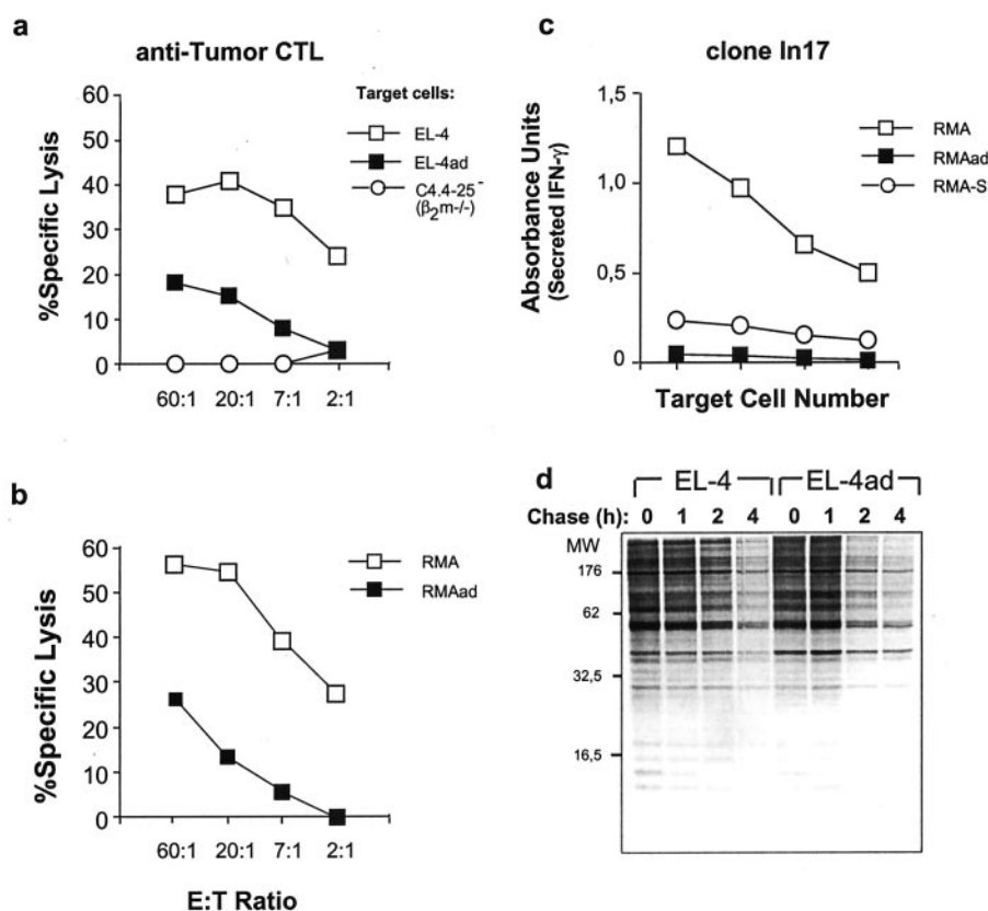
FIG. 2. Decreased tumor antigen presentation due to reduced reliance on proteasomal activity. ^{51}\text{Cr} release assays were performed using antitumor-specific CTLs tested against ^{51}\text{Cr} -labeled EL-4 (a) and RMA (b) target cells. RMA-S and C4.4-25 - are MHC class I mutant cell lines used to control for nonspecific target cell killing. Tumor antigen (NK-GENAQAI 30 )-specific CTL clone In17 was used to test antigen presentation by RMA, RMA-S, and RMAad cells (c). Antigen recognition was quantified by detection of IFN- \gamma secretion by effector cells, as described previously (31). Bulk protein turnover was assessed by metabolic labeling of control EL-4 and EL-4ad cells with ^{35}\text{S} for 15 min, and the fate of radiolabeled proteins was followed by a chase for the indicated times, SDS-PAGE separation, and autoradiography (d). \beta_2\text{m}^{-/-} , \beta_2 -microglobulin-deficient; E/T , effector to target ratio.
