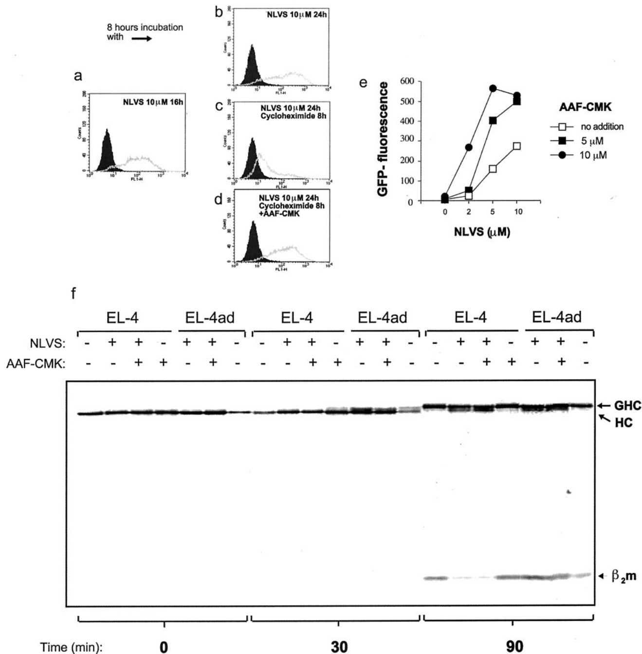
FIG. 5. Degradation of an N-end rule substrate is influenced by non-proteasomal oligopeptidases. Shown are the results from FACS analysis of EL-4.Ub-R-GFP cells incubated with 10 \mu M NLVS for 16 h (a) and further incubated for 8 h in the presence of no addition (b), cycloheximide (c), or 10 \mu M AAF-CMK (d). EL-4.Ub-R-GFP cells were incubated in the presence of NLVS (0, 2, 5, or 10 \mu M) in combination with AAF-CMK (0, 5, or 10 \mu M) (e). Control EL-4 and EL-4ad cells were pulsed with [ 35 S]methionine, and transport of H-2K b molecules was followed by immunoprecipitation and SDS-PAGE in the presence (+) or absence (-) of 50 \mu M NLVS and 10 \mu M AAF-CMK (f). The cells were incubated with the protease inhibitors for 3 h prior to metabolic labeling. GHC , glycosylated heavy chains; HC , heavy chains; \beta_2 m, \beta_2 -microglobulin.
