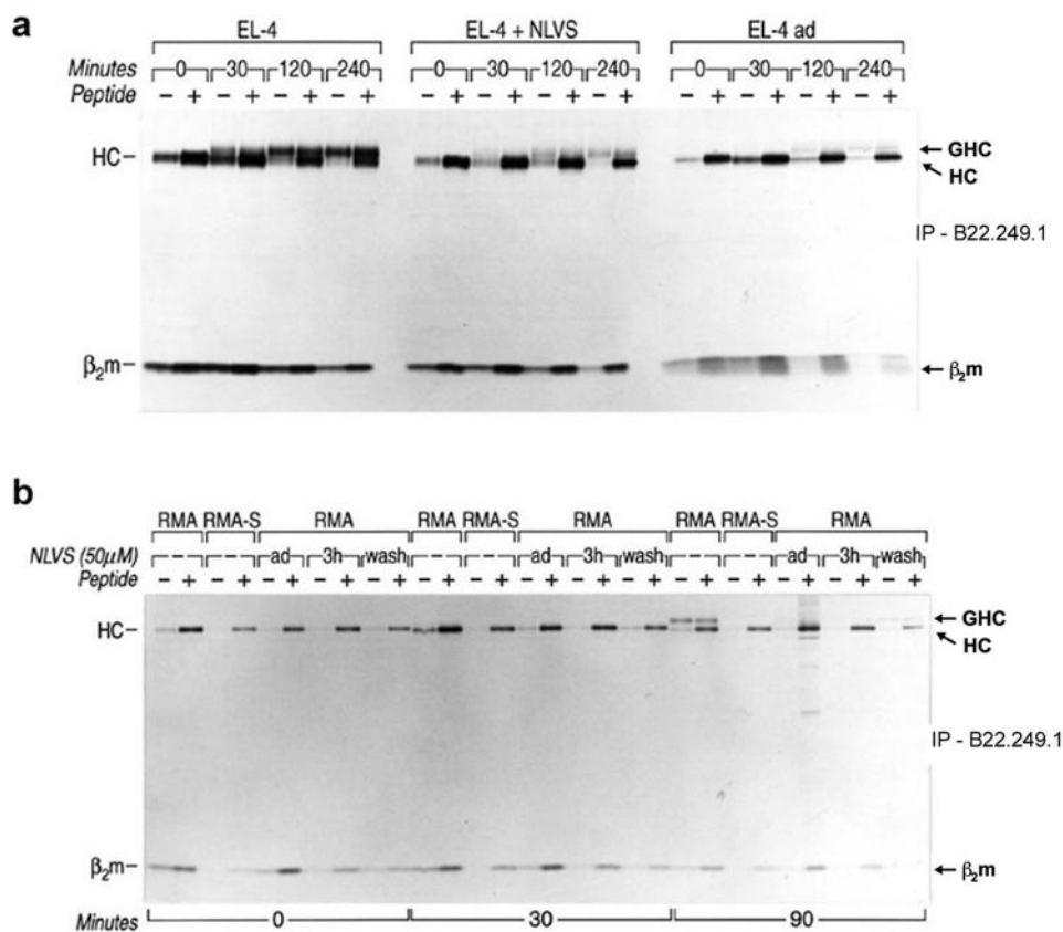
FIG. 1. Impaired assembly of MHC class I molecules in cells with reduced reliance on proteasomal activity. a , pulse-chase experiments were performed on control EL-4 cells, EL-4 cells treated with 50 \mu M NLVS for 16 h, or EL-4ad cells. H-2D b molecules were immunoprecipitated (IP) with anti-H-2D b antibody B22.249.1 in the presence or absence of an H-2D b -binding peptide, followed by SDS-PAGE analysis and autoradiography. b , RMA cells left untreated or treated with 50 \mu M NLVS for 3 h (3h), adapted (ad) to 50 \mu M NLVS (RMAad), or adapted to NLVS and washed (wash) and RMA-S cells were subjected to pulse-chase experiments. H-2D b molecules were immunoprecipitated in the presence or absence of an H-2D b -binding peptide, followed by SDS-PAGE analysis and autoradiography. Glycosylated heavy chains (GHC) that were transported from the endoplasmic reticulum, heavy chains (HC), and \beta_2 -microglobulin ( \beta_2m ) are indicated with arrows.
