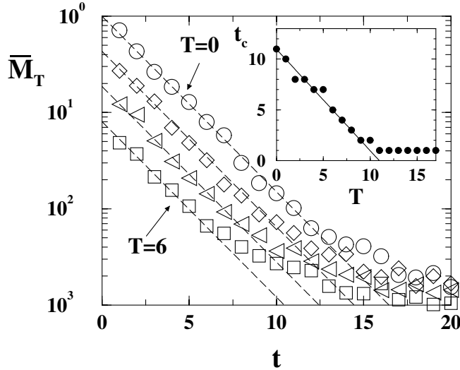
FIG. 1. Decay of the average fidelity \overline{M}_T for the kicked top with parameters \phi = 1.2 \times 10^{-3} , K = 3.9 and for preparation times T = 0 (circles), 2 (diamonds), 4 (triangles), and 6 (squares). In each case, the dashed lines give the analytical decay \overline{M}_T = \exp[-\lambda(t+T)] , in the Lyapunov regime with \lambda = 0.42 . Inset: threshold time at which \overline{M}_T(t_c) = M_c = 10^{-2} . The solid line gives the analytical behavior t_c = -\lambda^{-1} \ln M_c - T .
