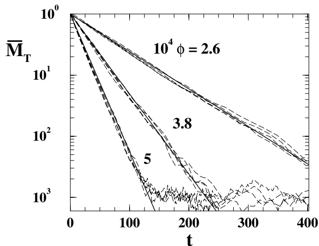
FIG. 2. Decay of \bar{M}_T in the golden rule regime for \phi = 2.6 \times 10^{-4} , 3.8 \times 10^{-4} , 5 \times 10^{-4} , K = 13.1 , and for preparation times T = 0, 5, 10 , and 20 (nearly indistinguishable dashed lines). The solid lines give the corresponding golden rule decay with \Gamma = 0.84\phi^2 S^2 [9].
