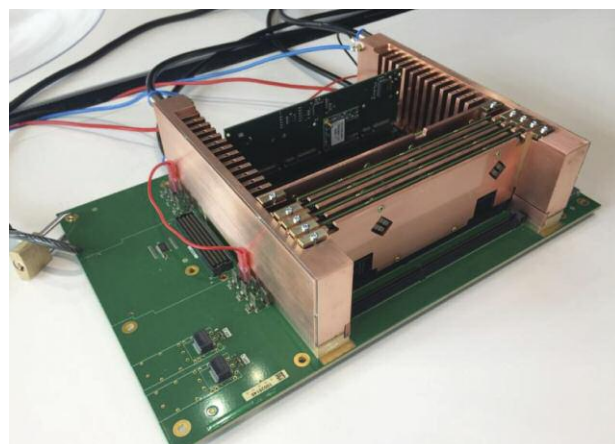
Figure 3: Microserver cluster demonstrator. Cooling water is delivered to the stack of cards via the manifolds on the left- and right-hand sides.
