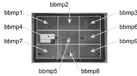
Figure 1. Measurement points in the laptop neighborhood: at the top part of a portable computer (left), at the bottom part of a portable computer (right).
