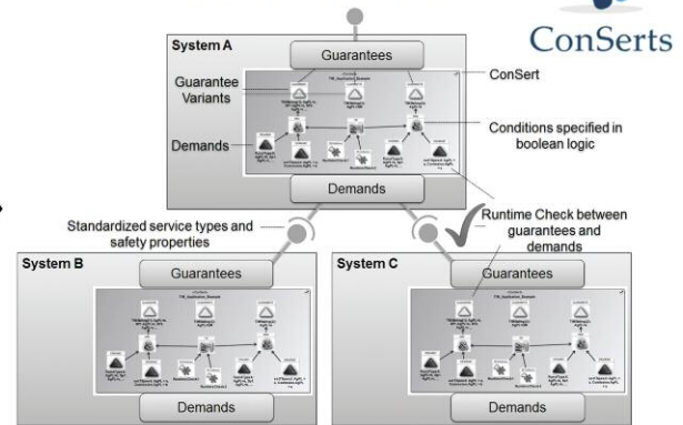
Figure 1: WEFACT addresses safety and security co-engineering at development time and ConSerts addresses CPS certification at Runtime. Both come together in the EMC 2 project.
