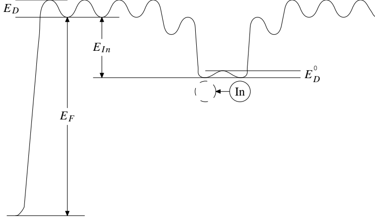
Fig. 13. One-dimensional energy landscape for a vacancy in the Cu(001) surface. For this one-dimensional situation the vacancy is formed at the step on the left and approaches the indium from there. It is only able to displace the indium atom to the left by one atomic spacing. E_F is the formation energy of a Cu(001)-vacancy, E_D is the diffusion barrier for a Cu(001)-vacancy, E_D^0 is the vacancy-indium exchange barrier and E_{In} is the binding energy for an indium-vacancy pair.
