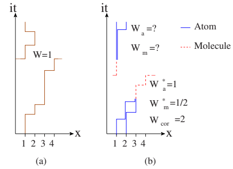
FIG. 2. (Color online) Example of world lines for a four-site lattice with periodic boundary conditions. (a) For a system without conversion between the different species, the world lines are continuous and the winding number is well defined. (b) The conversion between atoms and molecules leads to discontinuities in the world lines, and no true winding can be defined for each of the species. However, it is well defined for the atom-molecule mixture, because the composite world lines are continuous (see text for details).
