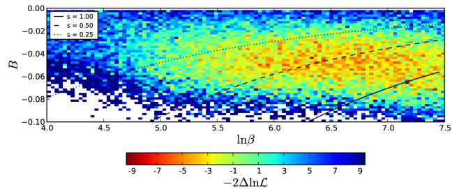
FIG. 3 (color online). Profile of \Delta\chi_{\text{eff}}^2 = -2\Delta\ln\mathcal{L} for the mode \mathcal{B} in the (\ln\beta, B) plane, showing the degeneracy between B and \ln\beta , and lines of s = \text{const} . Notice how the mode saturates the s < 1 bound.
