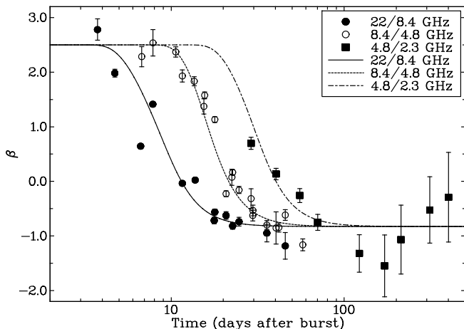
FIG. 5.— Spectral indices of SN 2008D based on the observed flux ratios between 22 and 8.4 GHz (solid circles), 8.4 and 4.8 GHz (open circles), 4.8 and 2.3 GHz (solid squares). The lines show the evolution of the spectral indices based on the model fits shown in Figure 1.
