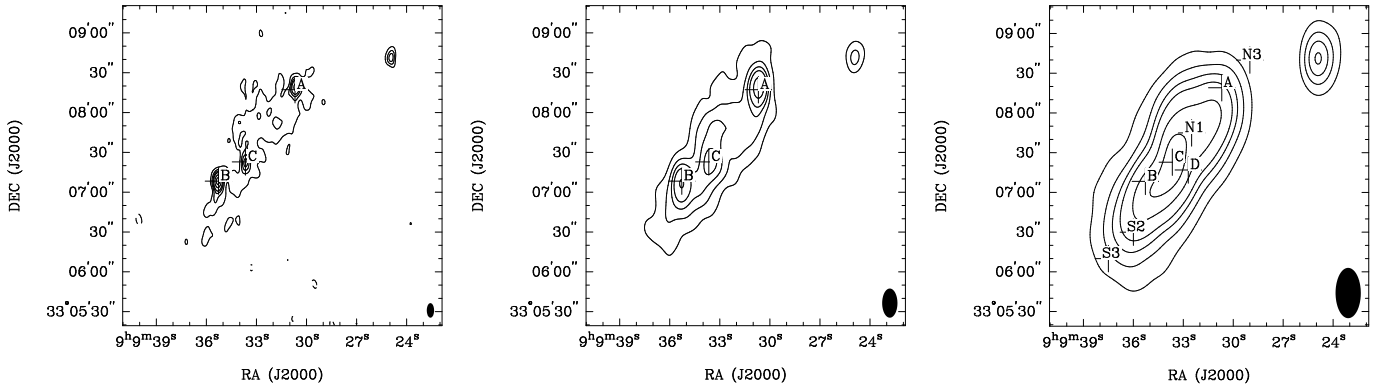
FIG. 3.— WSRT maps of the NGC 2770 field at 4.8 GHz (left), 2.3 GHz (middle), and 1.4 GHz (right), with the beam size plotted in the lower right corner of each panel. Indicated are SN 2008D (A), SN 2007uy (B), the core of NGC 2770 (C), and SN 1999eh (D). On the 1.4 GHz map the ARO observation positions are also shown (see Table 2 for the coordinates). Radio brightness contours are given at the -3, 3, 6, 9, 12, 18, 24, 30 sigma levels. We note that the compact source in the right hand corner of each panel has a spectral index of -1.2 , and is not significantly variable over our \sim 600 days of observations.
