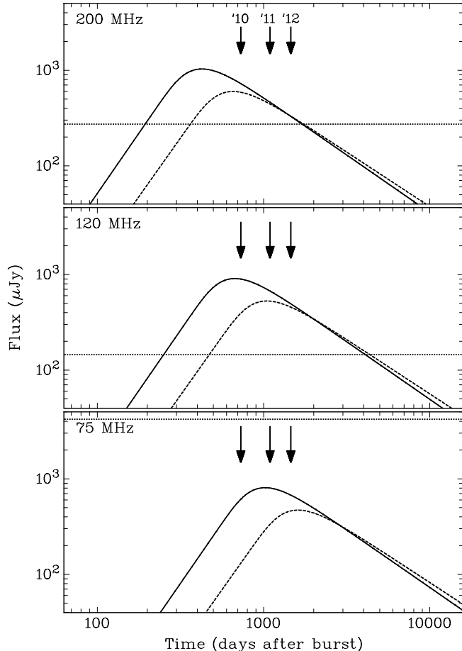
FIG. 6.— Predicted light curves of SN 2008D (solid lines) and SN 2007uy (dashed lines) at three frequencies in the LOFAR observing range. The dotted lines indicate the LOFAR sensitivity, at the 3\sigma -level after 4 hours integration. The vertical arrows indicate January 1 of the years 2010, 2011 and 2012.
