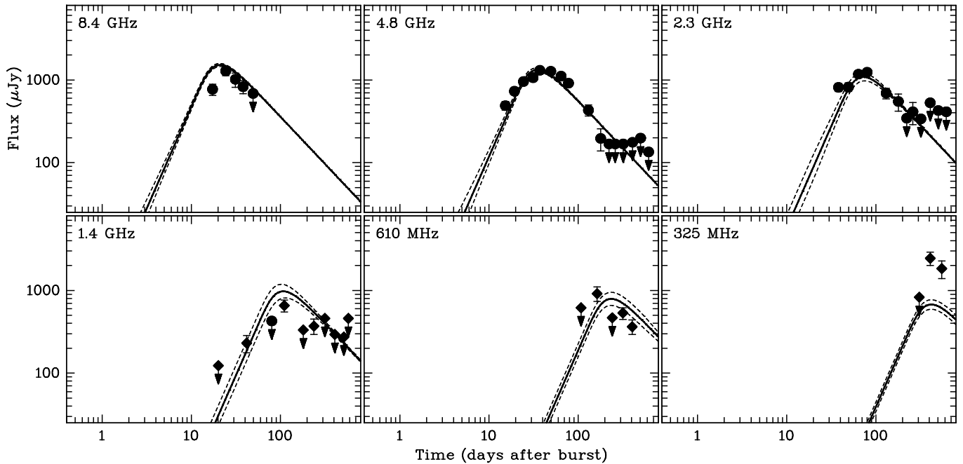
FIG. 2.— Light curves of SN 2007uy from WSRT (circles) and GMRT (diamonds). The solid lines represent the best broadband fit to the data, while the dashed lines indicate the flux modulation effects of interstellar scintillation. The flux values in Table 1 which are lower than three times their flux uncertainty, are plotted as 3\sigma upper limits.
