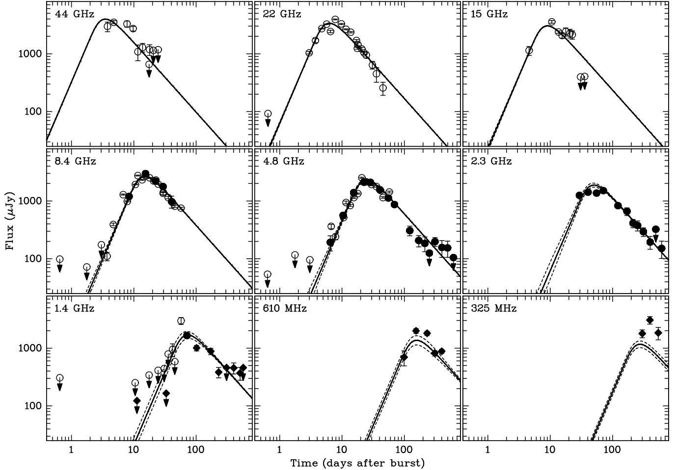
FIG. 1.— Light curves of SN 208D from WSRT (solid circles), GMRT (solid diamonds), and VLA (open circles); VLA fluxes are adopted from Soderberg et al. (2008). The solid lines represent the best broadband fit to the data, while the dashed lines indicate the flux modulation effects of interstellar scintillation. The flux values in Table 1 which are lower than three times their flux uncertainty, are plotted as 3\sigma upper limits.
