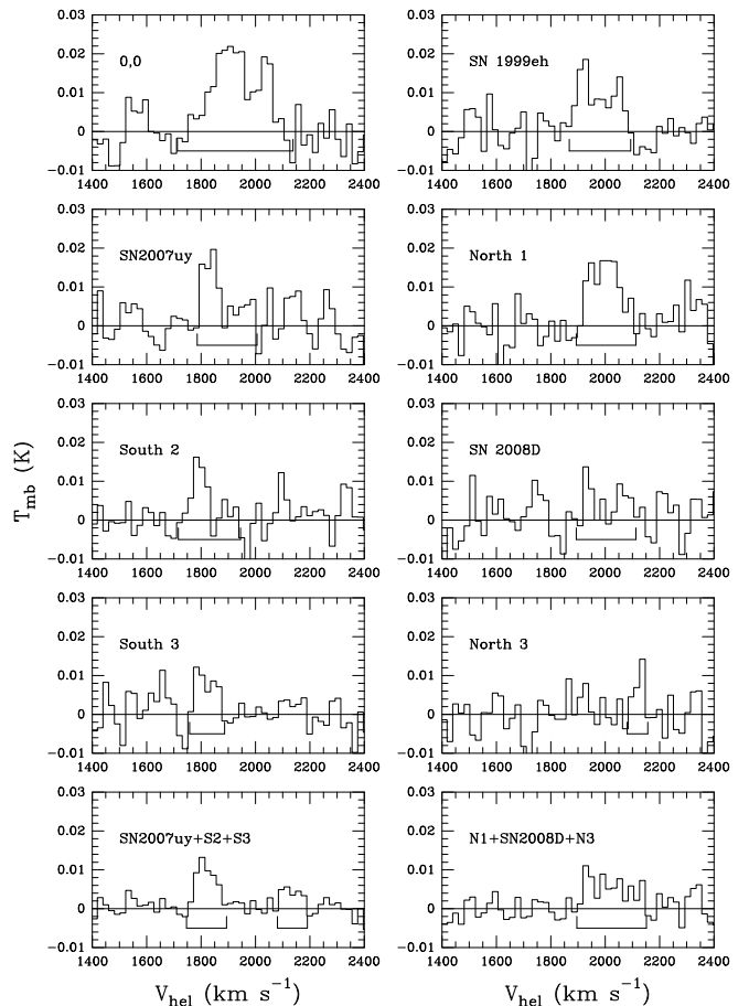
FIG. 4.— CO J = 1 \rightarrow 0 added and smoothed spectra, with positions indicated. The solid lines below the emission indicate the line windows used to determine the integrated intensities.
