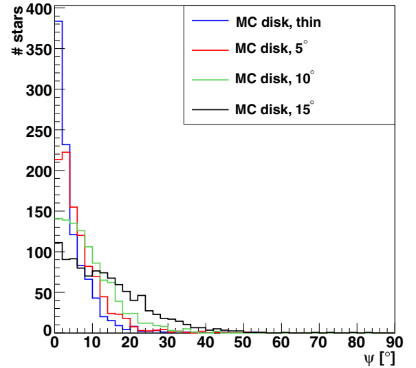
Figure 9. Distribution of the reconstructed angular deviation \psi of the disk stars from the common disk angular momentum direction for four MC-generated disk of 1000 stars each, with 0^\circ , 5^\circ , 10^\circ , and 15^\circ thickness.
