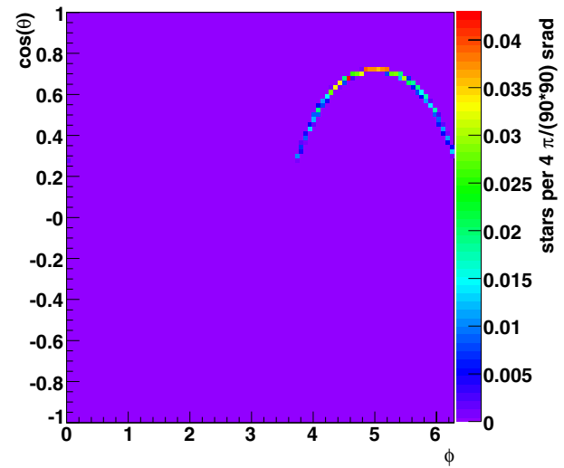
Figure 5. Cylindrical equal area projection of the distribution of the direction of the angular momentum vector ( \cos \theta_J vs. \phi_J ) for the star IRS16 CC for 1000 generated z -values. The z -coordinate is generated according to Equation (3) (assuming a power law stellar surface density with exponent \beta = 2 ). Only z -values of bound orbits are considered. Clockwise orbits have angular momentum directions in the upper hemisphere ( \cos \theta > 0 ) and counterclockwise orbits have angular momentum directions in the lower hemisphere ( \cos \theta < 0 ).
