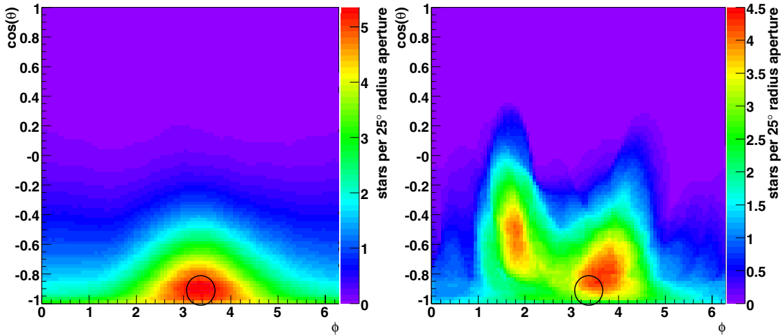
Figure 21. Cylindrical equal area projections of the density of reconstructed angular momenta in an aperture of 25^\circ radius (left) average for an MC-simulated disk of many stars, scaled to 15 stars. The disk angular momentum points in the direction of the counterclockwise disk of Paumard et al. (2006). (Right) 15 MC-simulated stars with the same azimuthal distribution as the observed stars. All 15 stars are members of a disk ( 10^\circ thickness) in the direction of the counterclockwise disk of Paumard et al. (2006).
