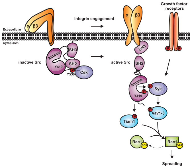
Fig. 4. Src binding to \beta 3 integrins influences cell spreading via regulation of Rac1 GTP loading. Following ligand binding, \alpha \text{Ib} \beta 3 and \alpha \text{v} \beta 3 integrins can directly interact with the SH3 domain of Src via the cytoplasmic domain of integrin \beta 3 . These interactions result in a release of Csk from tyrosine 530 and induce the activation of Src. Clustering of \beta 3 integrins promotes transphosphorylation in the kinase domain of Src. This is followed by the recruitment and phosphorylation of Syk, which can occur in concert with signaling downstream from growth-factor receptors. Activated Syk phosphorylates Vav proteins, which act as GEFs for Rac1. Alternatively, activated Src can phosphorylate and regulate the activation of the RacGEF Tiam1. In turn, activated Rac1 induces membrane protrusions and spreading. Broken arrows indicate transition not supported by presented pathway or not supporting presented output. See main text for additional details.
