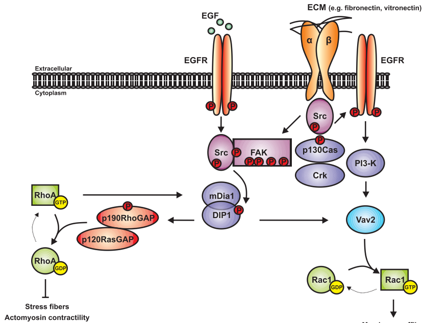
Fig. 5. Crosstalk between integrins and EGFR regulates Src activation to control Rho-GTPases. Integrins can promote Src-mediated phosphorylation of EGFR in the absence of growth factors, which occurs through a signaling complex that involves Src, p130Cas and Crk. Unengaged but activated EGFR signals through PI3K and Vav2 to promote Rac1 GTP loading. The binding of EGF to EGFR results in the direct activation of Src, which might be enhanced in the presence of integrin-FAK-Src complexes. Src activation then leads to the activation of DIP1, which in turn interacts with p190RhoGAP (leading to the inactivation of RhoA) and with Vav2 (leading to the activation of Rac1). See main text for additional details. Broken arrows indicate transition not supported by presented pathway or not supporting presented output.
