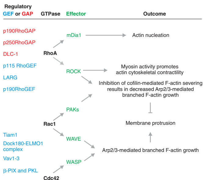
Fig. 2. Overview of Rho-GTPases, the GAPs and GEFs that regulate them and the effector pathways that act downstream of integrins. An overview of the currently known GEFs (indicated in blue) and GAPs (indicated in red) that control the activation of RhoA, Rac1 and Cdc42 downstream of integrins is shown. Through the recruitment and activation of different effector proteins (indicated in green) these Rho-GTPases regulate the actin cytoskeletal dynamics that are required for membrane protrusions and/or cytoskeletal contractility. See main text for additional details.
