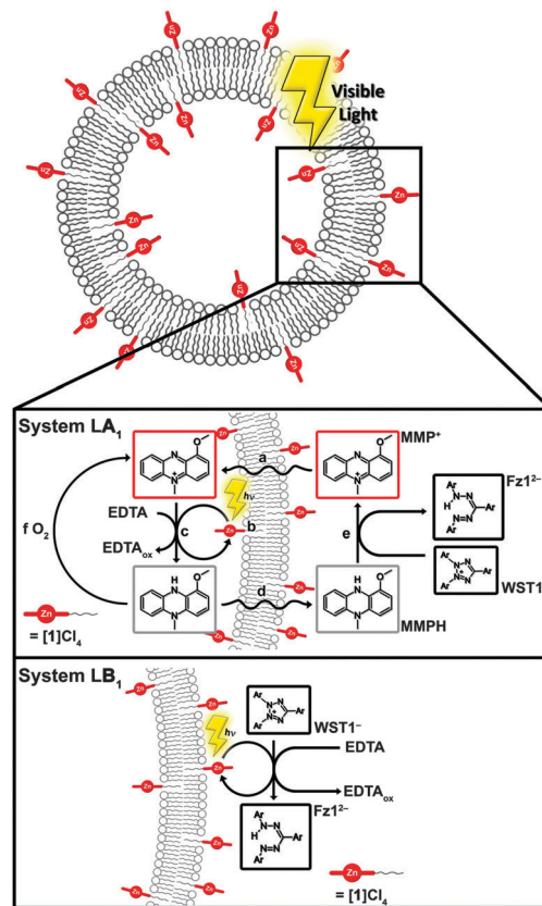
Fig. 2 Top: scheme of the photocatalytic reduction of \text{WST1}^- by \text{HEDTA}^{3-} with dye-functionalized liposomes. Middle: system LA 1 , with EDTA and \text{WST1}^- on opposite sides of the membrane. (a) Passive diffusion of \text{MMP}^+ through the membrane into the liposome. (b) Absorption of light by [\text{1}]^{4+} . (c) Photocatalytic oxidation of EDTA (in the form of \text{HEDTA}^{3-} at pH 8) and reduction of \text{MMP}^+ to \text{MMPH} . (d) Passive diffusion of \text{MMPH} through the membrane. (e) Chemical (dark) reduction of \text{WST1}^- to \text{Fz1}^{2-} by \text{MMPH} . (f) Undesired re-oxidation of \text{MMPH} to \text{MMP}^+ by molecular oxygen in system LA 4 . Bottom: system LB 1 , with \text{HEDTA}^{3-} and \text{WST1}^- on the same side of the membrane. \text{MMP}^+ has been left out for clarity as it does not influence the system significantly.
