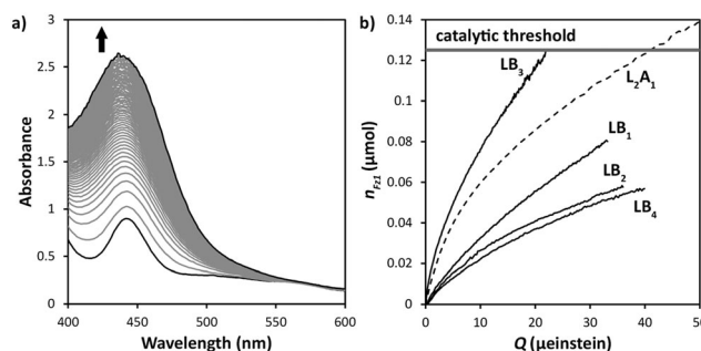
Fig. 1 (a) Evolution of the UV-vis spectrum of \text{L}_2\text{A}_1 (see Table 1) under blue light irradiation. Spectra were recorded every minute. (b) Photocatalytic formation of \text{Fz1}^{2-} ( n_{\text{Fz1}^{2-}} ) as a function of the amount of photons Q(t) absorbed by the porphyrin since t = 0 . See Table 1 for the composition of systems \text{L}_2\text{A}_1 and \text{LB}_{1-4} . Conditions: T = 298 \text{ K} , \lambda_{\text{irr}} = 449 \text{ nm} , \Delta\lambda_{1/2} = 25 \text{ nm} , photon flux \Phi = 3.3 \times 10^{-8} \text{ einstein s}^{-1} . Total irradiation time is 30 minutes, or shorter if the absorbance of the solution became higher than A = 3 at 438 nm.
