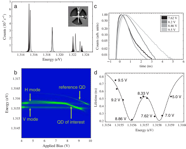
FIG. 4 (color online). (a) Microphotoluminescence spectra of nondegenerate optical modes in a micropillar. H (V) polarized modes are black (grey). Inset: SEM image of a micropillar. (b) Photoluminescence spectra as a function of applied bias for two QDs (labeled QD of interest and reference QD) and two nondegenerate fundamental cavity modes (labeled H mode and V mode). (c) Lifetime traces for a few bias settings; 7.62, 8.2, 8.86, and 9.5 V. (d) Deconvolved lifetimes as a function of emission energy with fit.
