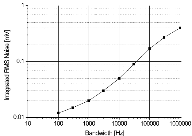
FIG. 5. Integrated rms voltage noise of the drivers with a capacitive load of 1.5 \text{ nF} .
