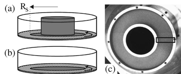
FIG. 1. (a) Schematic side-view of our split-bottomed Couette cell, showing the stationary bottom disk and inner cylinder (both gray), and the rotating bottom ring (striped) and outer cylinder. A thin layer of felt between the rings assures smooth rotation. The inner and outer cylinder radii are fixed at 65 and 105 mm, respectively, while R_s can be varied. (b) Setup in disk geometry. (c) Top view of the filled set up in the Couette geometry, where the rectangle indicates the area recorded by the video camera.
