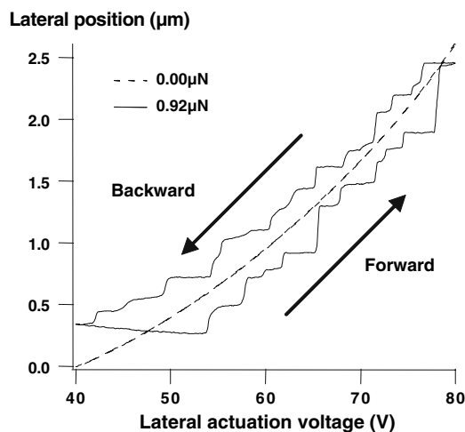
Fig. 5 Measured lateral slider position as a function of voltage on the lateral force comb drive for two settings of the normal force comb: (dashed curve) just out of contact and (solid curve) with 0.92 \mu\text{N} of normal force on the contact
