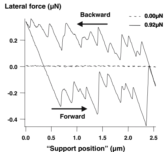
Fig. 6 High-resolution MEMS friction loops constructed using the measurements of Fig. 5: (dashed curve) just out of contact and (solid curve) with 0.92 \mu\text{N} of normal force on the contact. The area enclosed by the loop is the energy dissipated by the friction process during one forward-reverse cycle
