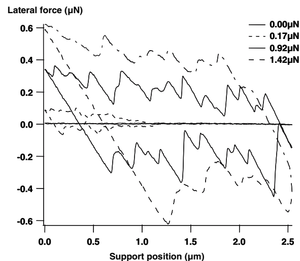
Fig. 7 Friction loops obtained by the Leiden MEMS Tribometer at different normal loads, starting with a pristine device and measured from lower to higher loads
