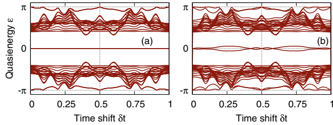
FIG. 2. (Color online) Effect of breaking CS by time shifting the pulse of the intracell hopping v(t) with respect to the other pulses. (a) In the PDSSH model, the extra PHS protects the end states at \epsilon = 0 . (b) In the PDRM model, there is no PHS, and all end-state energies are affected by the time shift.
