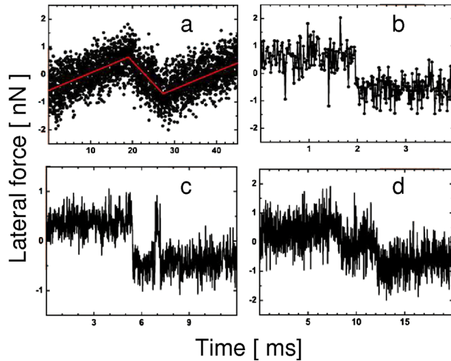
FIG. 3 (color online). Examples of experimentally observed slip events (reproduced from Ref. [9]). Compare panel (a) with Fig. 1(h), (b) with Figs. 1(d) and 1(l), (c) with Figs. 1(e) and 1(k), and (d) with Fig. 1(i).
