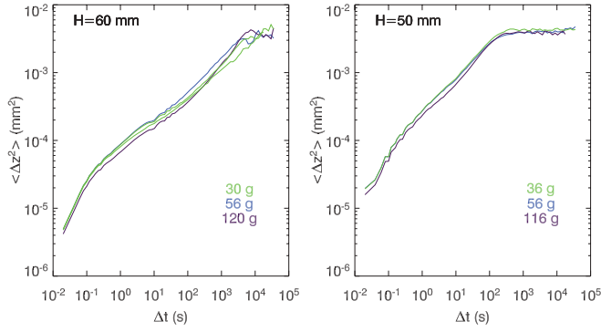
FIG. 13. (Color online) Left panel: \langle(\Delta z)^2\rangle for H = 60 mm, R = 25 mm, and M = 30 g, M = 56 g, and M = 120 g overlap. Right panel: \langle(\Delta z)^2\rangle for H = 50 mm, R = 25 mm, and M = 36 g, M = 56 g, and M = 116 g overlap.
