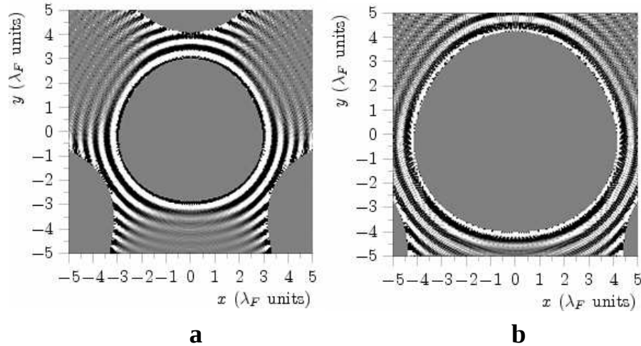
FIG. 5: Same as Fig. 3, but for a (111) interface plane. The x and y directions correspond to [11\bar{2}] and [\bar{1}10] directions respectively.
