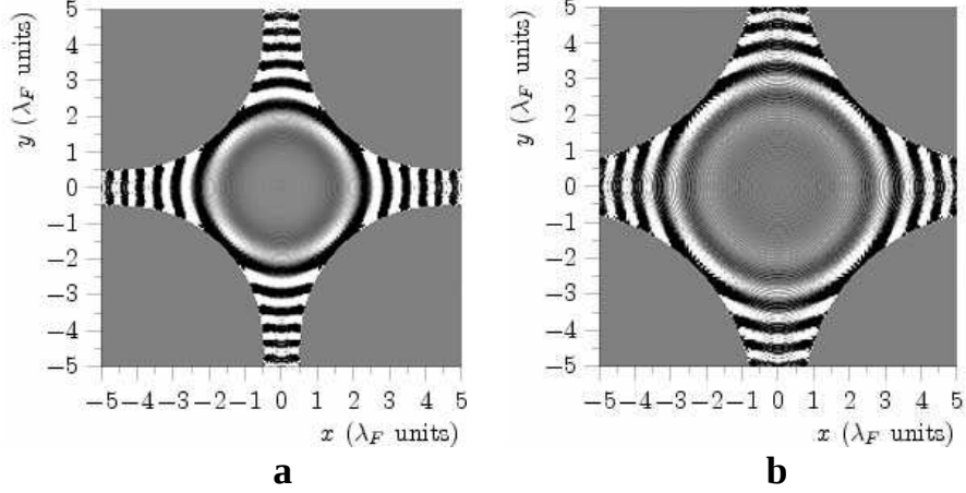
FIG. 3: Conductance G as a function of the contact position for a defect at the origin at depths 5\lambda_F (a) and 7\lambda_F (b) for a (100) interface plane. The x and y directions both correspond to \langle 100 \rangle directions. The conductance is plotted in gray scale, where the color of the 'dead' regions corresponds to the conductance value in absence the defect G = G_0 , positive addition to G is white and negative is black.
