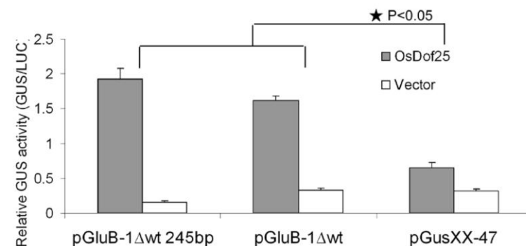
Figure 1. Activation of the GluB-1 promoter by OsDof24 and OsDof25.
