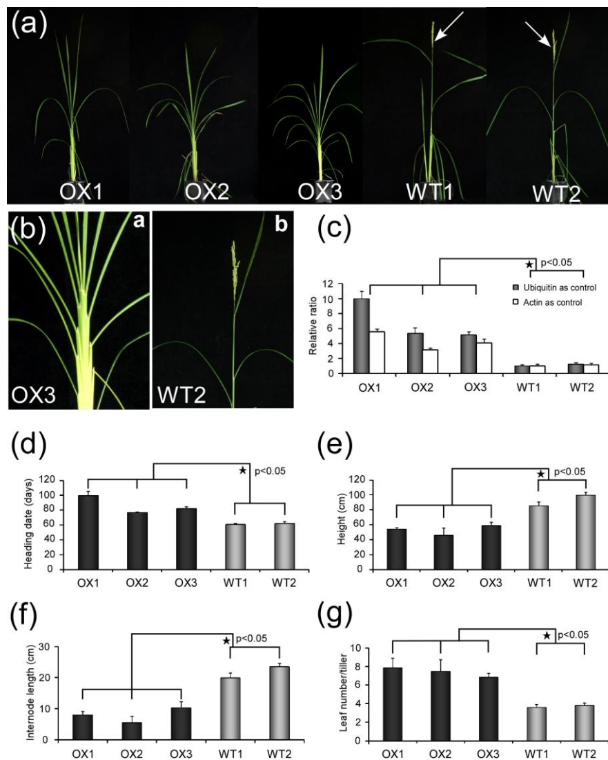
Figure 2. Phenotypal characterization and expression levels of OsDof24 in overexpression plants and control lines.
