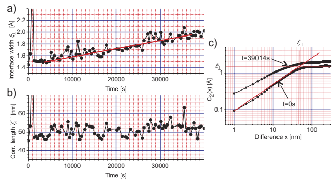
FIG. 2 (color online). Correlation values during film growth: (a) interface width \xi_{\perp} , (b) parallel correlation length \xi_{\parallel} , and (c) two examples of the height-difference correlation function; from the kink position we determine \xi_{\perp} and \xi_{\parallel} .
