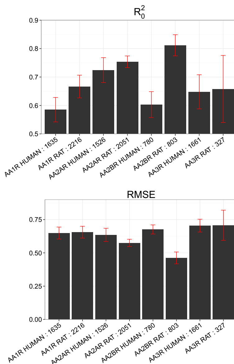
Figure 5 Model performance per target on the external set for the adenosine receptors dataset. The upper panel corresponds to R_0^2 , while the lower panel to RMSE ext . These values were averaged for ten models trained on each subset corresponding to a given target. The best modeled target is the rat adenosine A_{2b} receptor (AA2BR RAT), while the worst is the rat A_3 receptor (AA3R RAT). In all cases, the mean RMSE ext values are below 0.75 pK_i units, indicating that GP modeling can predict compounds bioactivities on subsets corresponding to a given target.
