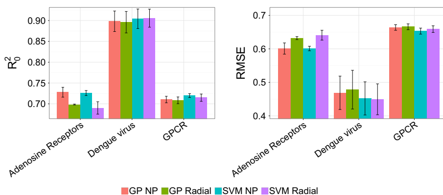
Figure 1 Comparison between the performance of GP and SVM with either the radial or the normalized polynomial (NP) kernel. Ten models were calculated for each dataset and for each combination of modeling technique and kernel, thus resulting in a total of 60 models. The performance of GP and SVM was assessed by kernel for the three datasets. Given that the distributions of \text{RMSEP}_{\text{ext}} and R_{0\text{ ext}}^2 values were normally distributed, a two-tailed t -test of independent samples was applied to statistically evaluate their differences. These analyses let us conclude that SVM and GP perform on par for the modeling of the three datasets considered in this study.
