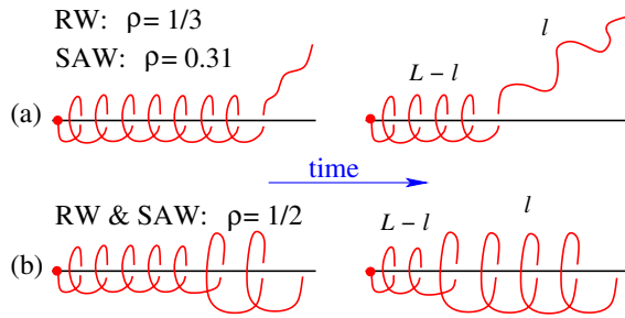
FIG. 5 (color online). Two possible configurations of polymers during unwinding. (a) A tight helix of length L - l connected to a loose equilibrated end of length l . (b) The part of the polymer detached from the bar here still has some winding. The exponents \rho governing the early-time decay of the winding angle predicted in the two cases are given.
