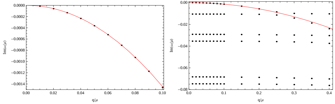
Figure 2: Dispersion relations of the purely imaginary ‘poles’ nearest the origin as determined by Leaver’s method, at fixed N_{\text{max}} = 300 (shown as dots). The red line shows the analytic result (55) for the T = 0 diffusion mode. The data on both plots is the same – the left hand plot is a magnified version of the near-origin region of the right hand plot.
