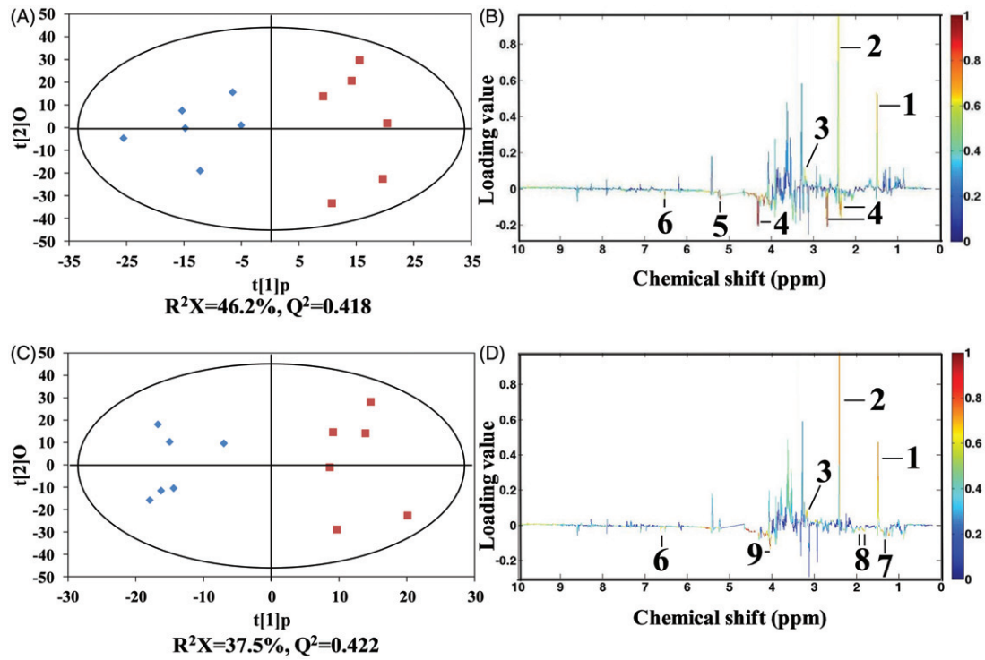
Figure 6. O-PLS-DA score plots derived from ^1H NMR spectra of tissue extracts from earthworms E. fetida exposed to controls (◆) and 1\text{ mg L}^{-1} small (10 nm) AgNPs (■) (A), and control (◆) and Ag^+ released from small AgNPs (■) (C) for 96 h, and corresponding coefficient plots (B) and (D). The color map shows the significance of metabolite variations between the two classes (control and treatment). Peaks in the positive direction indicate metabolites that were more abundant in the treatments, metabolites that were more abundant in the control are presented as peaks in the negative direction. Metabolites were assigned and labeled in Figure S2. Keys: (1) alanine, (2) succinate, (3) phosphocholine, (4) malate, (5) \alpha -glucose, (6) fumarate, (7) threonine, (8) arginine and (9) myo-inositol.
