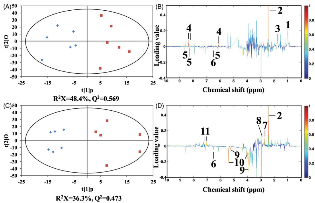
Figure 7. O-PLS-DA score plots derived from ^1H NMR spectra of tissue extracts from earthworm E. fetida exposed to control (◆) and 1\text{ mg L}^{-1} large (40 nm) silver nanoparticle treatment (■) (A), and control (◆) and the released Ag^+ treatment from large silver nanoparticle (■) (C) for 96 h, and corresponding coefficient plots (B) and (D). The color map shows the significance of metabolite variations between the two classes (control and treatment). Peaks in the positive direction indicate metabolites that are more abundant in the treatments. Consequently, metabolites that are more abundant in the control group are presented as peaks in the negative direction. Metabolites were assigned and labeled in Figure S2. Keys: (1) leucine, (2) succinate, (3) arginine, (4) inosine, (5) ATP, (6) fumarate, (7) aspartate, (8) asparagine, (9) \alpha -glucose, (10) maltose and (11) phenylalanine.
