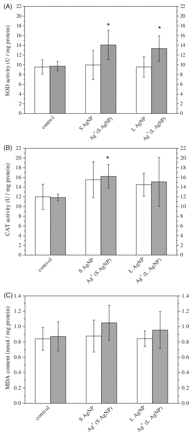
Figure 5. SOD (A), CAT (B) activities and MDA (C) content in the earthworm E. fetida after 96h exposure of 1 mg L -1 two sizes of PVP-capped AgNP and the corresponding released Ag + . The smaller AgNPs (named S AgNP) and larger AgNPs (L AgNP) had an average size of 10 and 40 nm, respectively. The two groups of released Ag + exposures from the small and large AgNPs are referred as Ag + (S AgNP) and Ag + (L AgNP), respectively. Error bars represent the standard deviation of the mean of three replicates. Significantly different from the control: * p<0.05 .
