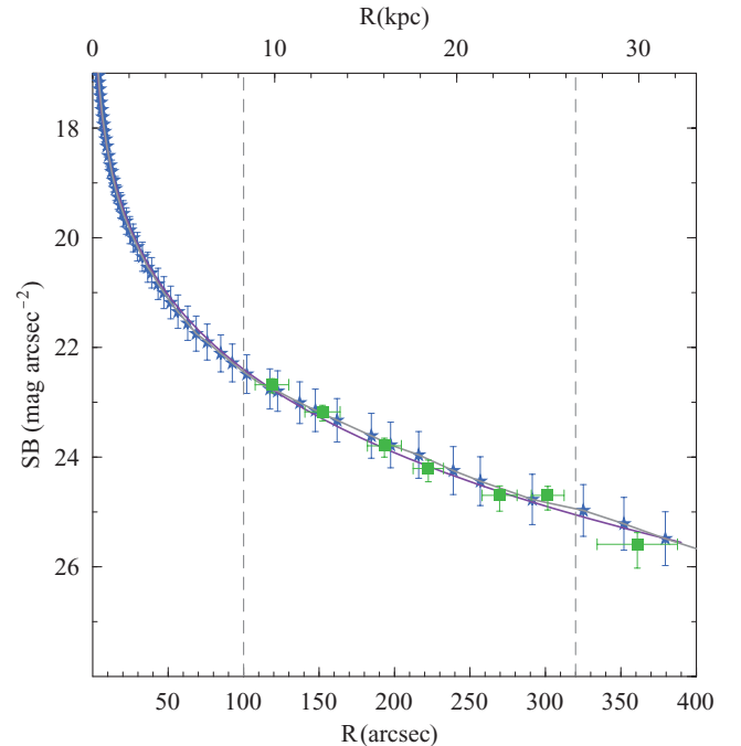
Figure 2. Radial surface density profiles of the field stars (V band; blue star symbols) and of the PNe (green squares) in NGC 4374. The PN number counts have been corrected for spatial incompleteness, and arbitrarily normalized to match the stellar data. The vertical error bars of the PN data in this and in the following figures represent the 1\sigma uncertainties (based in this case on counting statistics and completeness correction uncertainties), while the horizontal error bars show 68 per cent of the radial range of the PNe in each bin. The purple curve is a Sérsic model fit to the stellar photometry, and the grey solid curve is the interpolating profile. The vertical dashed lines show the spatial completeness interval of the PN system.
