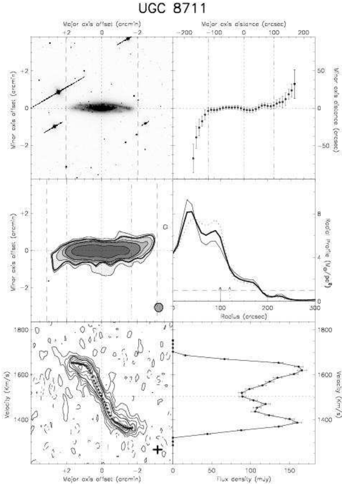
Fig. A.13. – continued. UGC 8711: This galaxy is isolated and exhibits quite a large warp. The warp can not be mistaken for inclined spiral arms because these run in the opposite directions. For this galaxy the lowest contour in the total HI map is 3.2 \cdot 10^{20} HI atoms/cm 2 , and in the XV diagram 3\sigma = 9.59 K.
