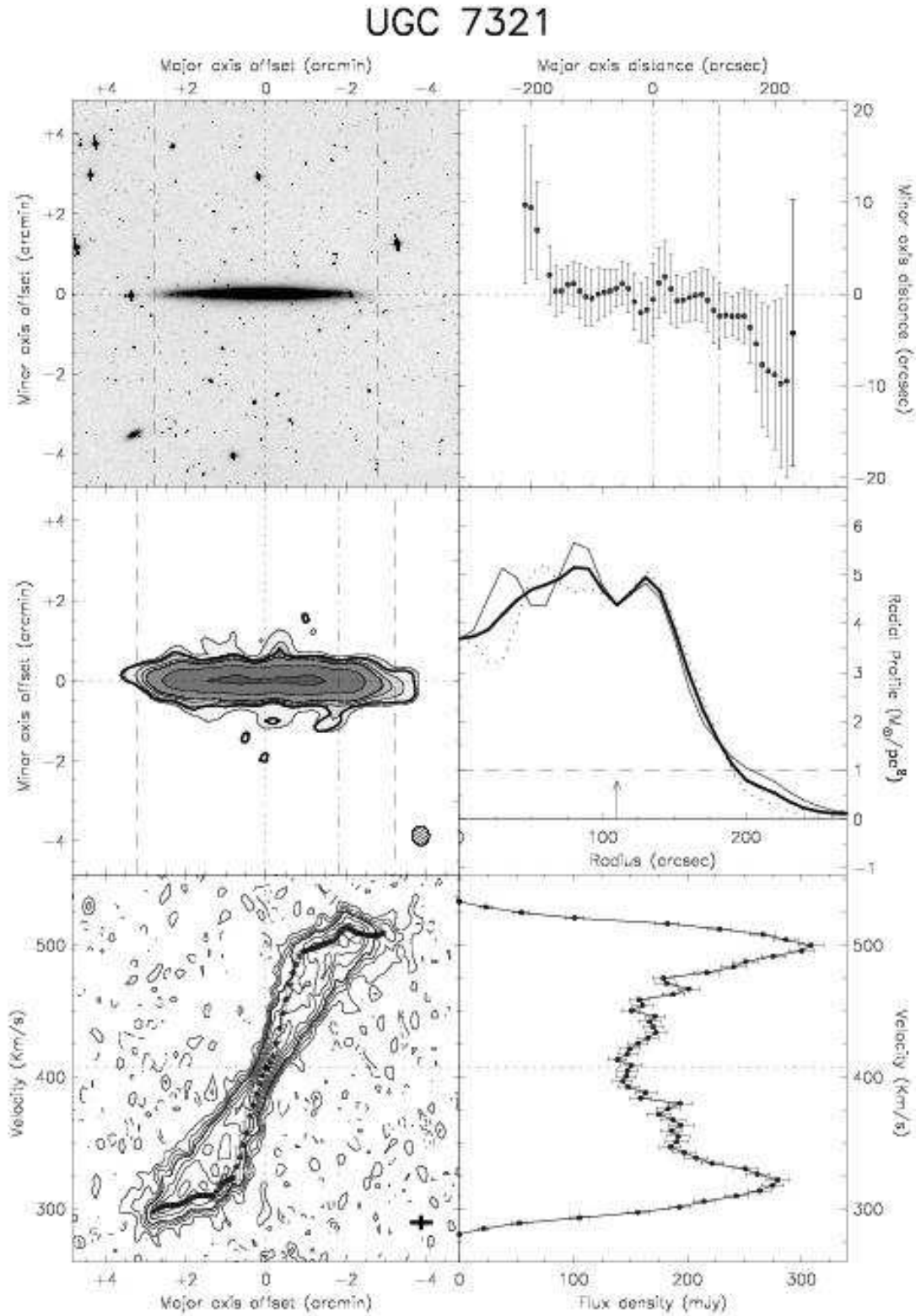
Fig. A.13. – continued. UGC 7321: This galaxy ultrathin (Goad & Roberts, 1981). There is a mild warp visible on the receding side. This places some constraints on the possible formation scenarios for the warp of this galaxy because some of the processes that generate warps do also heat up the disk. For this galaxy the lowest contour in the total HI map is 2.4 \cdot 10^{20} HI atoms/cm 2 , and in the XV diagram 3\sigma = 8.58 K.
