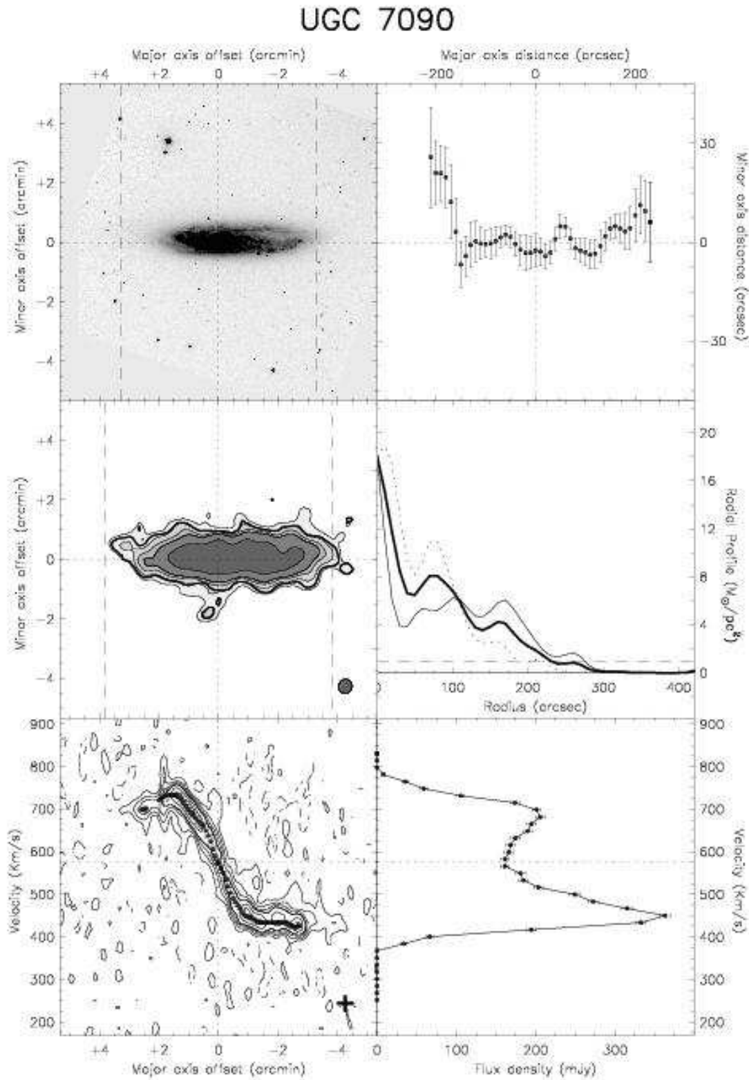
Fig. A.13. – continued. UGC 7090: This galaxy has very strong kinematical and density lopsidedness indices and a very asymmetric global profile. For this galaxy the lowest contour in the total HI map is 3 \cdot 10^{20} HI atoms/cm 2 , and in the XV diagram 3\sigma = 7.97 K.
