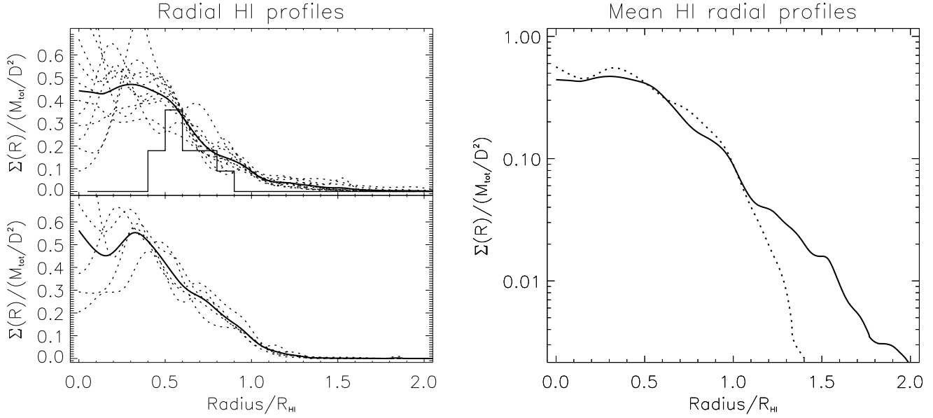
Fig. 9. Radial HI density profiles. The plot on the left shows the HI profiles for bona fide warped (upper panel) and non-warped (lower panel) galaxies (see Sect. 5.5 for definition of both groups). The profiles of individual warped and non warped galaxies are plotted in dotted line, and the thick line is the average profile for each group. In the upper panel a histogram of the radius where the warp begins is overplotted. We have treated both sides of the galaxy independently, to take into account that two of our bona fide warped galaxies have only one-sided warps. The plot on the right shows the mean profiles for both bona fide warped (solid line) and non warped galaxies (dotted line).
