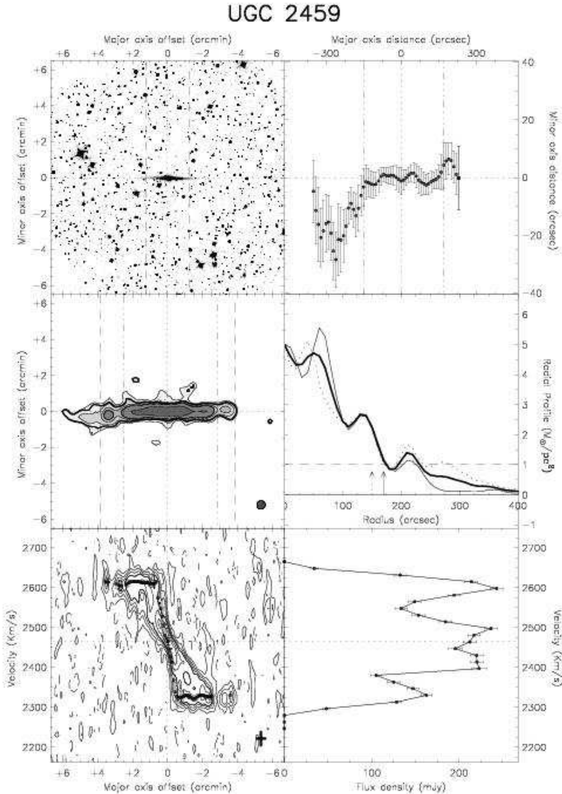
Fig. A.13. – continued. UGC 2459: This galaxy is located at very low galactic latitude ( -8.6^{\circ} ) and the optical image is highly affected by interstellar extinction. The total HI map shows evidence for spiral arms around R_{HI} and just before that the disk warps on both sides. The distribution of HI is asymmetric: the right side warp is very small, while on the left side the disk bends downwards and then turns back towards the plane of the inner disk as in the Galaxy. For this galaxy the lowest contour in the total HI map is 3 \cdot 10^{20} HI atoms/cm 2 , and in the XV diagram 3\sigma = 8.53 K.
