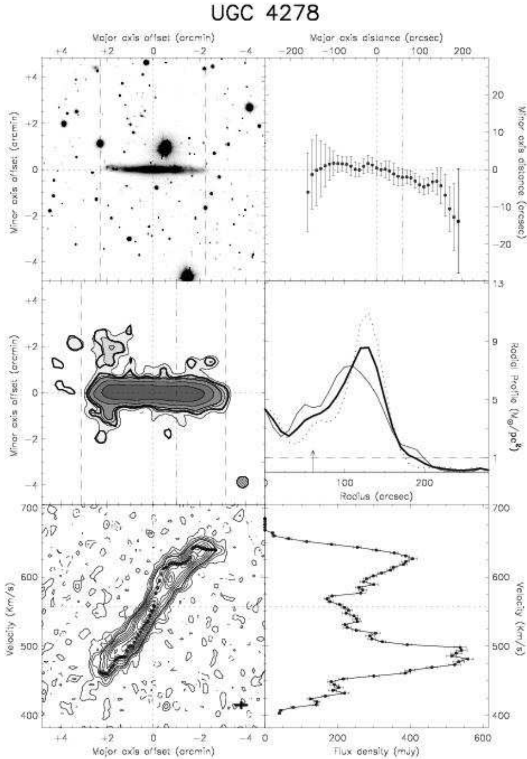
Fig. A.13. – continued. UGC 4278: The main disk of this galaxy is surrounded by some faint clouds on the left side. The galaxy is also kinematically lopsided. For this galaxy the lowest contour in the total HI map is 1.6 \cdot 10^{20} HI atoms/cm 2 , and in the XV diagram 3\sigma = 12.8 K.
