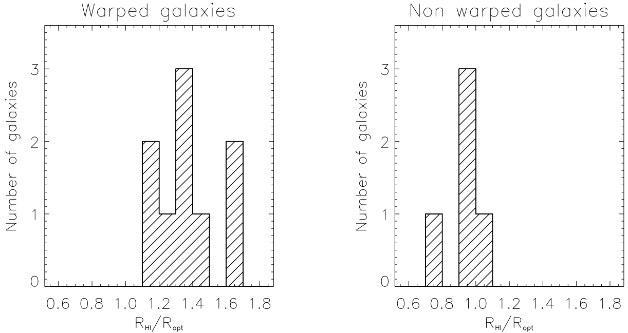
Fig. 10. Histograms of the ratio R_{\text{HI}} to R_{\text{opt}} for bona fide warped (left panel) and non-warped (right panel) galaxies (see Sect. 5.5 for definition of both groups). The histograms show that warped galaxies are more extended in HI than the non warped ones.
