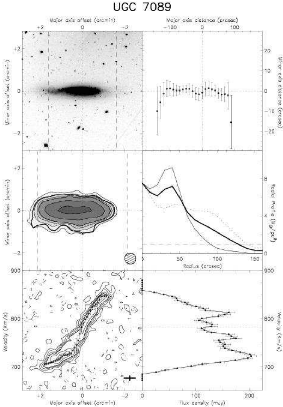
Fig. A.13. – continued. UGC 7089: This galaxy is very lopsided both in the optical and the HI distribution. The HI does not extend further than the optical. For this galaxy the lowest contour in the total HI map is 1.4 \cdot 10^{20} HI atoms/cm 2 , and in the XV diagram 3\sigma = 14 K.
