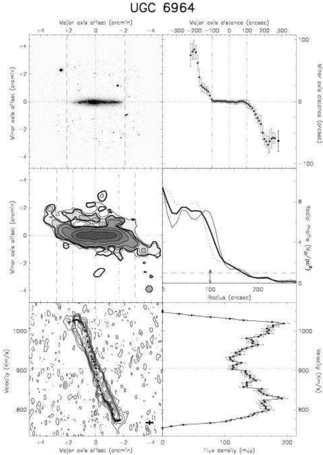
Fig. A.13. – continued. UGC 6964: This galaxy shows quite a large and symmetric warp. Note the lopsided optical image. The XV diagram shows a “bump” very close to the center and a closer inspection of the datacube suggests that this could be the signature of infalling (or outflowing) gas onto the disk. That feature is kinematically connected to the extra HI gas at the top-right part of the disk. For this galaxy the lowest contour in the total HI map is 9.2 \cdot 10^{19} HI atoms/cm 2 , and in the XV diagram 3\sigma = 19.7 K.
