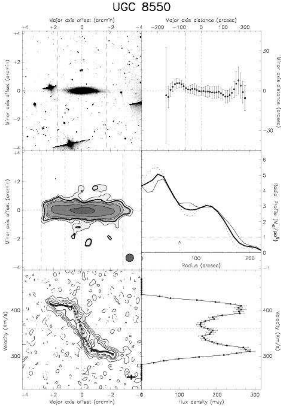
Fig. A.13. – continued. UGC 8550: The disk of this galaxy looks somewhat peculiar both in the optical and the HI. The optical image shows a faint extension of the disk misaligned with the inner isophotes, probably due to non edge-on spiral arms. For this galaxy the lowest contour in the total HI map is 1.4 \cdot 10^{20} HI atoms/cm 2 , and in the XV diagram 3\sigma = 16.8 K.
