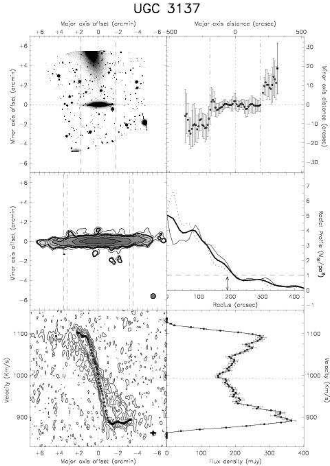
Fig. A.13. – continued. UGC 3137: This galaxy has a low level, very symmetric warp that bends suddenly and then stays at a fixed height, resembling a step. For this galaxy the lowest contour in the total HI map is 1.6 \cdot 10^{20} HI atoms/cm 2 , and in the XV diagram 3\sigma = 18.9 K.
