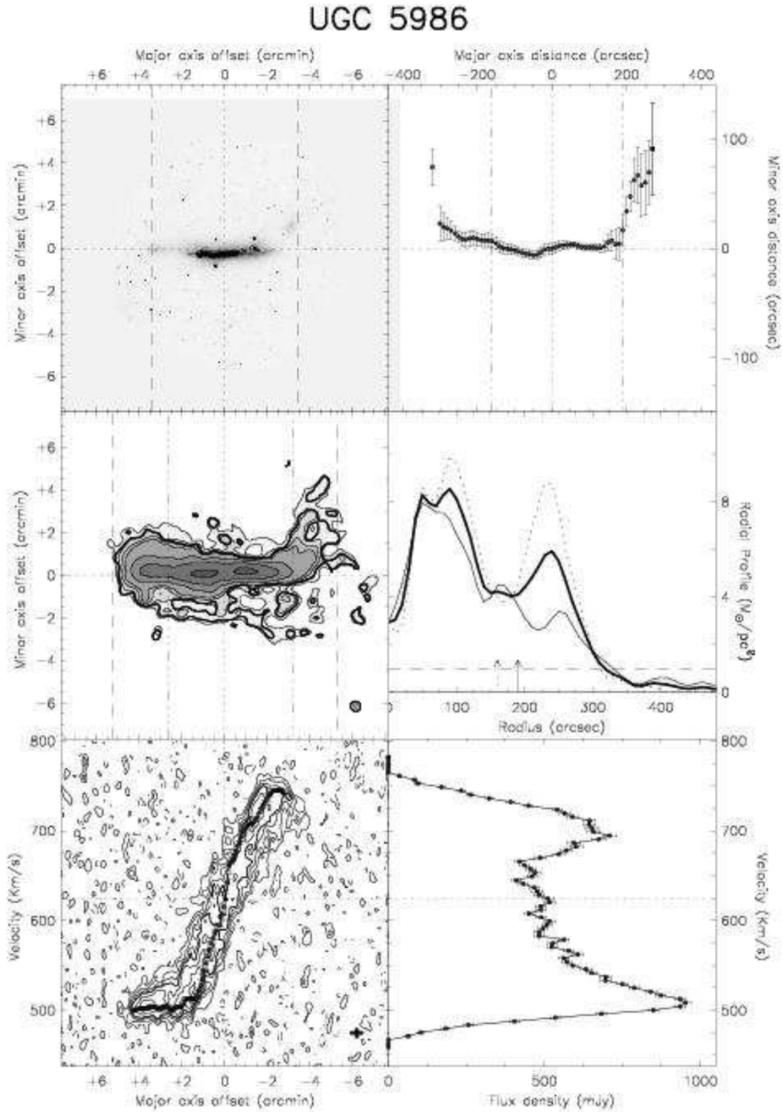
Fig. A.13. – continued. UGC 5986: This galaxy shows major distortions both morphologically and kinematically. The galaxy UGC 5983 (only 3.5' away) is likely to be responsible for some of these distortions. The central part of the galaxy shows non-circular motions of the gas. For this galaxy the lowest contour in the total HI map is 2 \cdot 10^{20} HI atoms/cm 2 , and in the XV diagram 3\sigma = 15.7 K.
