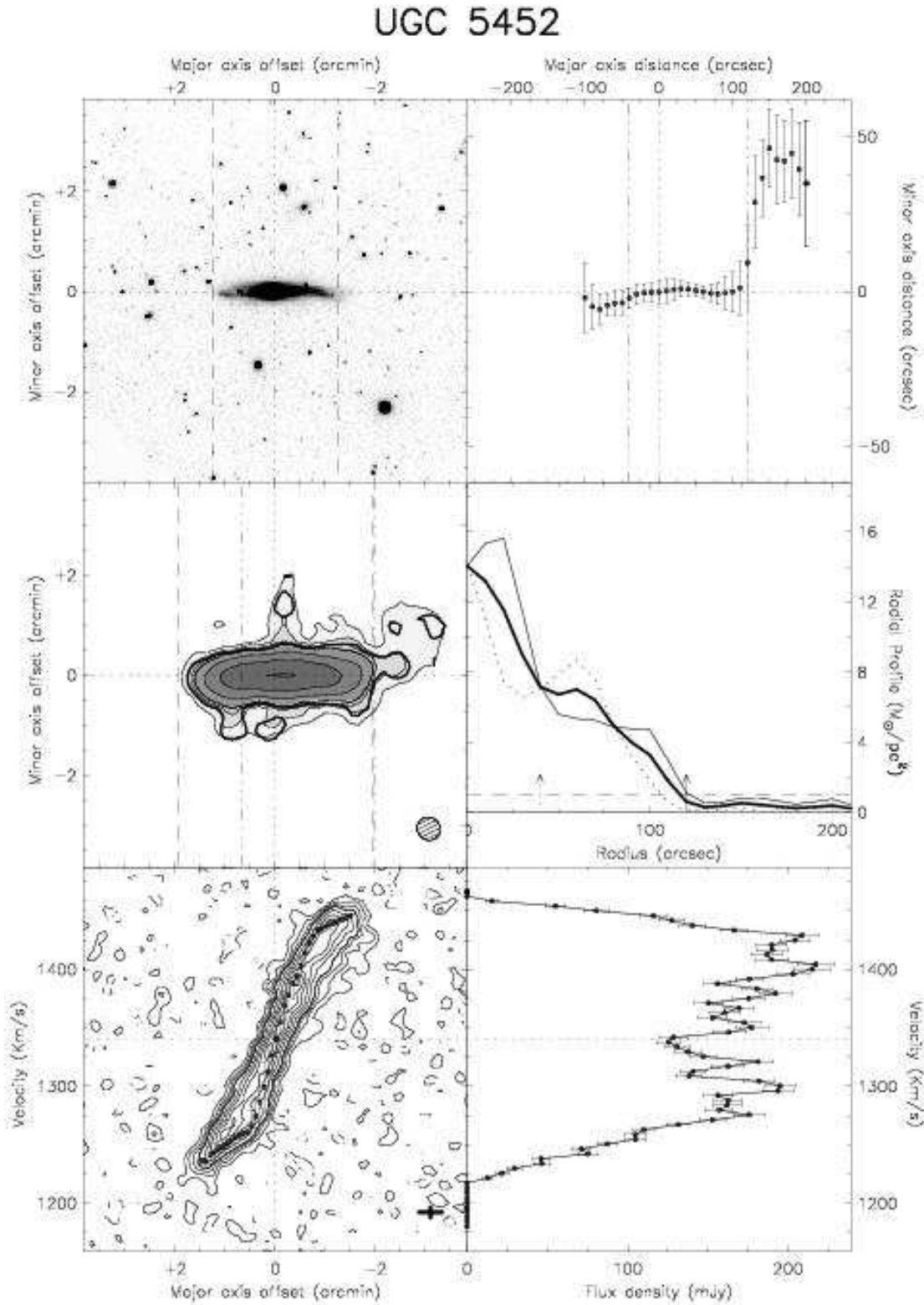
Fig. A.13. – continued. UGC 5452: The emission in the region of the warp (right side, see total HI map) is very faint and barely detected. The one-sided warp of this galaxy pointing towards the galaxy UGC 5446 suggests a tidal origin for it. The optical image seems to bend in the opposite direction to that of the HI warp in the right side. For this galaxy the lowest contour in the total HI map is 1.4 \cdot 10^{20} HI atoms/cm 2 , and in the XV diagram 3\sigma = 9.29 K.
