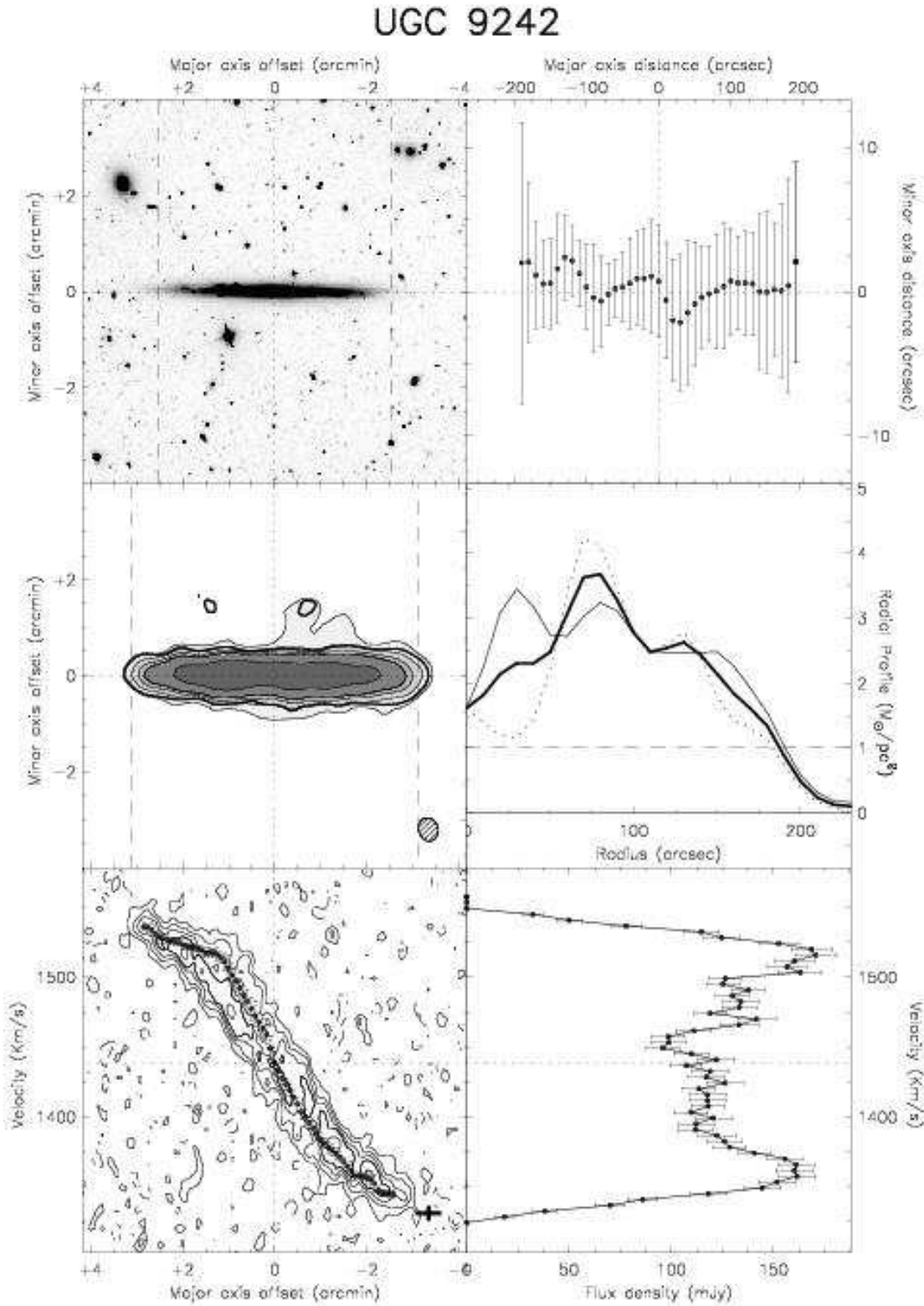
Fig. A.13. – continued. UGC 9242: This is another ultrathin galaxy. It is the flattest of the galaxies in our sample, with deviations smaller than 2.5'' over the 400'' diameter of the galaxy. There is evidence of non-circular motions in the central regions. For this galaxy the lowest contour in the total HI map is 1.9 \cdot 10^{20} HI atoms/cm 2 , and in the XV diagram 3\sigma = 20 K.
