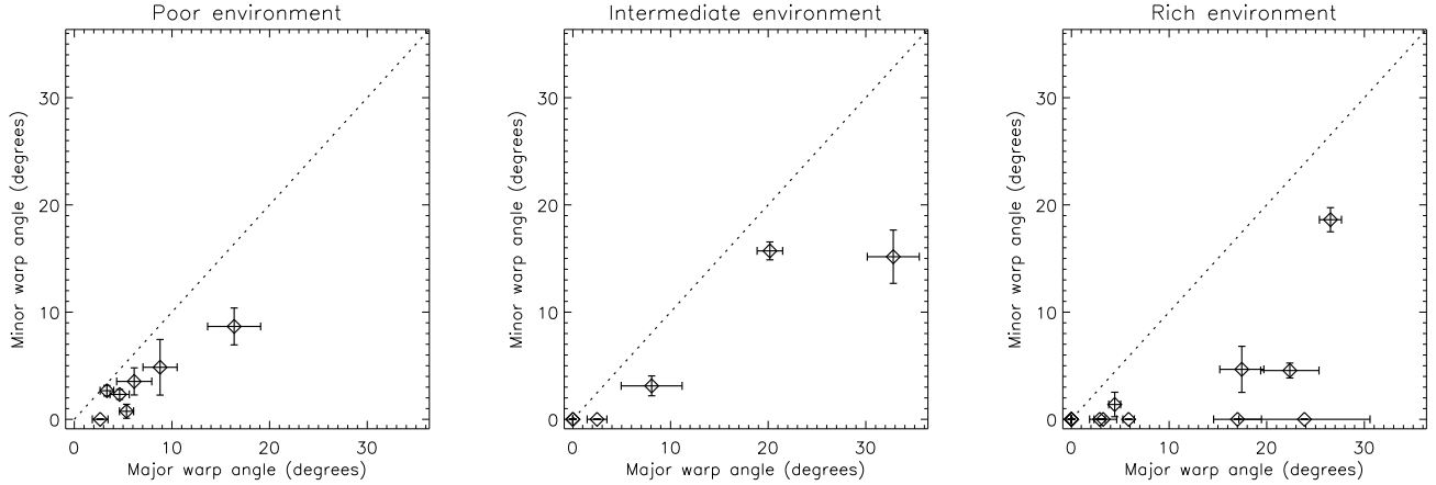
Fig. 8. Warp angles for each environment class (see definition in Sect. 4.8). The left panel shows the warps of galaxies in poor environments, the middle panel the galaxies in intermediate environments, and the right panel those in rich environments. For each galaxy, the larger of both side’s warp angles has been plotted on the x axis, versus the smaller one on the y axis (so the upper left part of the plots is empty). The galaxies with a detected warp on only one side lie in the y=0 line, and the non warped galaxies are in the origin. The dotted line indicates equal warp angles on both sides of the galaxy.
