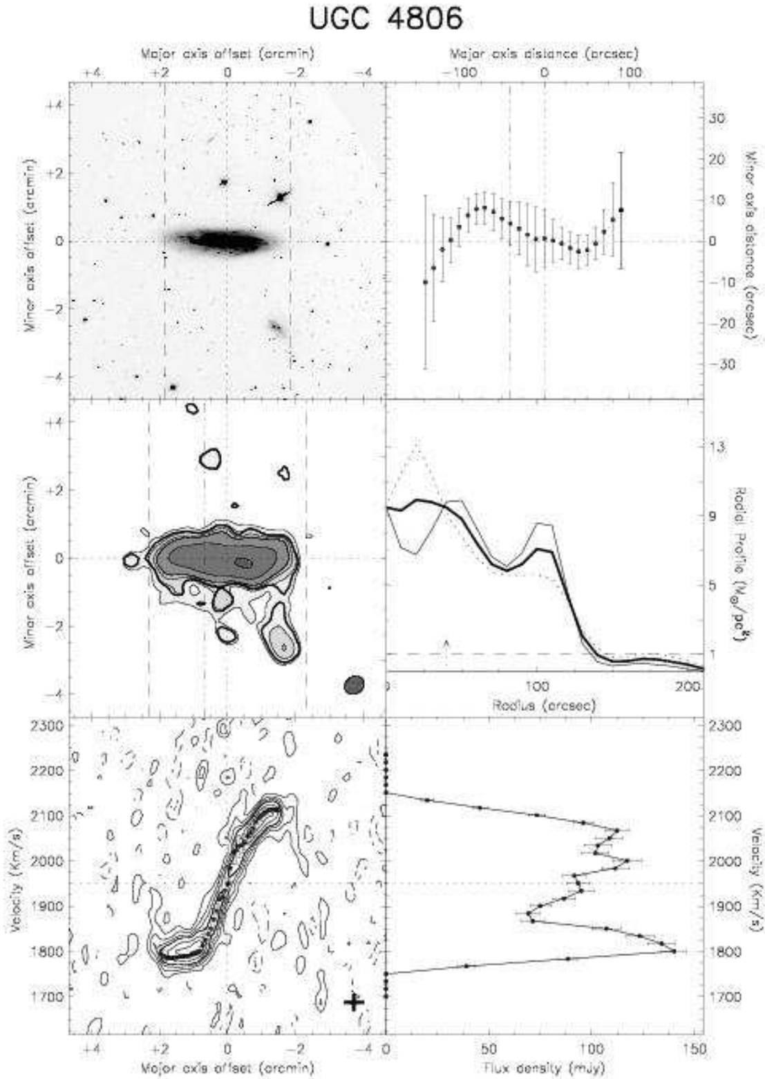
Fig. A.13. – continued. UGC 4806: We detected three galaxies in HI within a radius of 12' around this galaxy. The HI disk is only slightly larger than the optical and shows no warp. For this galaxy the lowest contour in the total HI map is 2.2 \cdot 10^{20} HI atoms/cm 2 , and in the XV diagram 3\sigma = 6.42 K.
