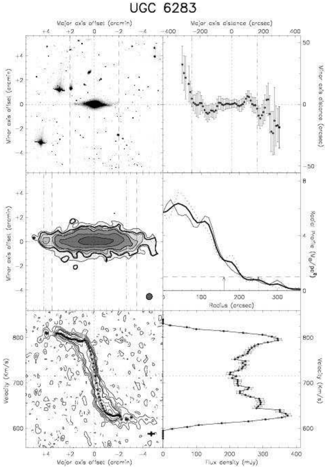
Fig. A.13. – continued. UGC 6283: This galaxy is the earliest type galaxy (Sab) of our sample and has a very prominent bulge. This inner bulge is inclined with respect to the plane defined by the HI disk by \simeq 3^\circ . The optical image also shows a faint disk component aligned with the HI disk (probably the warp detected in Sánchez-Saavedra et al. (1990)). For this galaxy the lowest contour in the total HI map is 1.6 \cdot 10^{20} HI atoms/cm 2 , and in the XV diagram 3\sigma = 13.1 K.
