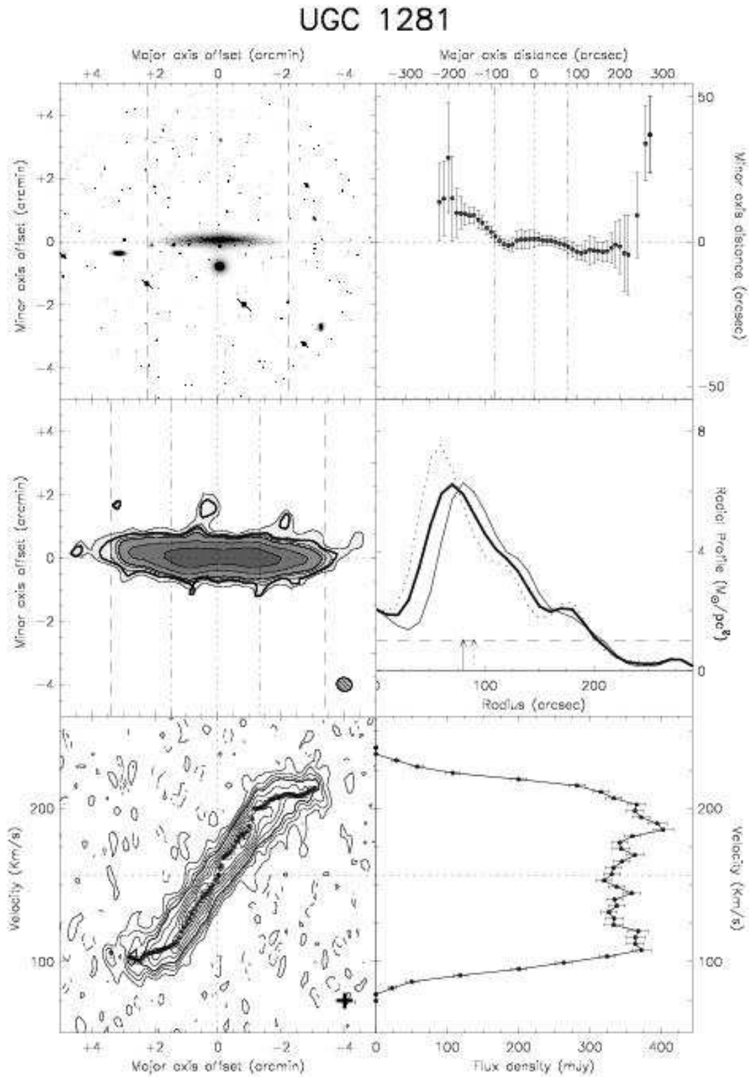
Fig. A.13. – continued. UGC 1281: The warp is visible in the extreme velocity channels on both sides of the disk. For this galaxy the lowest contour in the total HI map is 1.5 \cdot 10^{20} HI atoms/cm 2 , and in the XV diagram 3\sigma = 13.4 K.
