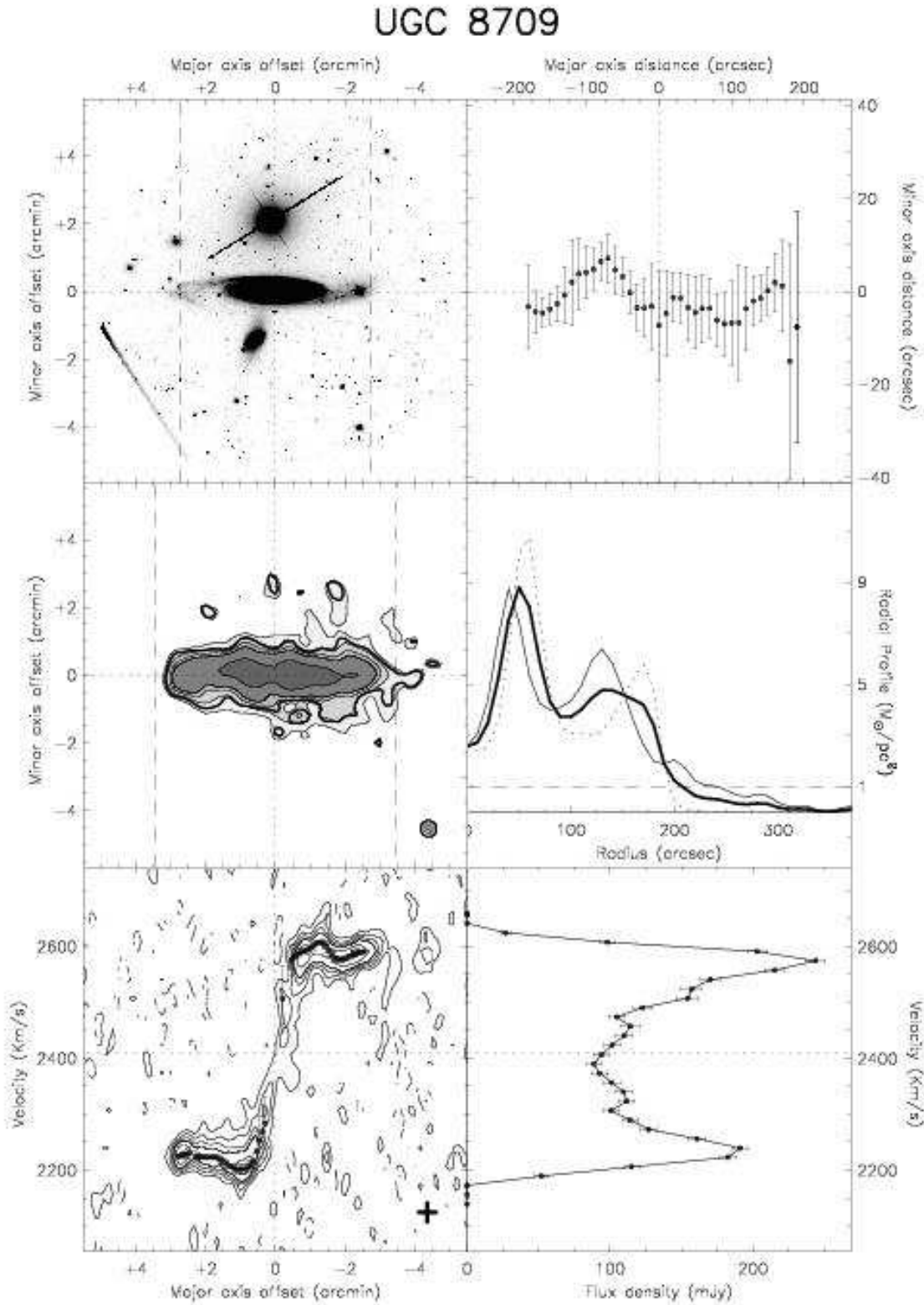
Fig. A.13. – continued. UGC 8709: This galaxy is not completely edge-on and two spiral arms are clearly visible on the optical picture. Even though it has a very close companion galaxy (NGC 5296), it has no warp. For this galaxy the lowest contour in the total HI map is 2.8 \cdot 10^{20} HI atoms/cm 2 , and in the XV diagram 3\sigma = 7.67 K.
