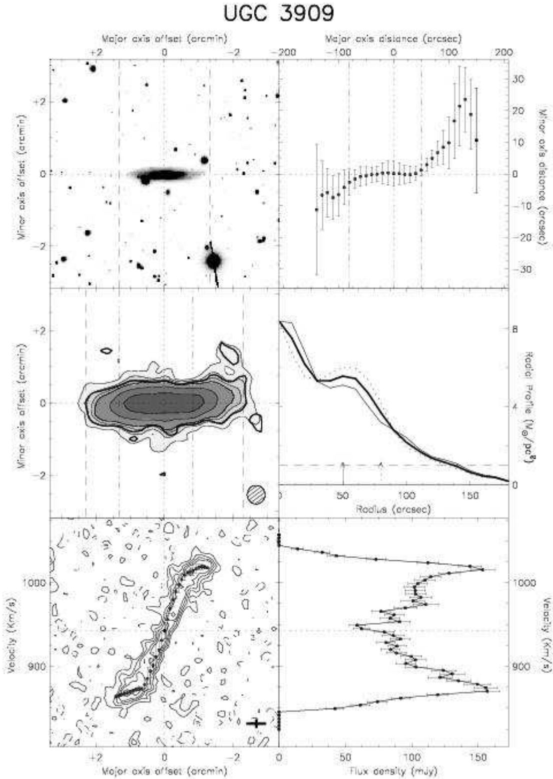
Fig. A.13. – continued. UGC 3909: The optical disk seems to warp in the same sense as the HI. For this galaxy the lowest contour in the total HI map is 1.2 \cdot 10^{20} HI atoms/cm 2 , and in the XV diagram 3\sigma = 21.7 K.
