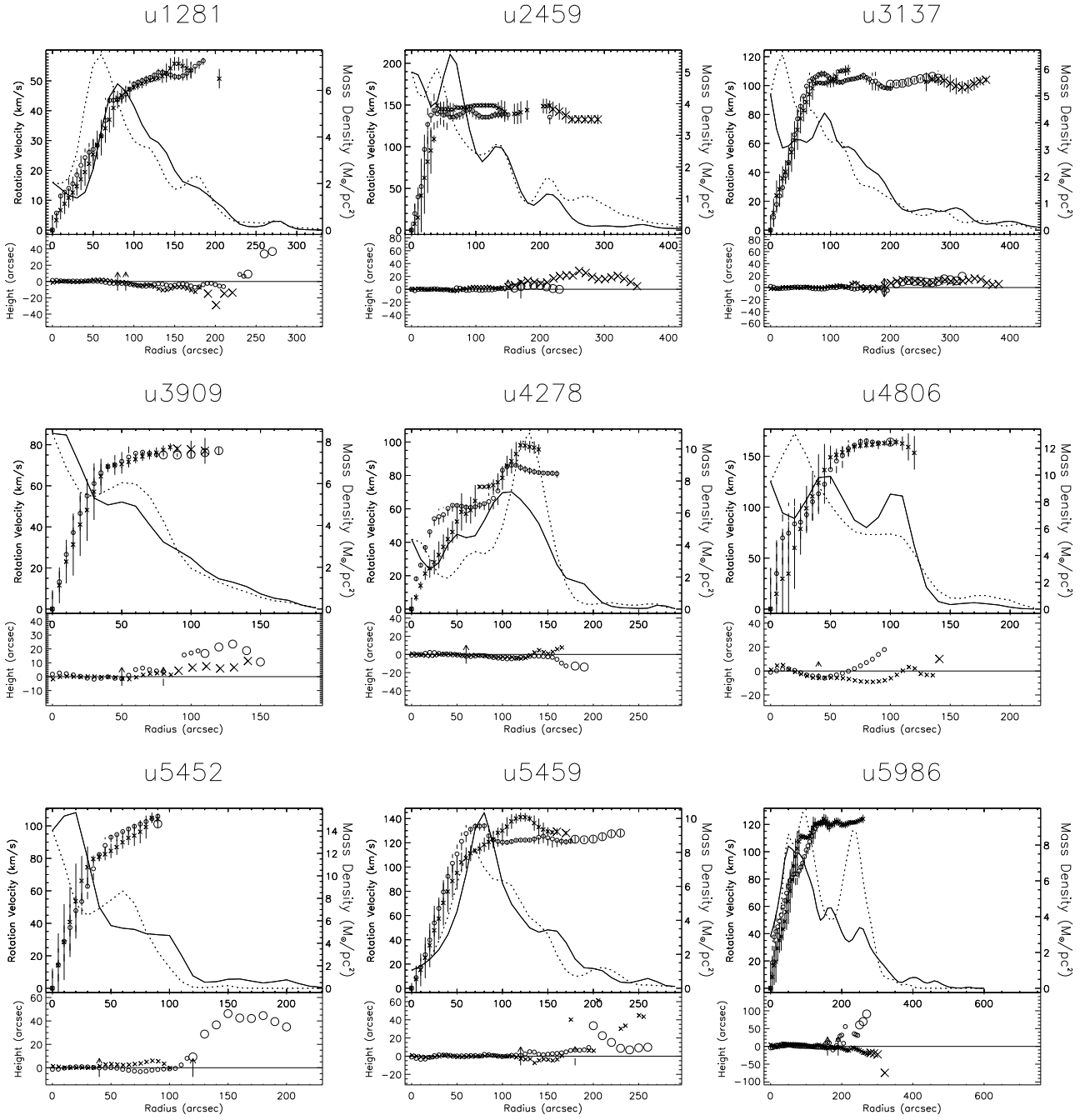
Fig. 7. Density - RC - warp plots. For each galaxy, the rotation curve along the major axis, the radial HI density profile and the curve of warp are plotted. We have measured these quantities independently for both sides of the galaxies, and here we present them together in the same plot. The top panel shows the rotation velocities and radial density profiles for both sides of the galaxy. The left axis shows the units for the rotation velocities, while the right axis applies to the density profiles. The bottom panel shows the warp curves for both sides. Because most of the warps have an S-shape, the warp curve derived for the left side has been inverted, to highlight symmetries or asymmetries between the two sides of the galaxy. With this process, both warp curves of a galaxy with a perfect S-shape symmetry (thus, antisymmetry) would fall on top of each other. One side is plotted with crosses (rotation curve and warp curve) and dotted line (density), and the other side is plotted with circles (rotation curve and warp curve) and solid line (density). The rotation curve and warp curves in the figure are shown at 2 different resolutions. We derived these curves using the full resolution data (small symbols), and then complemented it in the outer parts with the curves obtained at 30'' resolution (bigger symbols). Errorbars have not been plotted in the warp curves for sake of clarity, they are shown in Figure 13.
