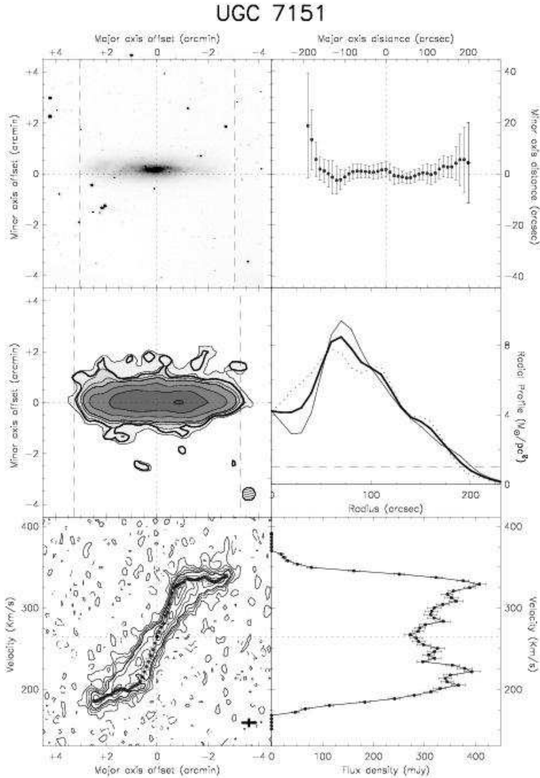
Fig. A.13. – continued. UGC 7151: The HI is confined to the extent of the optical disk in this galaxy. The rotation curve reaches a flat part on the receding side but rises continuously until the last measured point on the approaching side. For this galaxy the lowest contour in the total HI map is 1.4 \cdot 10^{20} HI atoms/cm 2 , and in the XV diagram 3\sigma = 14.5 K.
