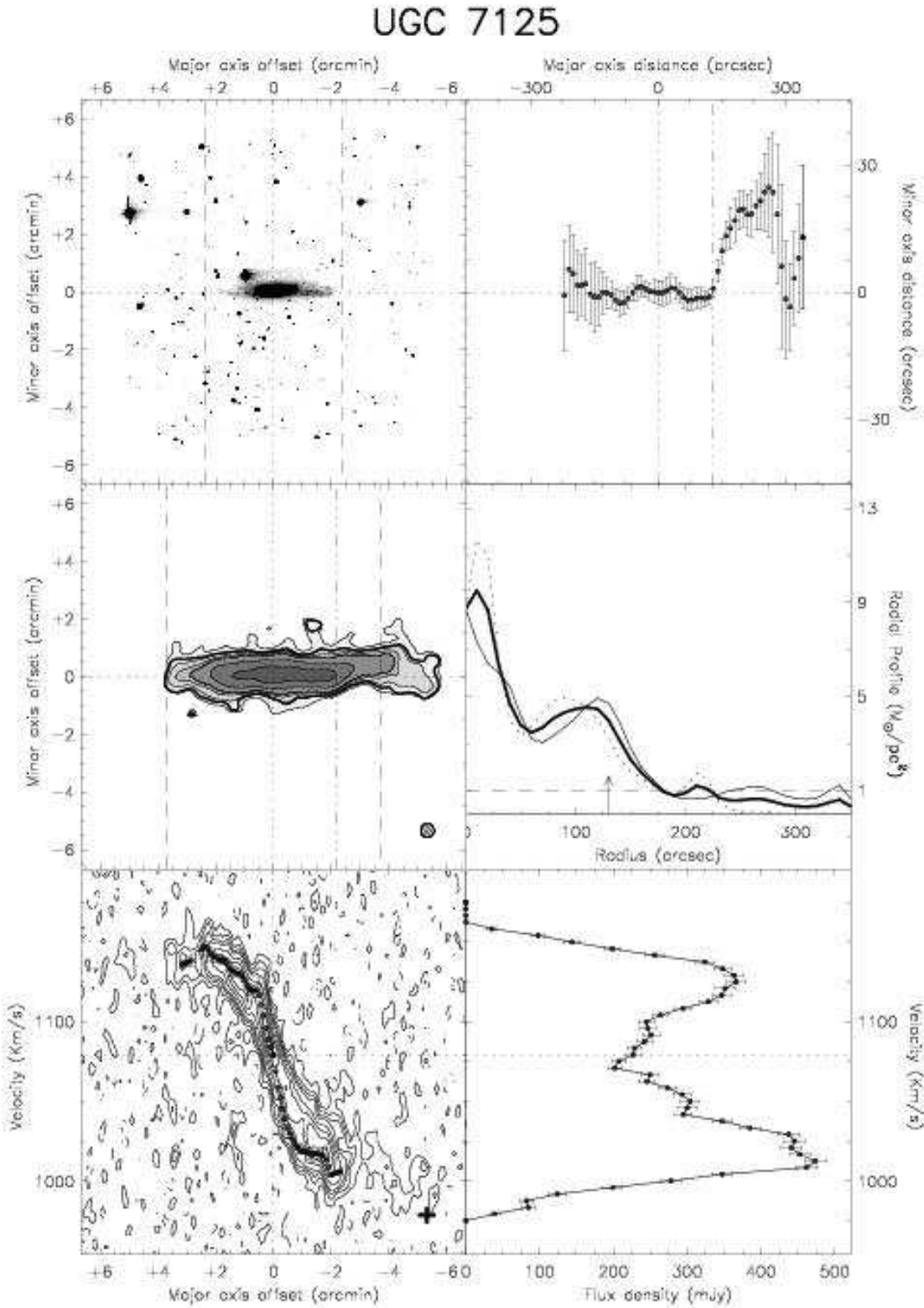
Fig. A.13. – continued. UGC 7125: The warp of this galaxy on the right part of the disk resembles that of the Milky Way: it rises and then turns back towards the plane, crossing it. For this galaxy the lowest contour in the total HI map is 1.7 \cdot 10^{20} HI atoms/cm 2 , and in the XV diagram 3\sigma = 11.6 K.
