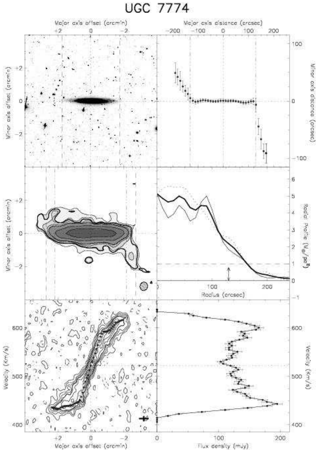
Fig. A.13. – continued. UGC 7774: This is the most remarkable galaxy in our sample. The right side of the disk is warped at a very high angle and the line of nodes (LON) is very close to the line of sight. However, the LON of the SE warp is not close to the line of sight, creating a very asymmetric warp. Standard tilted-ring models would be unable to fit the warp of this galaxy due to the difference in the LON for the receding and approaching sides. The closest known galaxy is at 300 kpc (projected separation), so tidal interaction is unlikely to be the cause of this extremely asymmetric warp. For this galaxy the lowest contour in the total HI map is 1.3 \cdot 10^{20} HI atoms/cm 2 , and in the XV diagram 3\sigma = 12.5 K.
