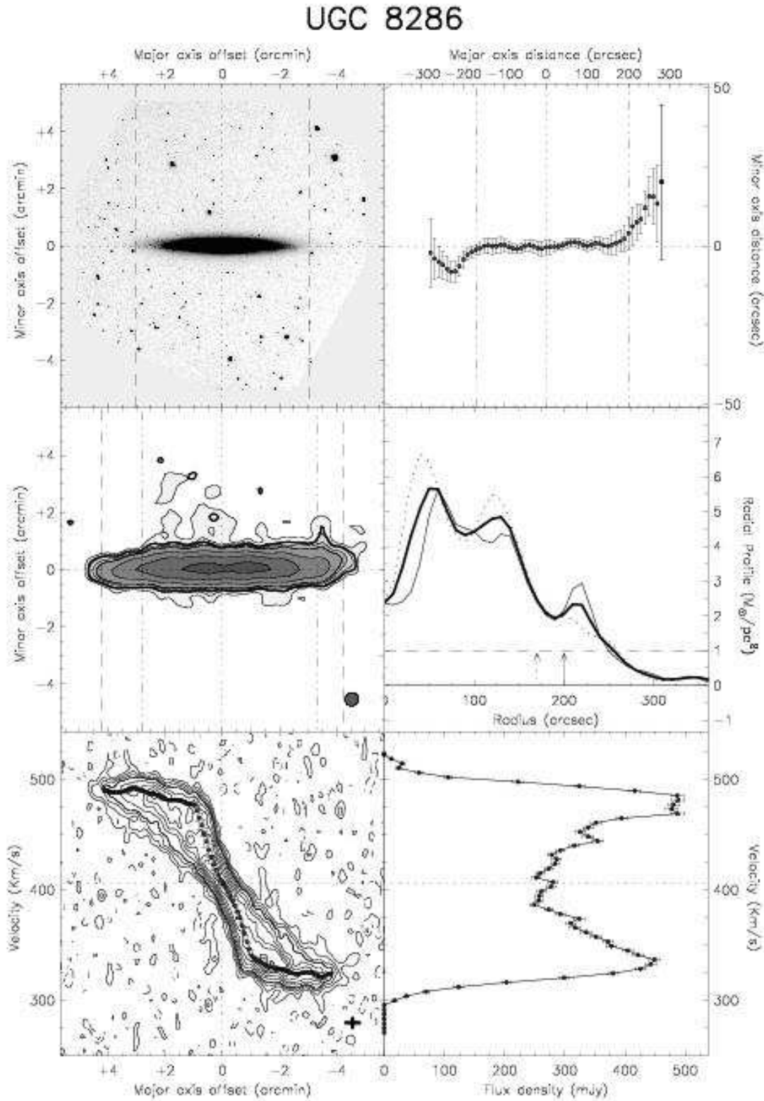
Fig. A.13. – continued. UGC 8286: This galaxy has a mild warp on both sides of the galaxy, starting around the edge of the optical disk. For this galaxy the lowest contour in the total HI map is 1.2 \cdot 10^{20} HI atoms/cm 2 , and in the XV diagram 3\sigma = 9.87 K.
