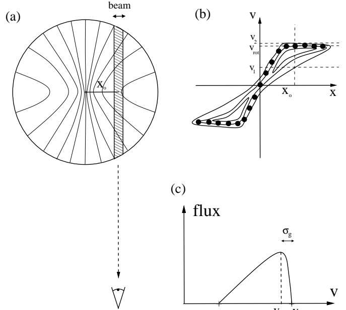
Fig. 2. Schematic representation of the HI detected at each position along the major axis in an edge-on galaxy. (a) At a certain distance x_o from the center of the galaxy, all the emission from gas in the dashed area is detected by the telescope. Isovelocity lines (with respect to the observer) have been drawn in the figure. The XV diagram along the major axis with the rotation curve (filled dots) is shown in (b), and a velocity profile at a certain major axis distance ( x_o ) in (c). The rotation velocity at x_o is indicated by v_{\text{rot}} , where \sigma_g is the broadening due to instrumental and random motion effects.
