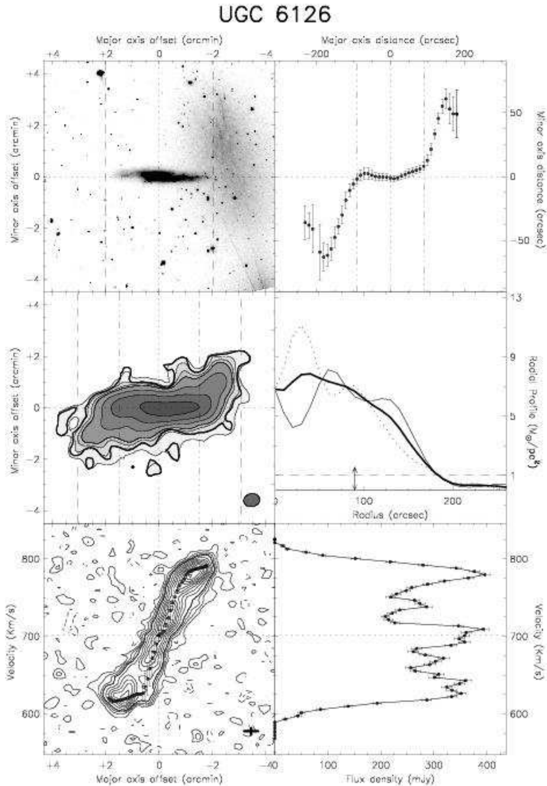
Fig. A.13. – continued. UGC 6126: This galaxy has one of the largest warps of the sample. It is surrounded by companion galaxies, three of which are detect in HI. Taylor et al. (1994) observed this galaxy with a higher resolution with the VLA and detected low level HI emission above the end of the disk on the right side. Careful inspection of our datacube smoothed to a 60'' beam and velocity resolution of 25 km/s resulted in a marginal detection of that HI cloud. The warp has more structure in density than usual at full resolution and it has a velocity slightly higher than the maximum of the rotation curve (which in general is not true for the warps in other galaxies). For this galaxy the lowest contour in the total HI map is 1.1 \cdot 10^{20} HI atoms/cm 2 , and in the XV diagram 3\sigma = 7.68 K.
