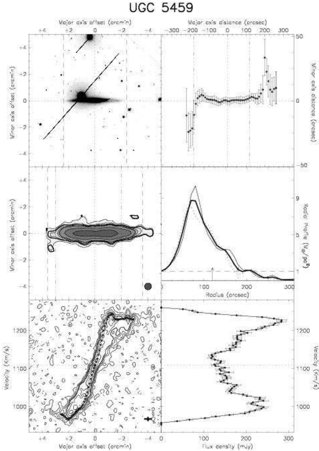
Fig. A.13. – continued. UGC 5459: This is a prototype of a kinematically lopsided galaxy. The rotation curve rises fast and remains approximately flat on the receding side, whereas it keeps smoothly rising on the approaching side. For this galaxy the lowest contour in the total HI map is 2.3 \cdot 10^{20} HI atoms/cm 2 , and in the XV diagram 3\sigma = 15.7 K.
