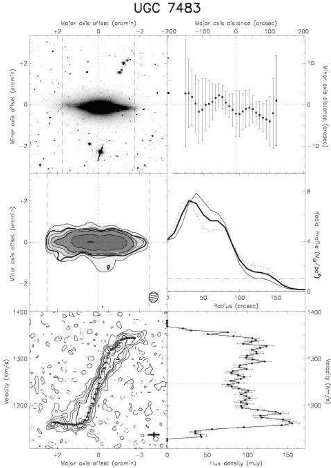
Fig. A.13. – continued. UGC 7483: We found this galaxy to be classified as SBc. The optical picture shows a very prominent bulge and a small disk (even in the HI) so it is likely that it is an earlier type. As with other galaxies with bulges, we find that the optical disk is misaligned with the HI disk by few degrees. For this galaxy the lowest contour in the total HI map is 2 \cdot 10^{20} HI atoms/cm 2 , and in the XV diagram 3\sigma = 11.4 K.
