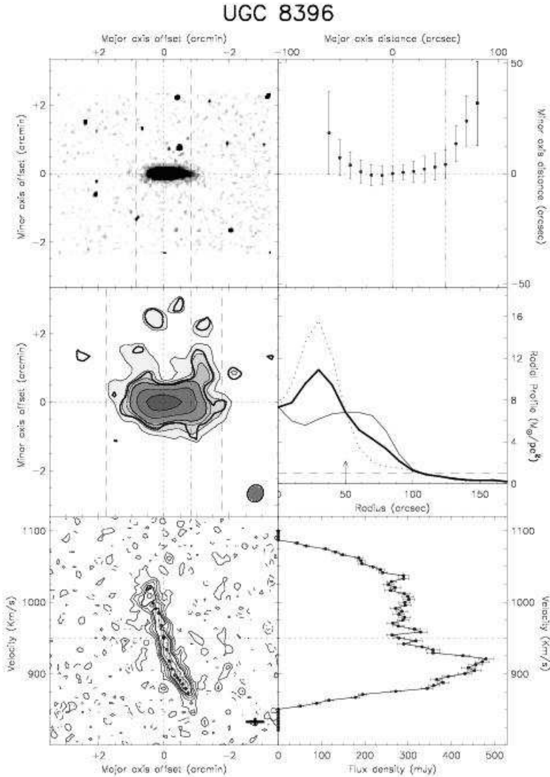
Fig. A.13. – continued. UGC 8396: This galaxy is very close to NGC 5112 (13 arcmin) and seems to be perturbed by it. The U shaped warp seems to ‘point’ towards NGC 5112. We also detected some “loose” HI gas between UGC 8396 and NGC 5112. For this galaxy the lowest contour in the total HI map is 1.5 \cdot 10^{20} HI atoms/cm 2 , and in the XV diagram 3\sigma = 14.5 K.
