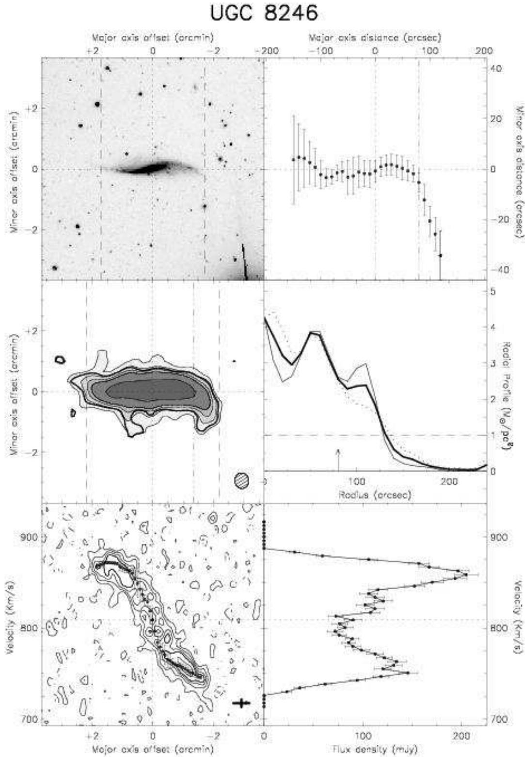
Fig. A.13. – continued. UGC 8246: This galaxy is very close (6 arcmin) to NGP9 F269-1340356, detected at similar velocities in our 21 cm data. The central parts of the galaxy show evidence of large non-circular motions, and it is possible that the warped appearance is due to either spiral arms or tidal features. For this galaxy the lowest contour in the total HI map is 1.3 \cdot 10^{20} HI atoms/cm 2 , and in the XV diagram 3\sigma = 10.6 K.
